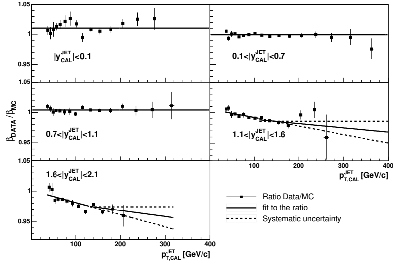
FIG. 4: Ratio \beta_{\text{data}}/\beta_{\text{mc}} as a function of p_{T,\text{cal}}^{\text{jet}} in different |y_{\text{cal}}^{\text{jet}}| regions. The solid lines show the nominal parameterizations based on fits to the ratios. In the region |y_{\text{cal}}^{\text{jet}}| > 1.1 , the dashed lines indicate different parameterizations used to describe the ratios at high p_{T,\text{cal}}^{\text{jet}} , and are considered in the study of systematic uncertainties.
