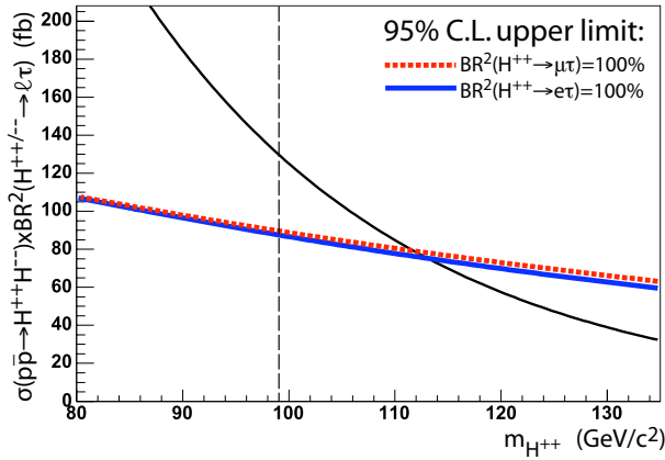
FIG. 1: Theoretical production cross sections for the pair production of left-handed H^{\pm\pm} , and 95% C.L. limit curves for \sigma(p\bar{p} \rightarrow H^{++}H^{--} \rightarrow \ell\tau) \times B^2(\ell^+\tau^+\ell^-\tau^-) , for \ell = e (solid), \mu (dashed). The vertical dashed line corresponds to limits from experiments at LEP2 for exclusive H_L^{\pm\pm} decays to any one dilepton channel [9].
