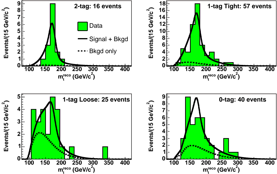
FIG. 2: The m_t^{\text{reco}} distribution of the template method is shown for each subsample overlaid with the expected distribution using M_{\text{top}} , \Delta_{\text{JES}} and signal and background normalizations from the combined fit. The events with \chi^2 > 9 have been excluded from each subsample.
