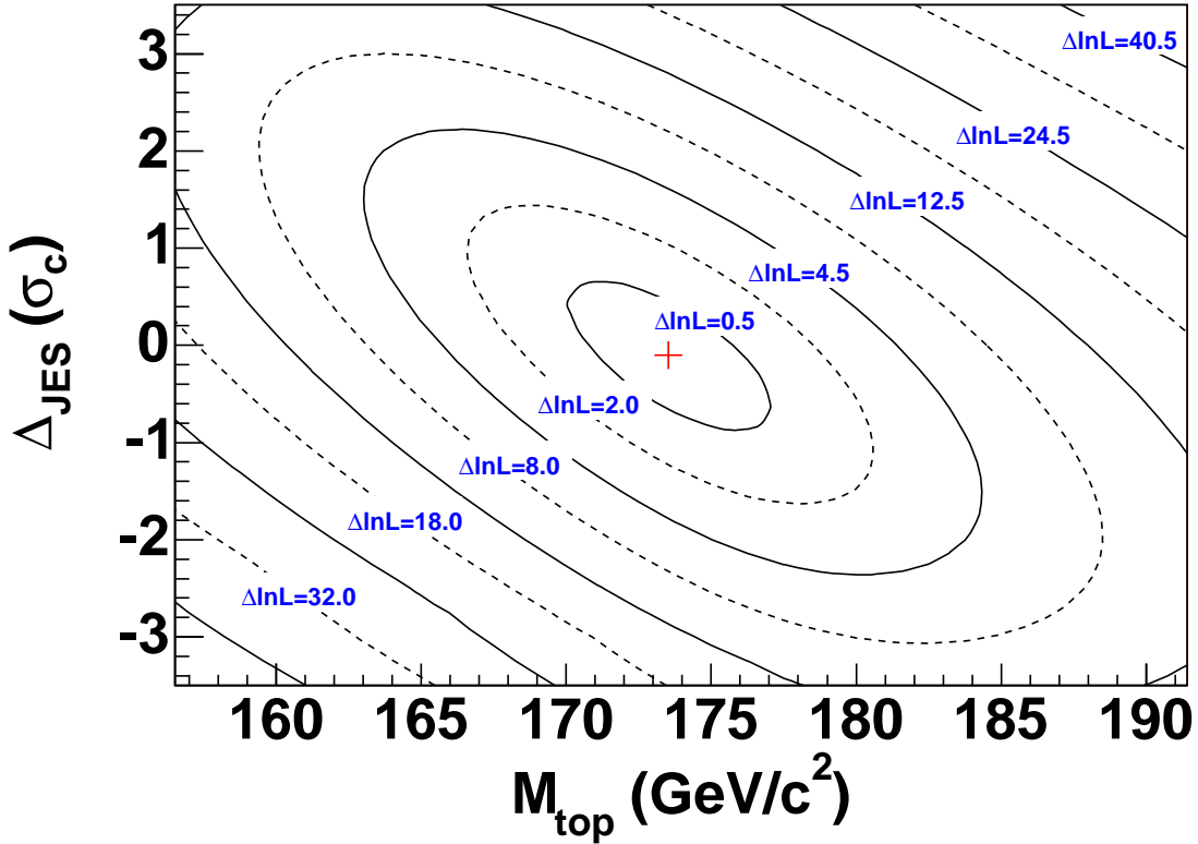
FIG. 3: Contours of the template method likelihood are shown in the M_{\text{top}}-\Delta_{\text{JES}} plane for the combined fit to all four subsamples. The crosshair shows the best fit point. Contours are given at intervals of \Delta \ln L , the change in log-likelihood from its maximum.
