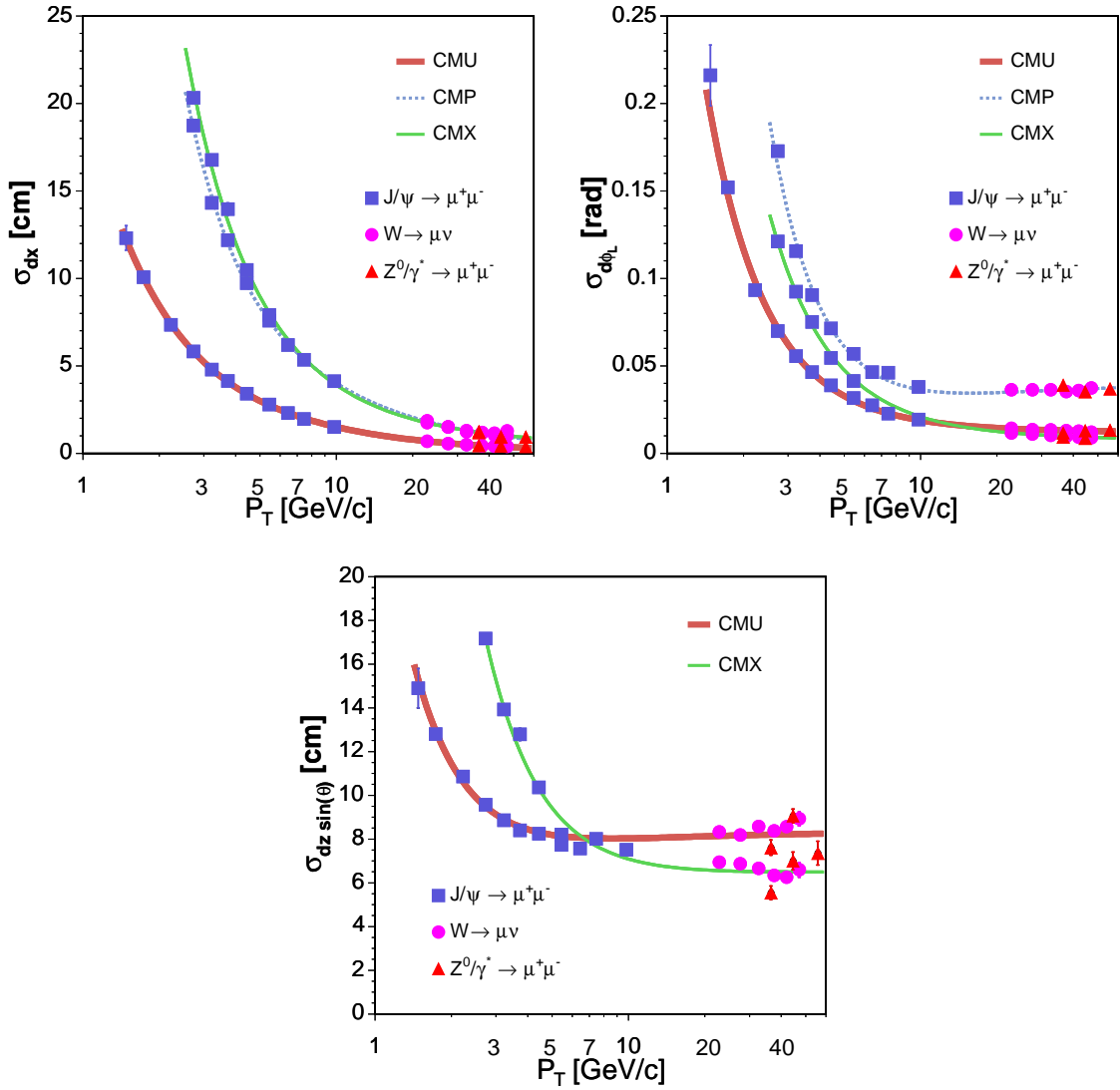
FIG. 4: Width of the matching variable distributions ( dx , dz \sin \theta , d\phi_L ) vs. P_T for each of the muon chambers. The data points, from J/\psi , W and Z decays, are fit to the parameterizations described in the text.
