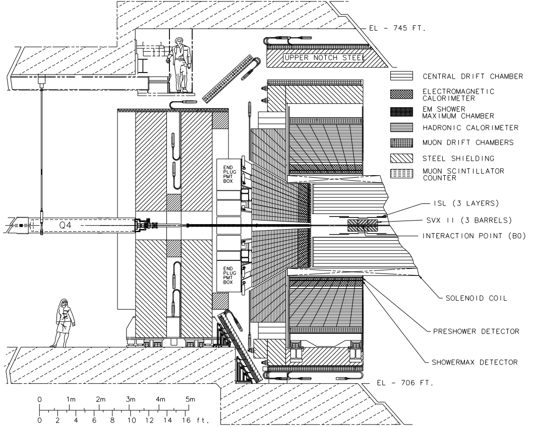
FIG. 1: Elevation view of the CDF II detector.
