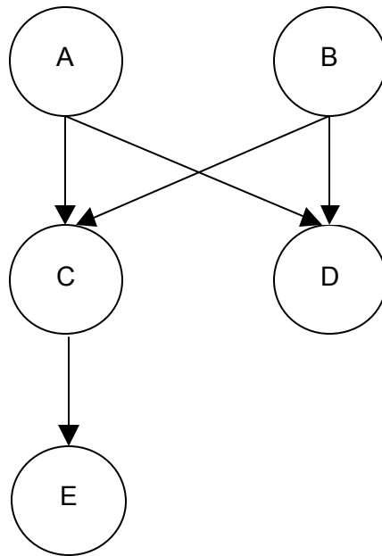
Figure 4.10. Bayesian networks: indirect mediation of effects of explanatory variables
