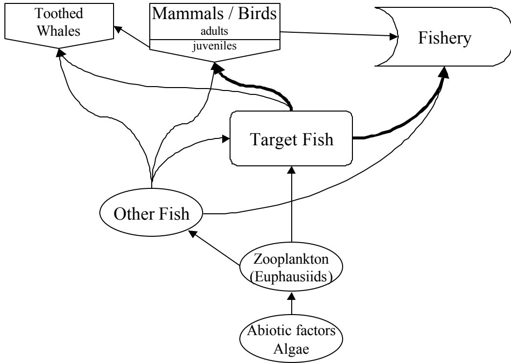
Figure 4.8. A food web that includes environmental factors.
