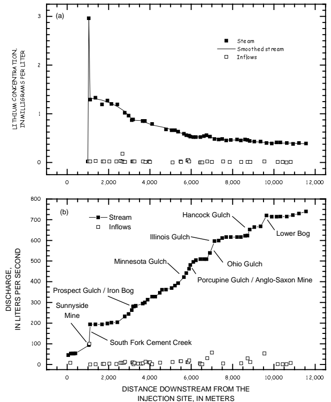
Figure 2. (a) Variation of lithium concentration with distance downstream from the injection site. The relatively low concentration of lithium in inflow samples indicates that lithium was an effective tracer. (b) Variation of calculated discharge with distance. Some major tributaries are indicated.
