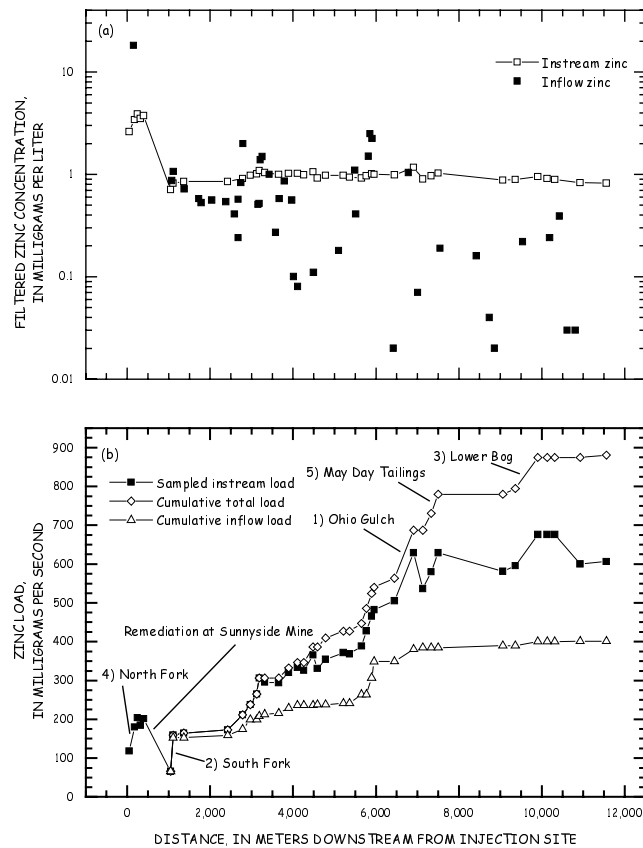
Figure 4. Variation of (a) zinc concentration and (b) zinc load with distance in samples from Cement Creek, Colorado. The five largest inflows are indicated by name and a number for its rank. The sampled instream load represents the calculated load at each stream site. The cumulative total load represents a summation of the entire load entering the stream. The cumulative inflow load represents the part of the total load that can be attributed to sampled inflows.
