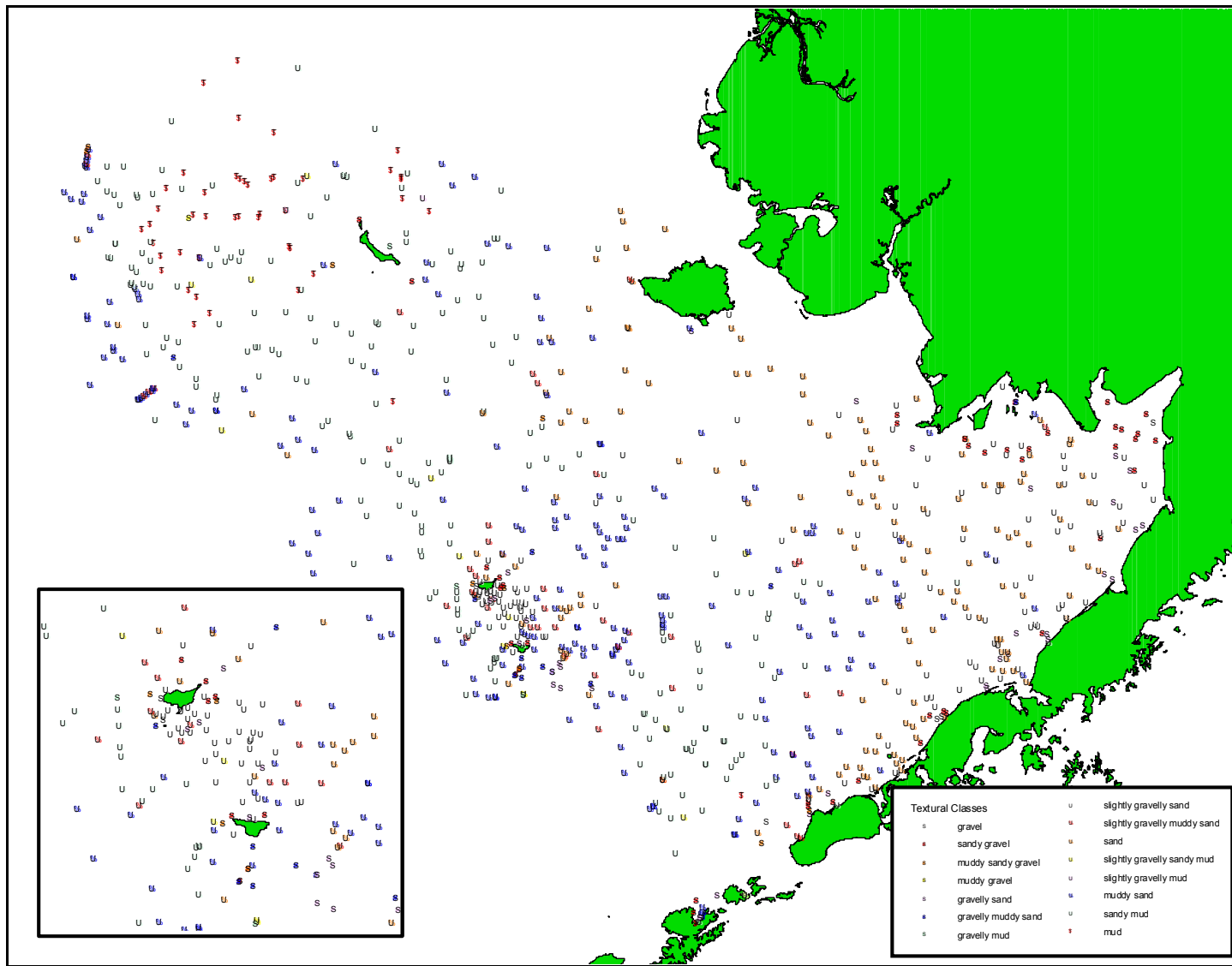
Figure 3.1.3 High resolution textural class of grain size analysis samples. Source: Smith and McConnaughey 1999).
