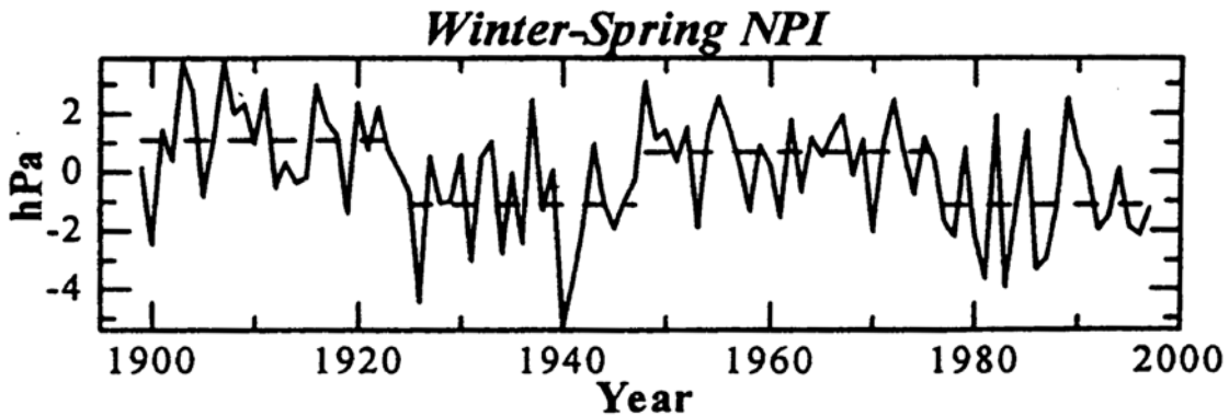
Figure 3.1.5 The North Pacific Index (NPI) , area-averaged Sea Level Pressure anomaly in the region 160E-140W, 30-65N over winter-spring (Dec.-May) seasons (solid curve), and the respective averages for 1899-1924, 1925-1947, 1948-1976, and 1977-1997 (dashed lines), (Minobe, 1999).
