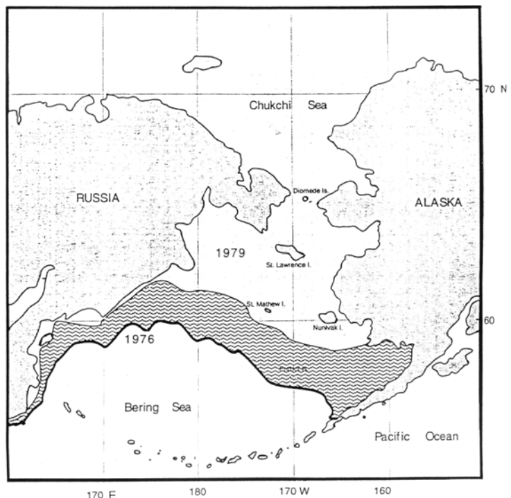
Figure 3.1.4 Maximum (1976) and minimum (1979) extent of sea ice in the Bering Sea.
