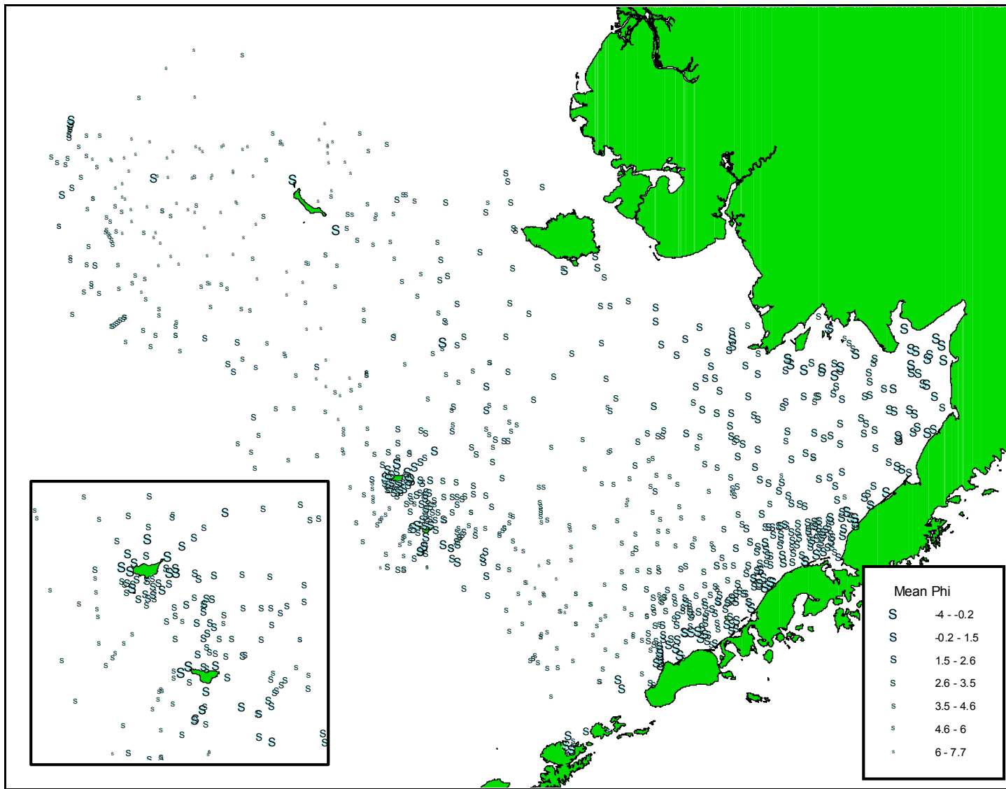
Figure 3.1.2 Mean diameter of sediment grains at 994 sample locations. Inset is larger-scale view of St. George and St. Paul Pribilof Islands and vicinity. Source: Smith and McConaughy 1999).
