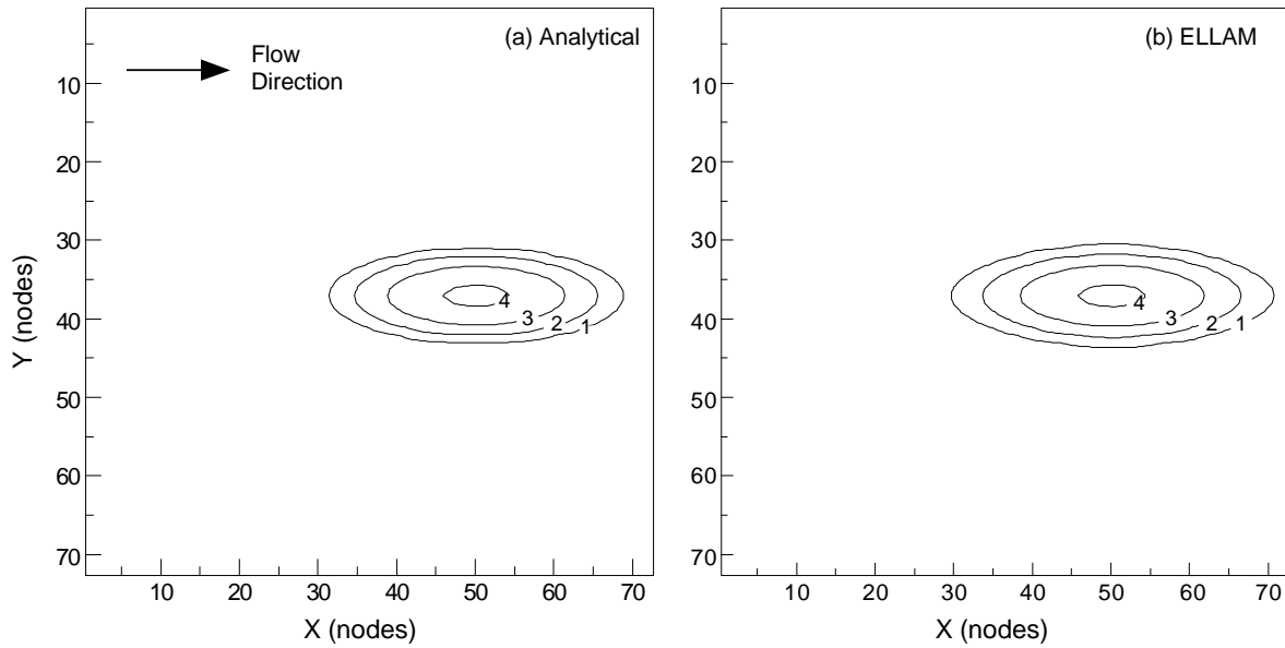
Figure 17. Concentration contours for (a) analytical and (b) ELLAM numerical solutions for transport of a dispersed-point initial condition in uniform flow in the x -direction at t = 130 days. The y - and z -components of flow are zero, but dispersion occurs in all three directions. Contour values are the log of the concentrations.
