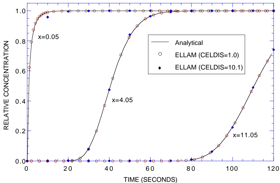
Figure 10. Numerical and analytical solutions at three different locations for solute transport in a one-dimensional, steady flow field. Parameter values for the base case are listed in table 3.
