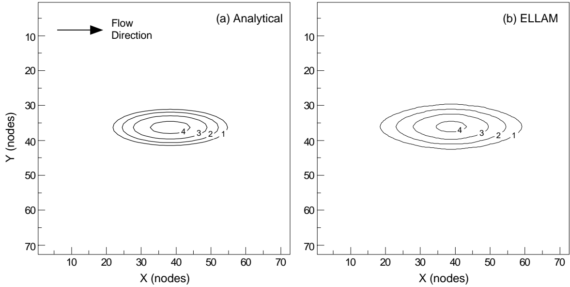
Figure 16. Concentration contours for (a) analytical and (b) numerical solutions for transport of a point initial condition in uniform flow in the x -direction at t = 90 days. The z -component of flow is zero, but there is dispersion in all three directions. Contour values are the log of the concentrations.
