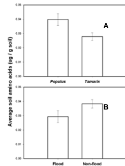
Figure 4. Average soil amino acids in Populus vs. Tamarix sites (2-way ANOVA: N = 8, df = 1, F = 5.24, p = 0.033) (A) and in flood vs. non-flood sites (N = 8, ns) (B) ± 1 SE. No interaction effect exists between vegetation and flood type.
