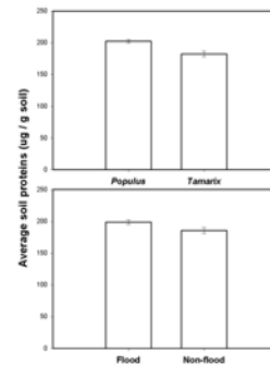
Figure 5. Average soil proteins in Populus vs. Tamarix sites (2-way ANOVA: N = 8, df = 1, F = 9.04, p = 0.007) (A) and in flood vs. non-flood sites (N = 8, df = 1, F = 3.78, p = 0.066) (B) ± 1 SE. No interaction effect exists between vegetation and flood type.
