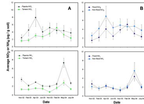
Figure 6. Average NO 3 (RMANOVA, N = 8, ns) and NH 4 (N = 4, F = 64.27, p = 0.001) ± 1 SE in Populus vs. Tamarix sites (Panel A) and in flood (N = 8, ns) vs. non-flood sites (N = 8, ns) (Panel B).
