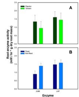
Figure 7. Average root enzyme activity of gluco-7-amin-4-methylcoumarin (GAM) and leucine amino peptidase (LAP) in Populus vs. Tamarix roots (2-way ANOVA, N = 8, ns) (A) and in roots from flood vs. non-flood sites (N = 8, ns) (B) ± 1 SE.
