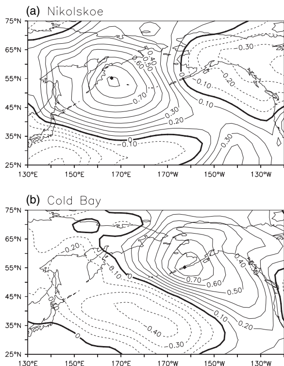
Figure 7. One-point correlation maps for winter (DJF) SATs at (a) Nikolskoe and (b) Cold Bay. Data: 1950–2003. Correlation coefficients exceeding 10.251 (10.341) are significant at the 0.05 (0.01) level.
