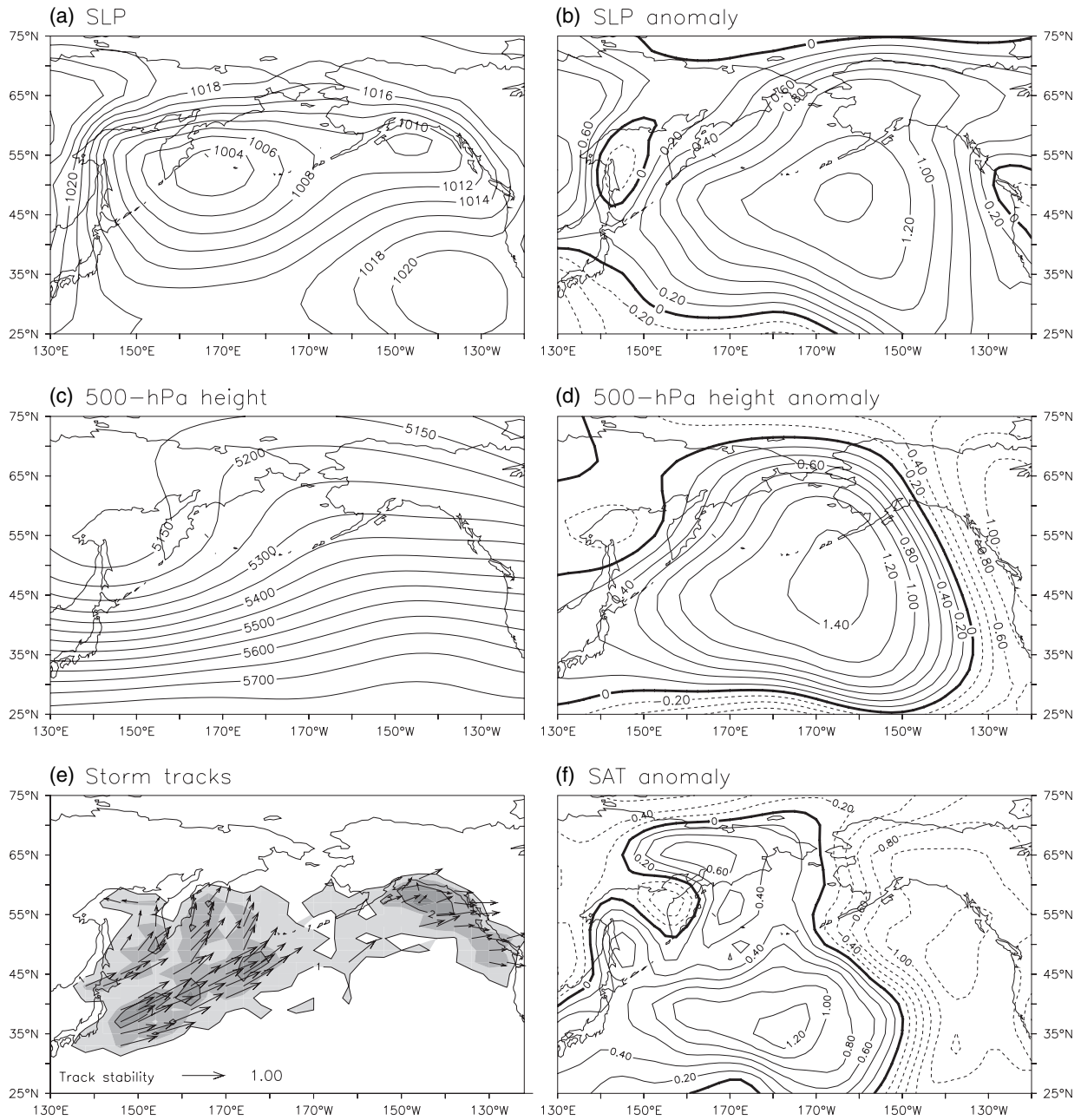
Figure 6. Same as Fig. 4, but for 10 yr with the highest NP index.
