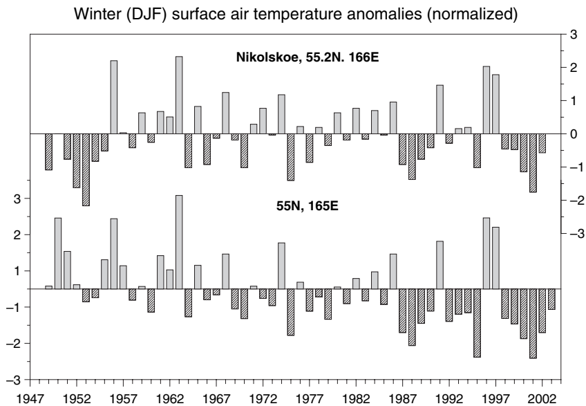
Figure 9. Normalized (by SD) mean winter (DJF) SAT anomalies at Nikolskoe (1949–2002) and the grid point 55°N, 165°E from the Reanalysis (1949–2003).
