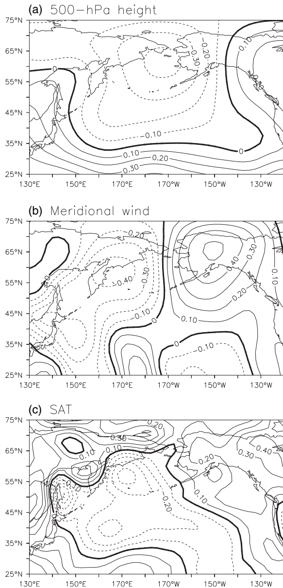
Figure 10. Correlation coefficients with time (yr) for mean winter (DJF) (a) 500 hPa height, (b) meridional wind component at the 500 hPa level, and (c) SAT. The correlation coefficients exceeding |0.25| are significant at P < 0.05 .
