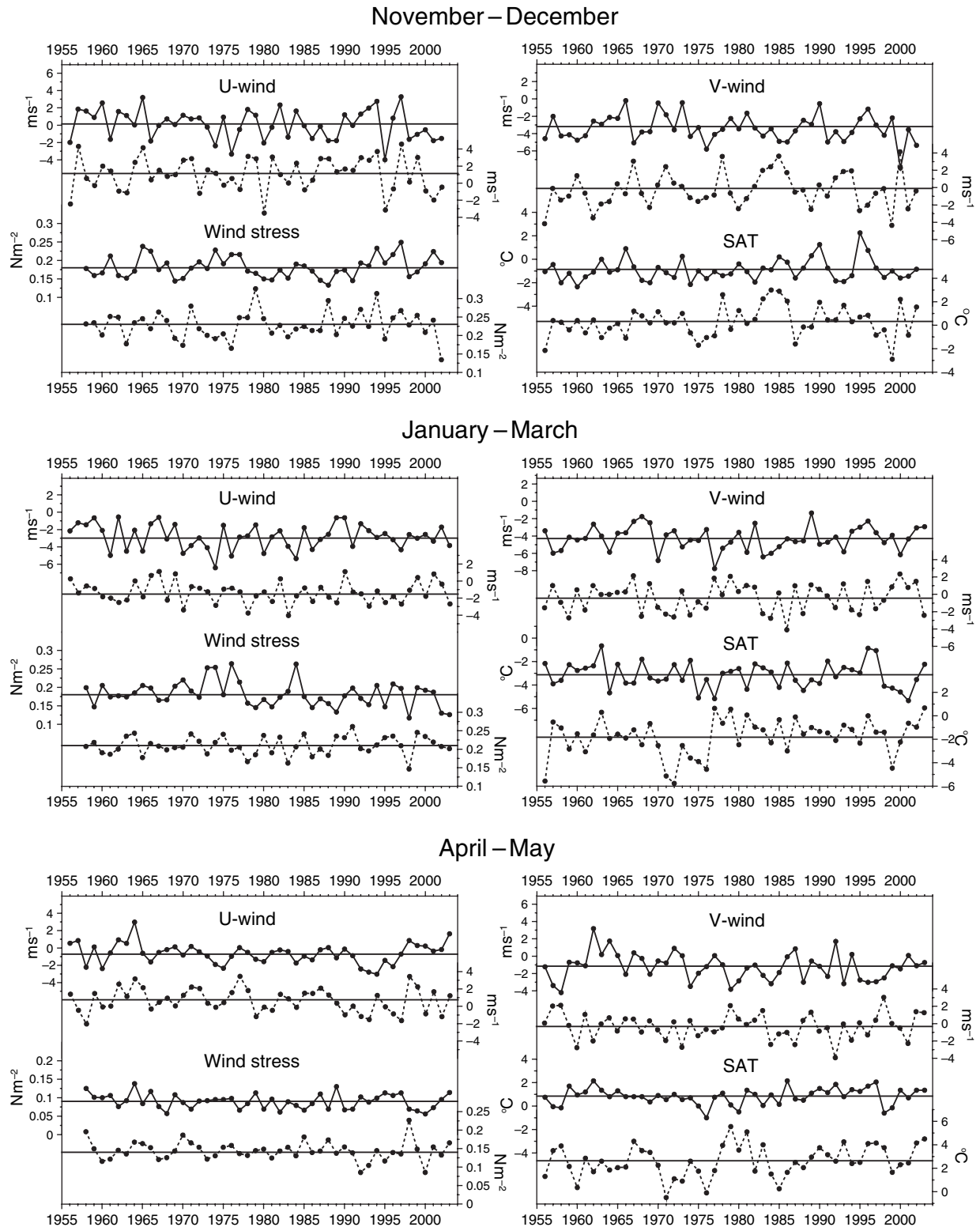
Figure 8. Time series of zonal ( u ) and meridional ( v ) wind components, wind stress, and SAT at Nikolskoe (solid line) and Cold Bay (broken line) averaged for November–December (top panel), January–March (middle panel), and April–May (bottom panel). The horizontal lines for each time series indicate the mean values for the base period, 1961–2000.
