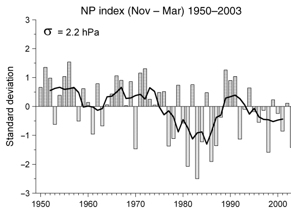
Figure 4. The North Pacific Index, 1950–2003 (adapted from Trenberth and Hurrell, 1994). The solid line is a 5-year running average.
