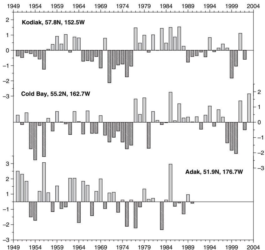
Figure 14. Normalized mean winter (DJF) SAT anomalies at (from top to bottom) Kodiak, Cold Bay, and Adak, Alaska.
