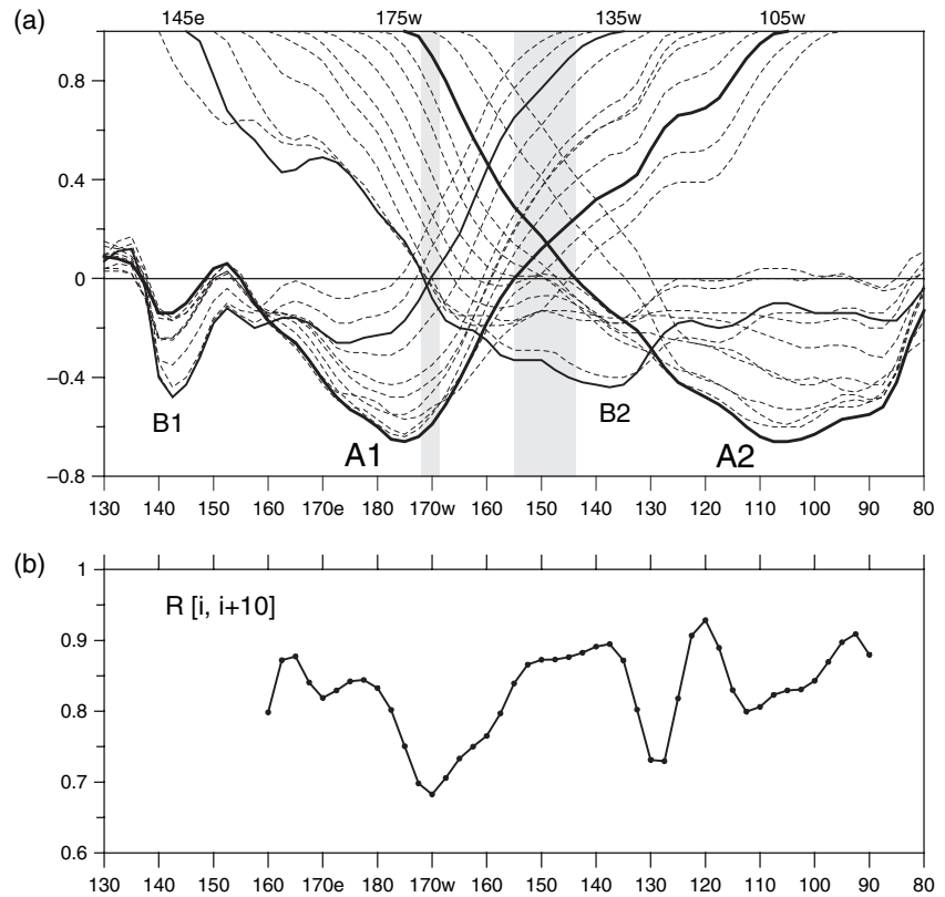
Figure 15. (a) Spatial correlation functions of winter (DJF) SAT along the 52.5°N parallel for different base points. Solid lines are the correlation functions for the dipoles A1–A2 (thick line) and B1–B2 (thin line). The grey vertical bars indicate the transition zones between the opposite centres of the dipoles. (b) Correlation coefficients along the same parallel between SATs at the pairs of grid points 5° to the east and 5° to the west of the given point.
