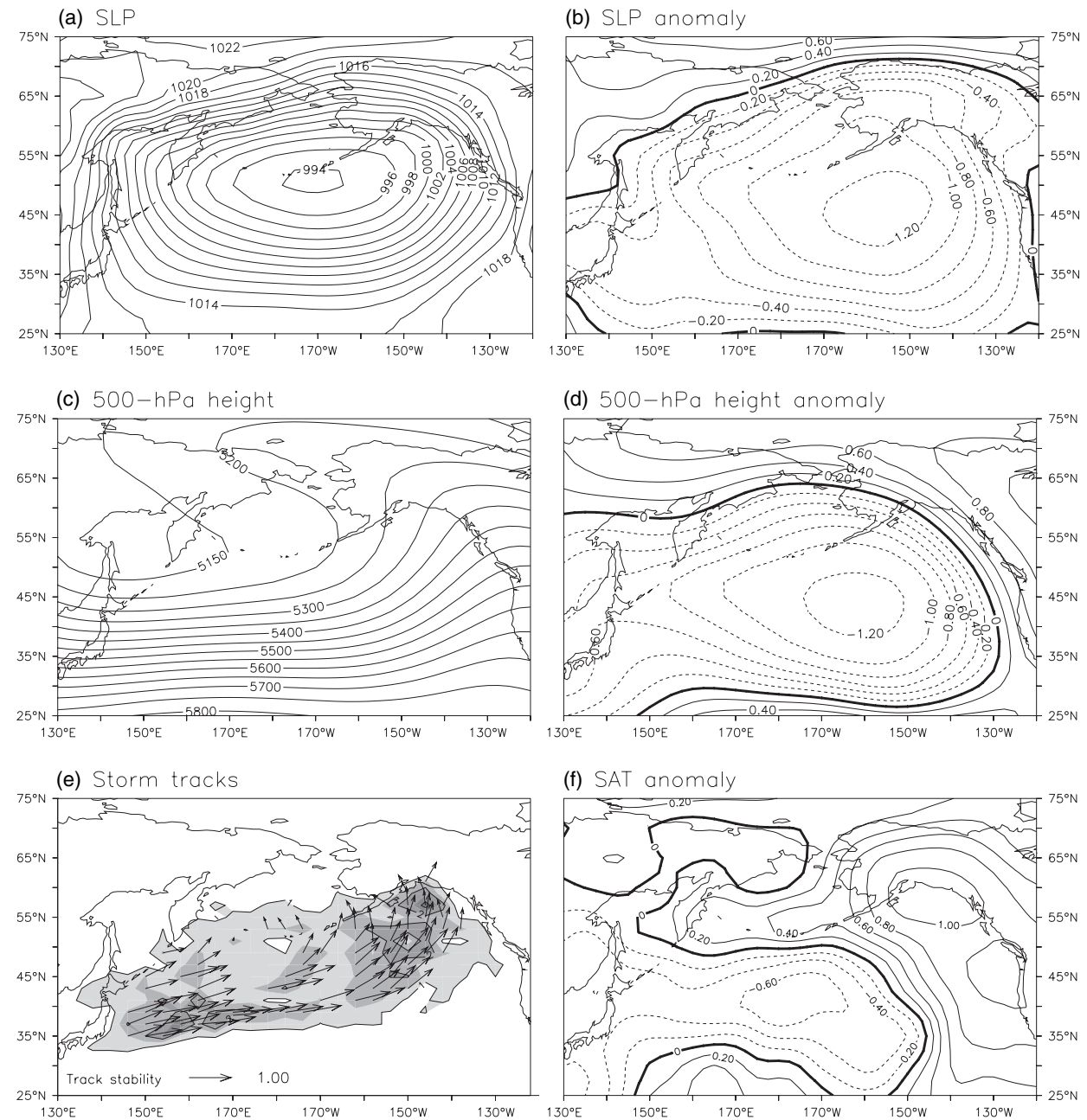
Figure 5. Composite maps of (a) SLP (hPa), (b) SLP anomaly (SD), (c) 500-hPa height (m), (d) 500-hPa height anomaly (SD), (e) storm tracks, and (f) SAT anomaly (SD) for 10 yr with the lowest NP index during 1950–2002. The base period for anomalies is 1951–2000. Assuming that the variance has not changed over time, the anomalies in figure b, d, and f are locally significant at the 0.05 probability level (one-tail t -test) if their magnitude exceeds 0.57.
