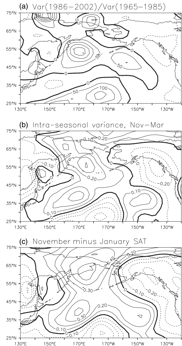
Figure 11. (a) Difference in mean winter (November–March) SAT variance between 1986–2002 and 1965–1985, in percent, (b) Correlation coefficients with time (yr) for intra-seasonal (November–March) SAT variance, and (c) same as (b) but for the SAT difference between November and January.
