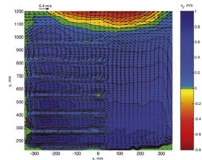
Sectional view of the SPIV-measured flow velocity field in the doorway of an ISO 9705 test room (inflow indicated by blue, outflow by red).
