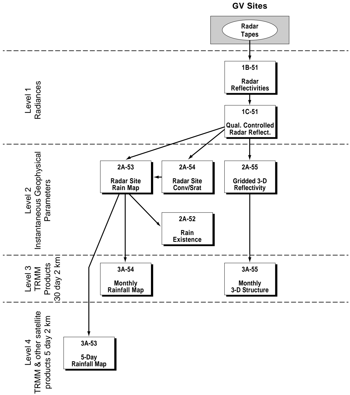
Figure 2. Flow Diagram Showing Interaction of TRMM Ground-Based Radar Validation Products.
