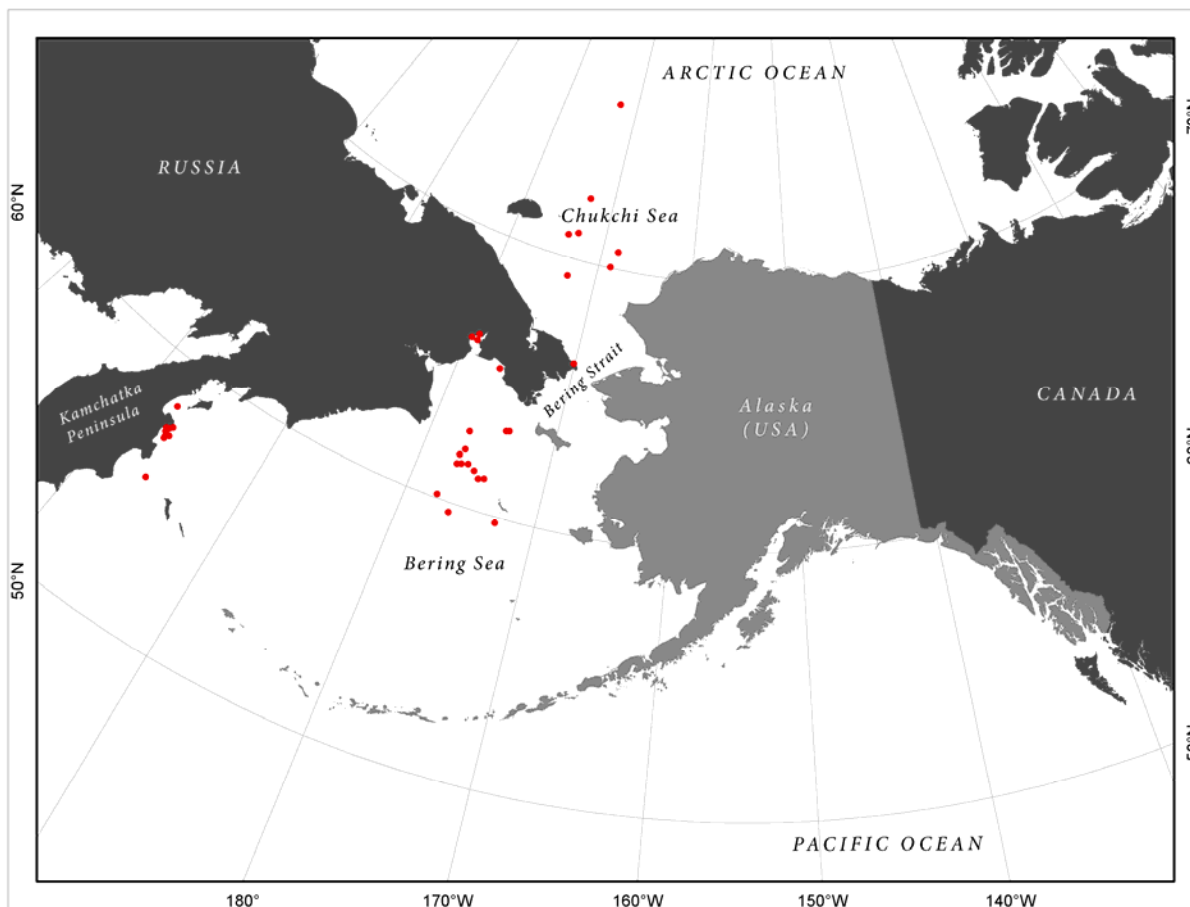
Figure 5. -- Positions at the highest recorded latitudes (red points) for each of 36 satellite-tracked ribbon seals between 1 June and 1 September from 2005 to 2008. These positions provide an indication of the proportion of the tracked sample that spent the ice-free pelagic season either north or south of the Bering Strait (no tracked seals moved north of the Bering Strait after 1 September). None of 10 seals tagged in the western Bering Sea near the Kamchatka Penninsula moved north of the Bering Strait. Of 26 seals tagged in the central Bering Sea, 8 seals moved into the Bering Strait or Chukchi Sea, but 3 of those returned south into the Bering Sea well ahead of the next southward advance of winter ice.
