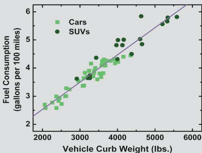
Relationship of fuel consumption rate to vehicle weight for a representative set of vehicles used in the United States. Data from: Effectiveness and Impact of Corporate Average Fuel Economy (CAFE) Standards , National Academy Press (Washington, DC: 2002)
