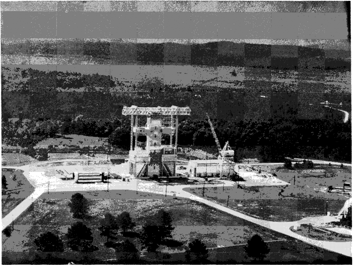
Saturn IB test stand, Marshall Space Flight Center
