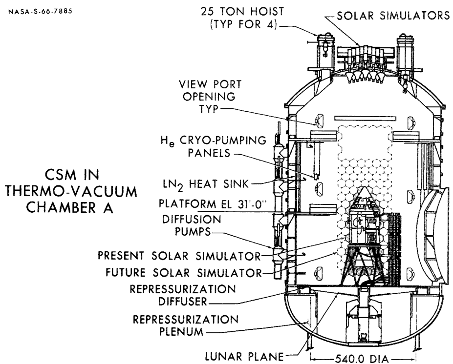
Space environment simulation laboratory, chamber A diagram
