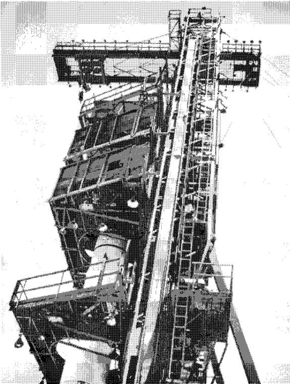
Mercury/Redstone spacecraft and service structure, Air Force Space Museum (complex 26B), Cape Canaveral Air Force Station, 1981
