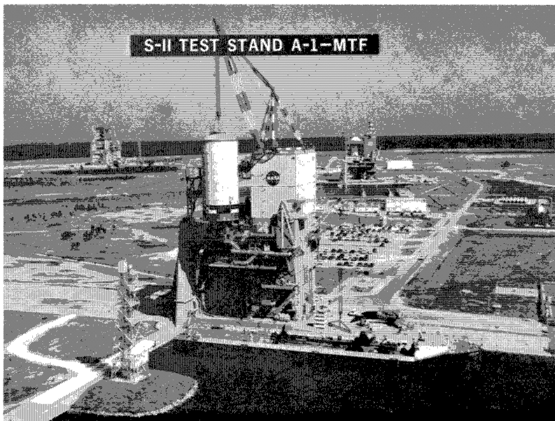
Test stand, National Space Technology Laboratories
