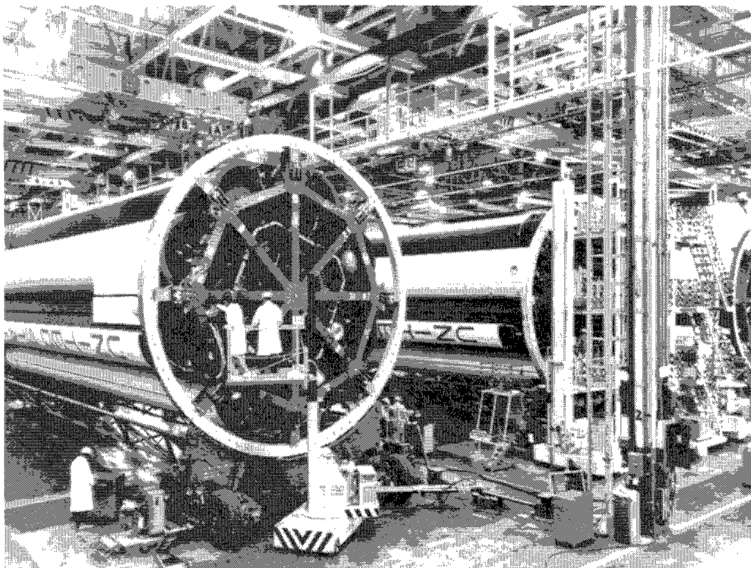
Stage assembly, Michoud Assembly Facility
