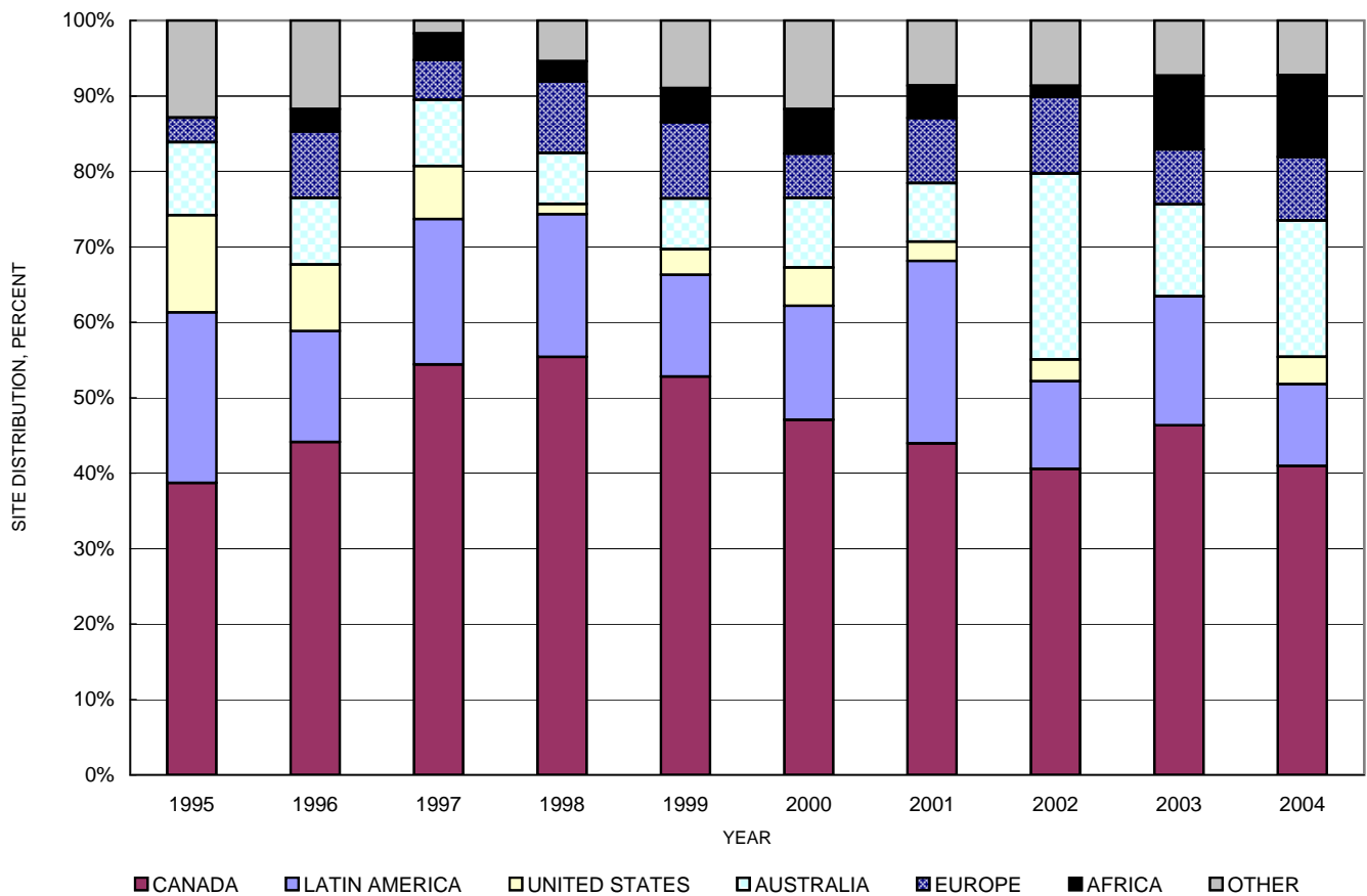
Figure 7. Lead and zinc exploration activity by region for 1995 through 2004. Exploration activity is expressed in terms of the percentage of total exploration activity, as determined by the number of active exploration sites considered for each year in this study. Europe includes Eastern Europe and Western Europe; Latin America includes Central America, Mexico, and South America; and other includes Asia, the Commonwealth of Independent States, India, the Middle East, Southeast Asia and the Pacific islands (excluding Australia).
