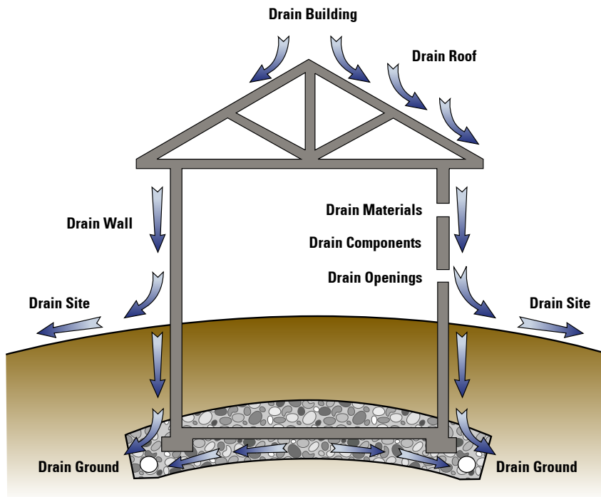
FIGURE 3: Drainage
