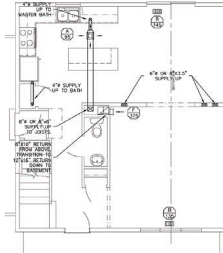
A duct layout was designed and shown on plans to help ensure accurate installation.
