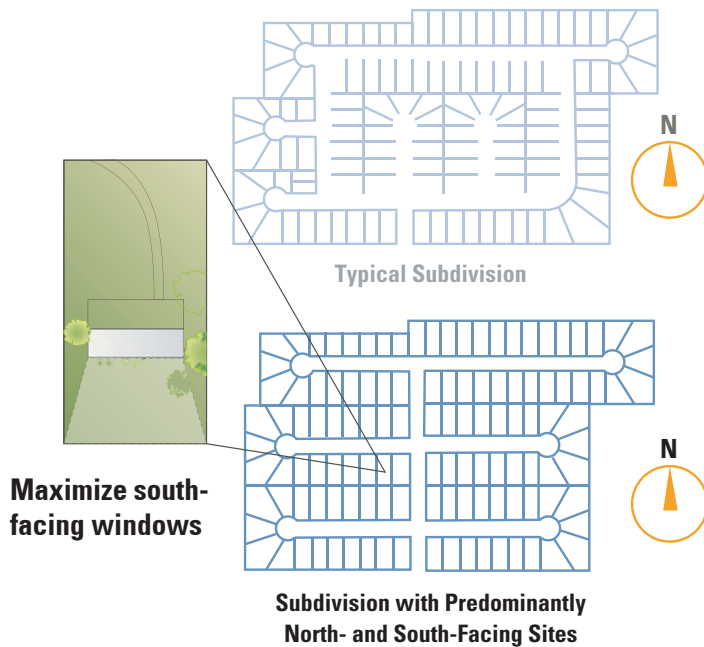
FIGURE 1: Plan subdivision lot lines and roads for predominantly north and south orientation – minimize north-facing windows and place houses within lots to take advantage of solar access.
