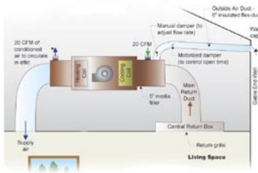
FIGURE 15: Outside Vents
