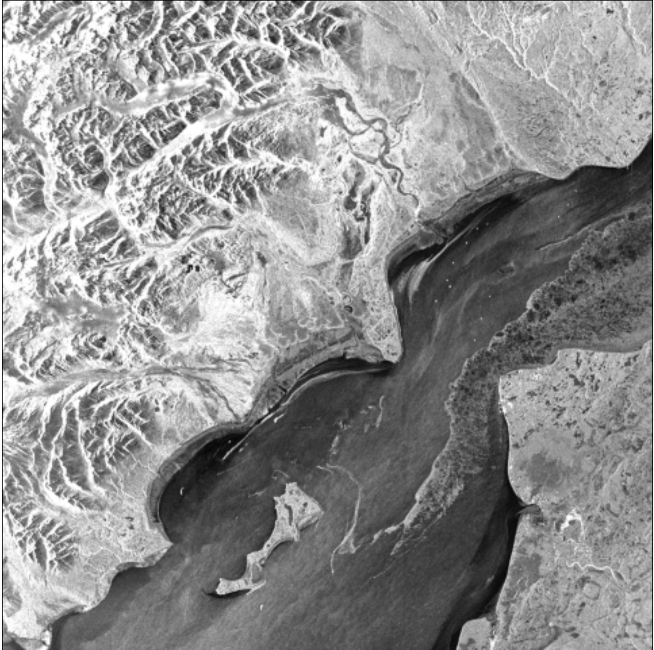
Figure 14. Radarsat-1 SAR imagery showing the Forelands area of Cook Inlet at near low tide on December 30, 1998. The region appearing stippled along the East Foreland is 6 to 10 tenths young and first-year thin sea ice. Tidal flats are visible along the northern shores with streaks of 5 to 7 tenths new ice forming just offshore in Trading Bay and Redoubt Bay. The bright white specks in three distinct rows that appear in the water north of the Forelands are oil production platforms. [Image copyright by Canadian Space Agency (1998); used by permission.]
