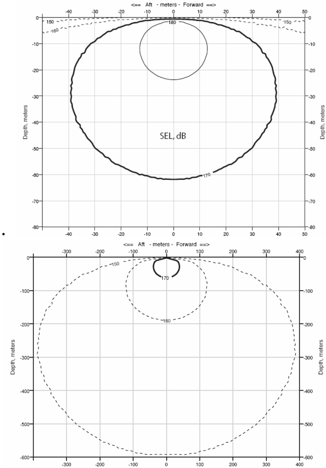
FIGURE 7. Modeled received sound levels (SELs) from a single 40 in 3 airgun, at a 7-m tow depth, planned for use during power-down operations during the proposed seismic surveys in the ETP during 2007.
