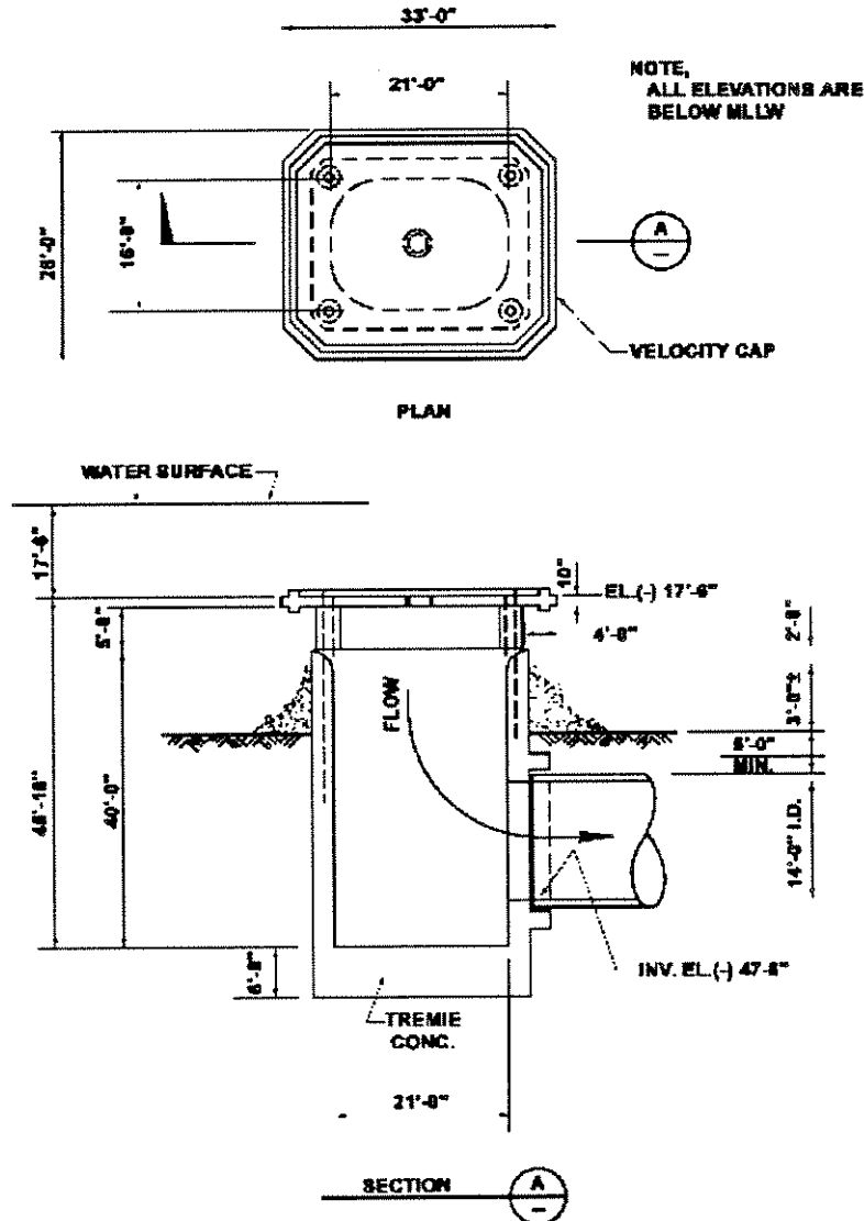
Figure 2. Layout of velocity cap (top) and profile at the offshore intake structure (bottom). AES Huntington Beach L.L.C. generating station.
