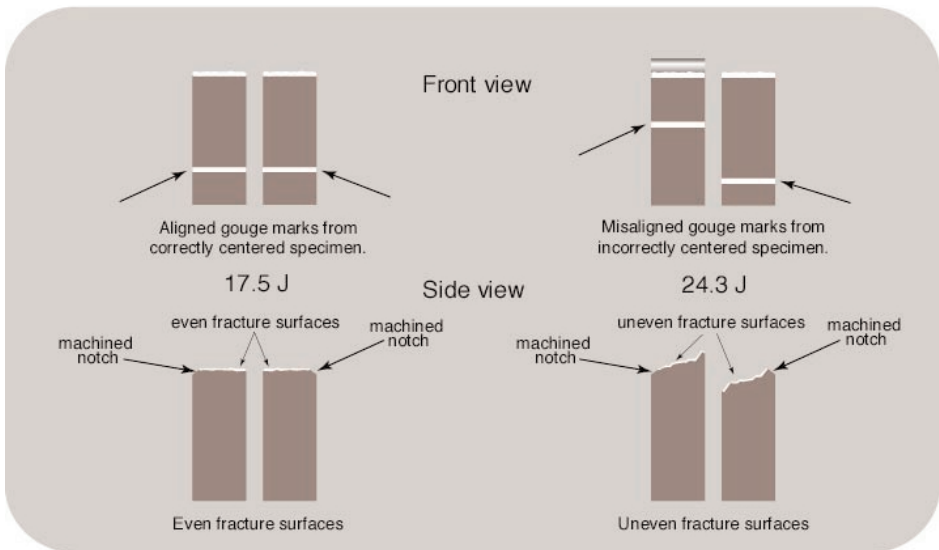
Figure 2. Off-Center Specimen.
