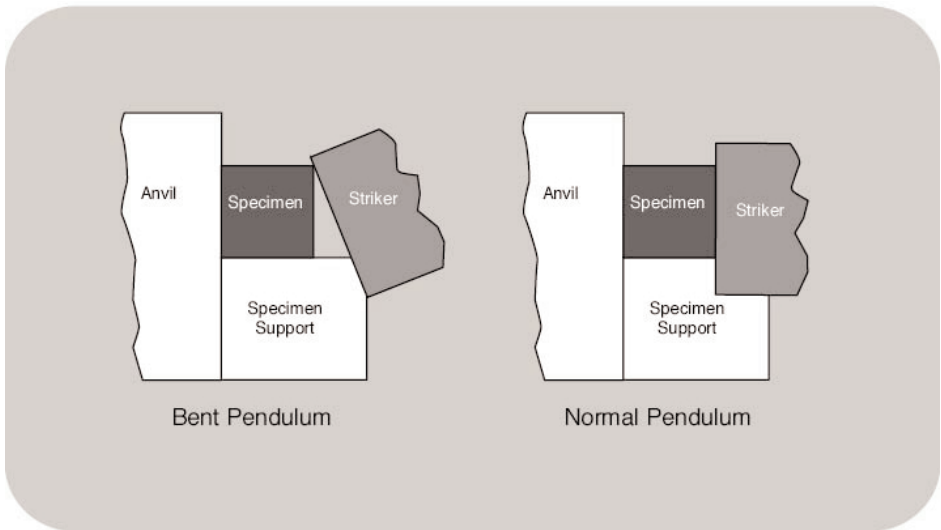
Figure 8. Bent Pendulum.
