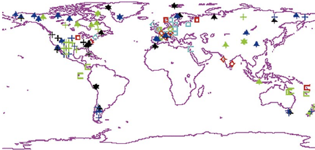
Figure 1. Distribution of annual resolution proxy indicators used in this study. Denroclimatic reconstructions are indicated by tree symbols, ice core/ice melt proxies by star symbols, and coral records by C symbols. Long historical records and instrumental "gridpoint" series are shown by squares (temperature), or diamonds (precipitation). Groups of plus (+) symbols indicate principal components of dense tree-ring subnetworks, with the number of such symbols indicating the number of retained principal components. Sites are shown dating back to at least 1820 (red), 1800 (blue-green), 1750 (green), 1600 (blue), and 1400 (black). Certain sites (e.g., the Quelccaya ice core) consist of multiple proxy indicators (e.g., multiple cores, and both oxygen isotope and accumulation measurements). [Reprinted with permission from Mann et al. (Mann et al. 1998).]
