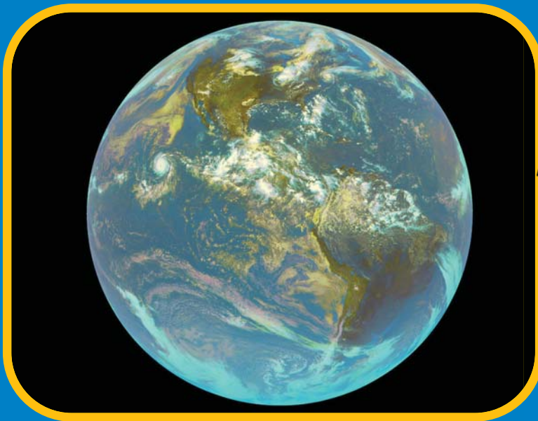
The GOES weather satellites see the whole Earth at once. This picture shows a tropical storm brewing in the Atlantic Ocean near New England and a hurricane in the Pacific Ocean. How do hurricanes form? Find out at spaceplace.nasa.gov/en/kids/goes/hurricanes .
