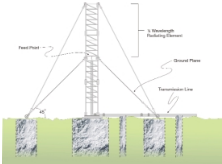
Figure 3.5. Diagram of WWV Antenna
