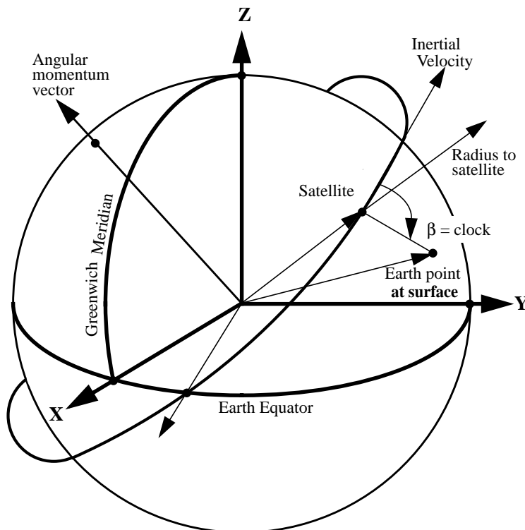
Figure 4-2. Clock Angle
