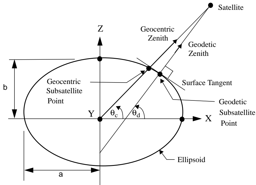
Figure 15-3. Subsattellite Point
