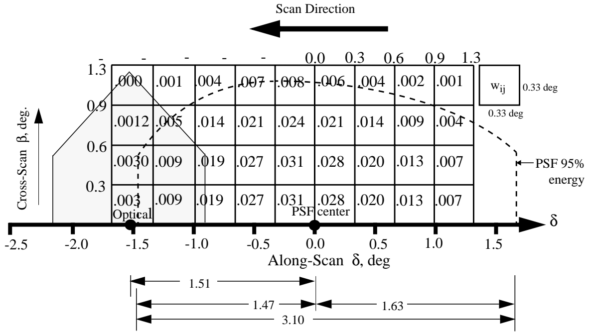
Figure 8-3. CERES Field-of-View Angular Grid
