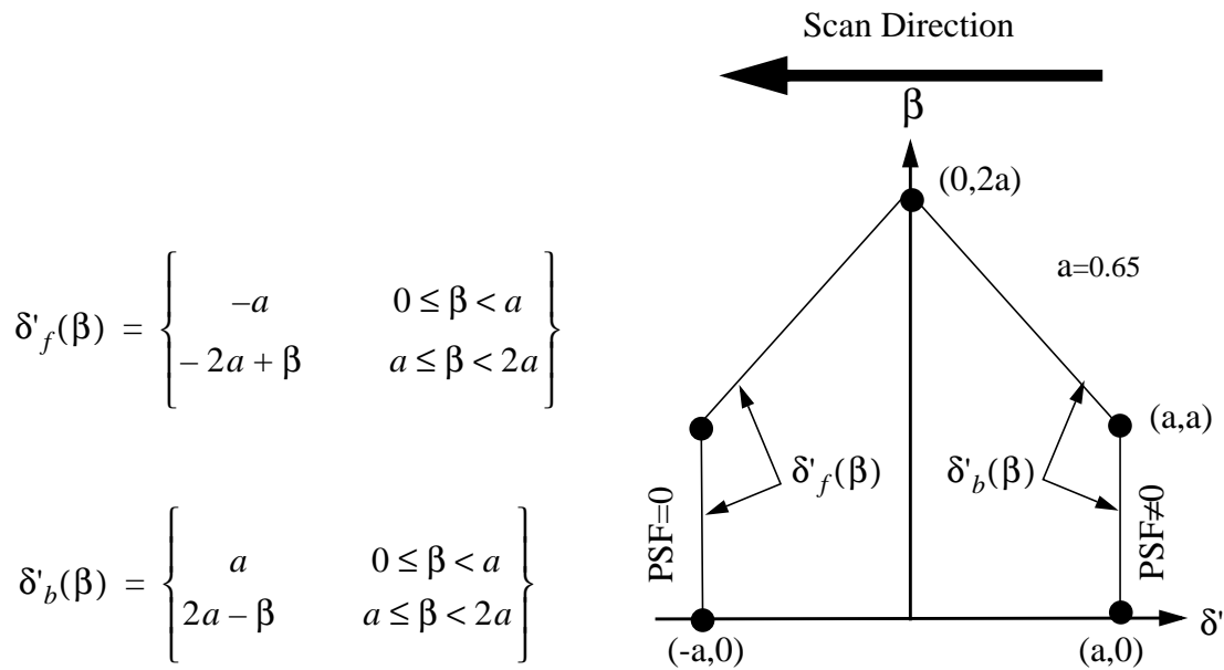
Figure 8-2. Optical FOV
