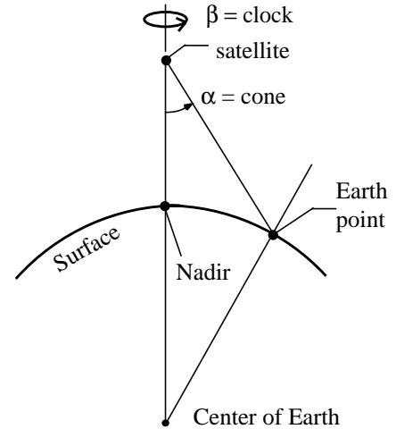
Figure 4-3. Cone and Clock Angles
