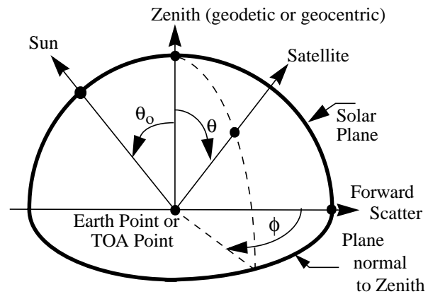
Figure 4-1. Viewing Angles at Surface or TOA
