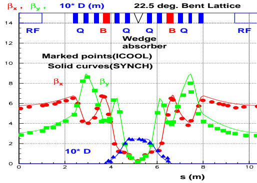
FIG. 41: (Color)The \beta_x , \beta_y , and D (dispersion) in a 22.5^\circ bending cell. SYNCH calculations(solid curves) and beam parameters from an ICOOL simulation(marked points) are compared.
