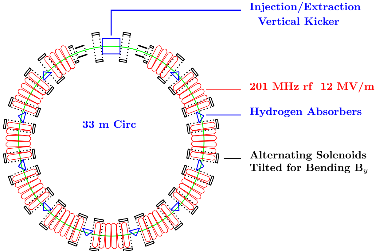
FIG. 37: (Color) Layout of an RFOFO cooling ring.
