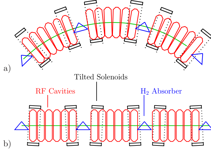
FIG. 38: (Color) Three cells of the RFOFO lattice; a) plan, b) side.
