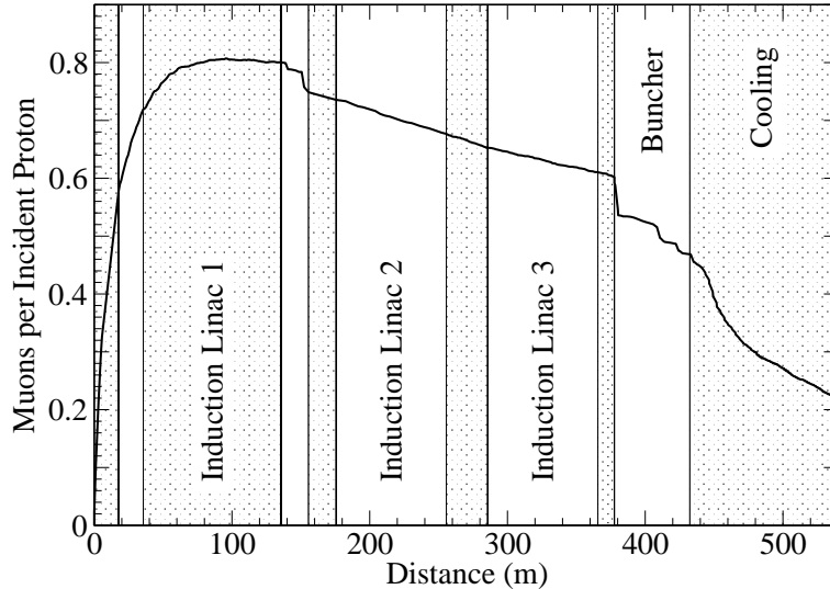
FIG. 25: Muons per incident proton in the Study II neutrino factory front end.
