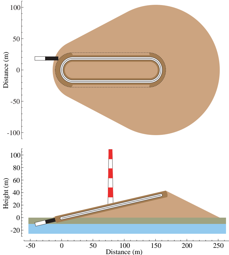
FIG. 26: (Color) Top view and cross section through 20 GeV ring and berm. The existing 110 m tower, drawn to scale, gives a sense of the height of the ring on the BNL landscape.
