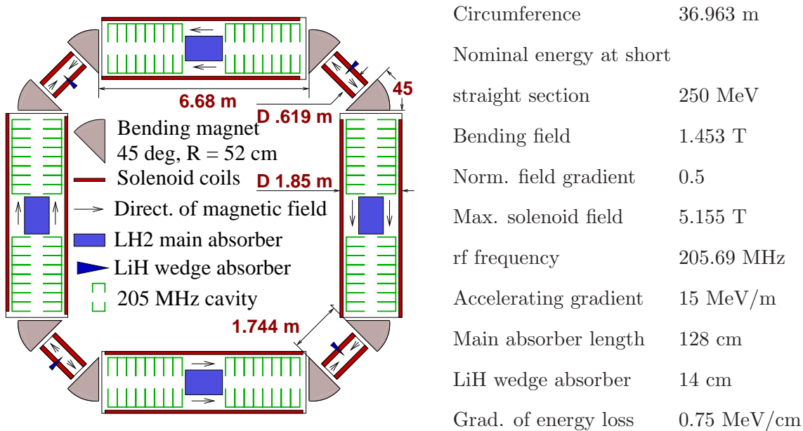
FIG. 34: (Color) Layout and parameters of the solenoid based ring cooler
