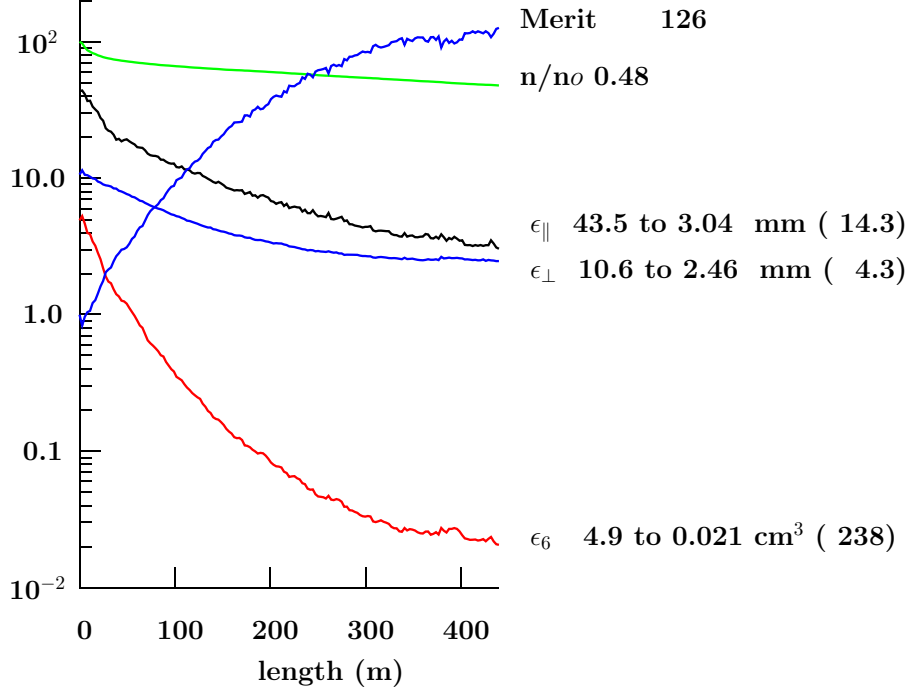
FIG. 39: (Color)Transmission, normalized transverse emittance, normalized longitudinal emittance, normalized 6-dimensional emittance, and the merit factor, as a function of distance.
