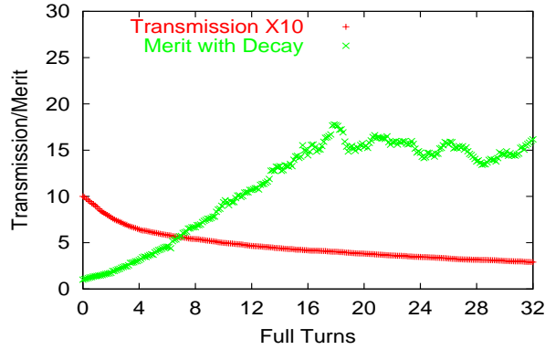
FIG. 44: (Color) The transmission and the figure of merit factor as a function of the arc length in 32 full turns.
