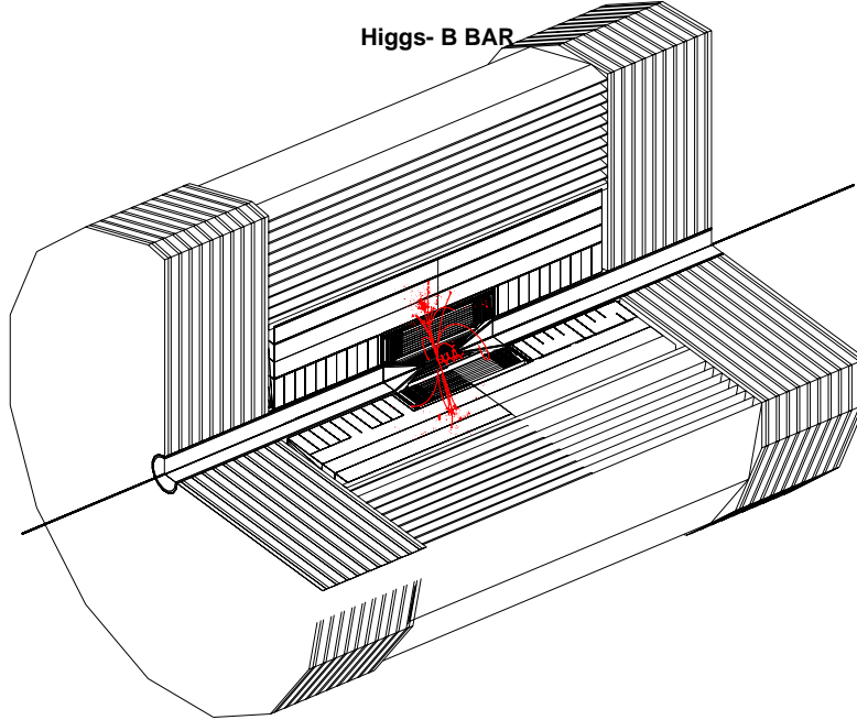
FIG. 45: (Color)Cut view of a strawman detector in Geant for the Higgs factory with a Higgs → b\bar{b} event superimposed. No backgrounds shown. The tungsten cones on either side of the interaction region mask out a 20 deg area.
