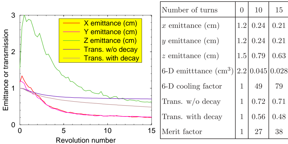
FIG. 35: (Color)Evolution of the beam emittance/transmission at the ring cooler.
