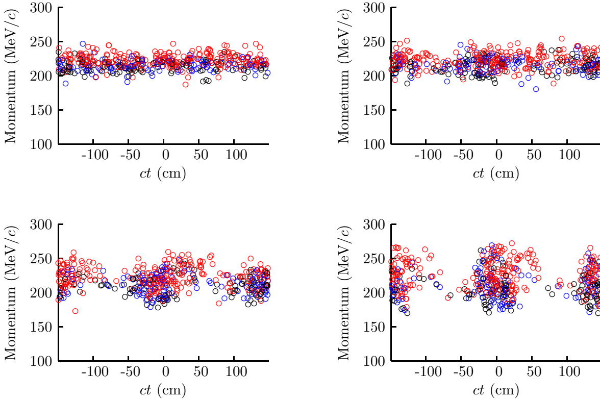
FIG. 17: (Color)Evolution of beam in buncher. Plots are at the beginning of the buncher (top left), and at the ends of the three bunching stages (top right, bottom left, and bottom right, in that order).
