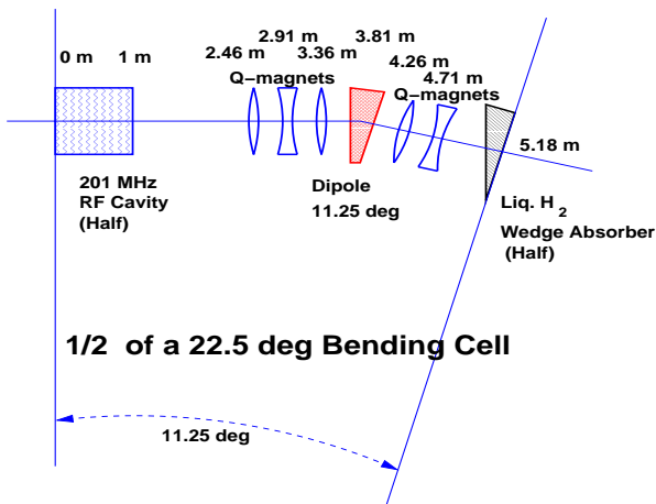
FIG. 40: (Color) Schematic diagram of half of a 22.5^\circ bending cell. A wedge absorber is located in the middle of the cell.
