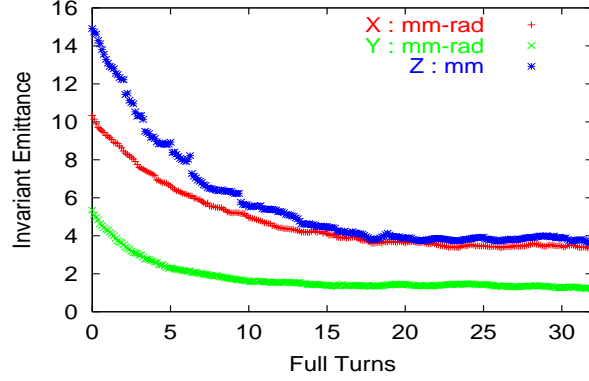
FIG. 43: (Color) The evolution of x, y, z normalized emittances in 32 full turns.
