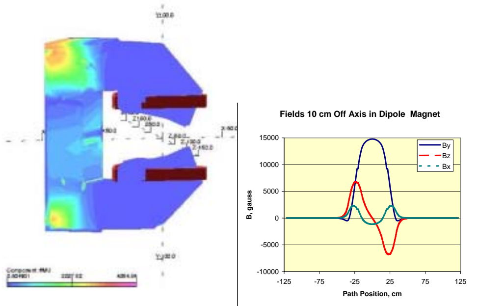
FIG. 36: (Color)Figure shows a computer model of a 52cm radius dipole with index n = -\frac{1}{2} and the calculated field components radially 10cm off axis.
