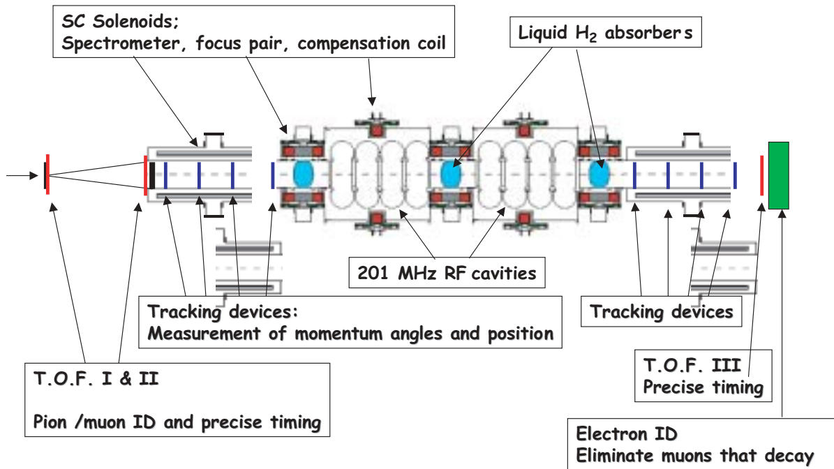
FIG. 47: (Color) Schematic layout of MICE apparatus.
