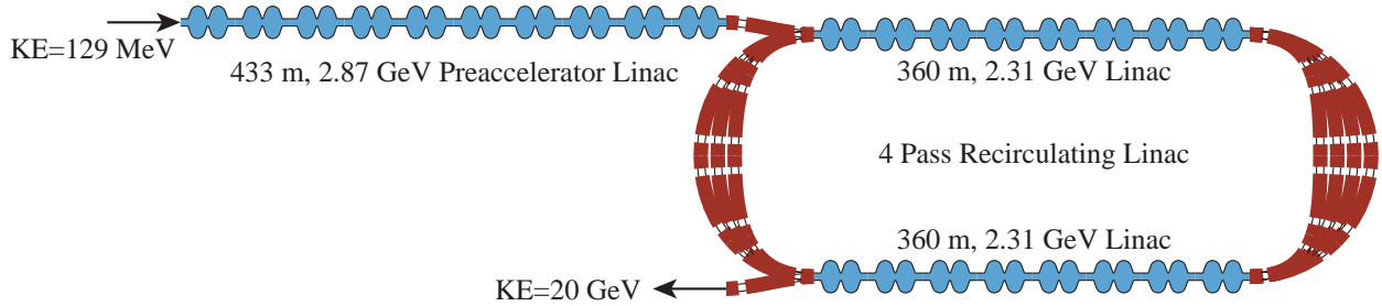
FIG. 21: (Color)Accelerating system layout.
