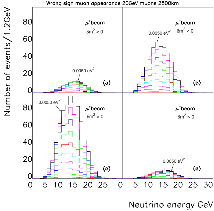
FIG. 4: (Color) The wrong sign muon appearance rates for a 20 GeV muon storage ring at a baseline of 2800 km with 10^{20} decays and a 50 kiloton detector for (a) \mu^+ stored and negative \delta m_{32}^2 , (b) \mu^- stored and negative \delta m_{32}^2 , (c) \mu^+ stored and positive \delta m_{32}^2 , (d) \mu^- stored and positive \delta m_{32}^2 . The values of |\delta m_{32}^2| range from 0.0005 to 0.0050 \text{eV}^2 in steps of 0.0005 \text{eV}^2 . Matter enhancements are evident in (b) and (c).
