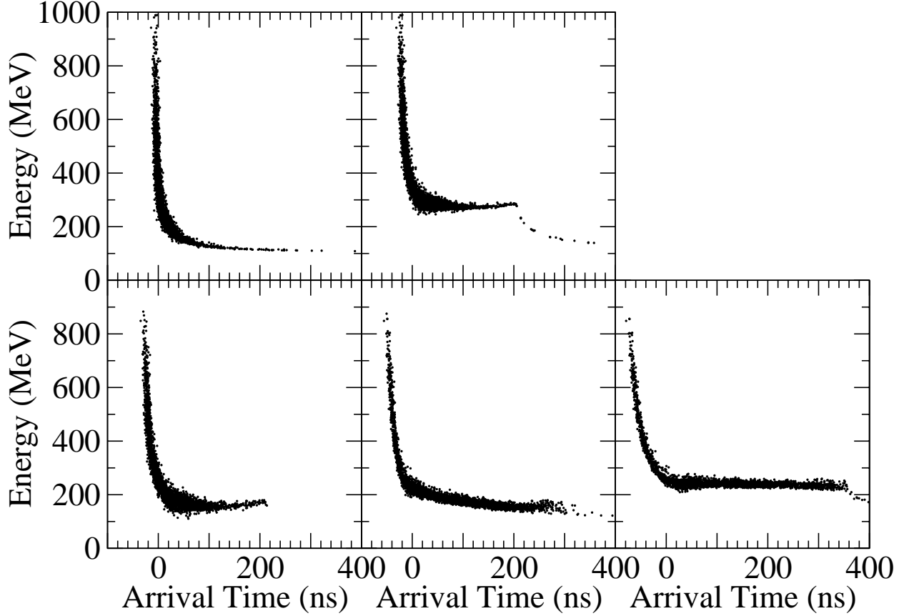
FIG. 16: Evolution of the beam distribution in the phase rotation section. The graphs show the distribution before the phase rotation, after the first induction linac (top row, left to right), after mini-cooling, and after the second and third induction linacs (bottom row).
