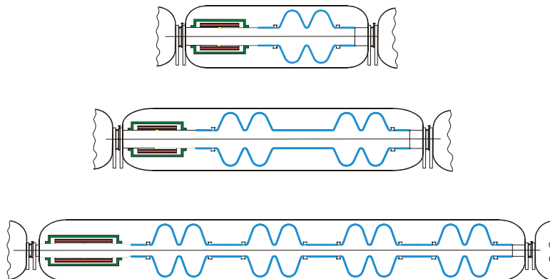
FIG. 22: (Color)Layouts of short (top), intermediate (middle) and long (bottom) cryomodules. Blue lines are the SC walls of the cavities. Solenoid coils are indicated in red.
