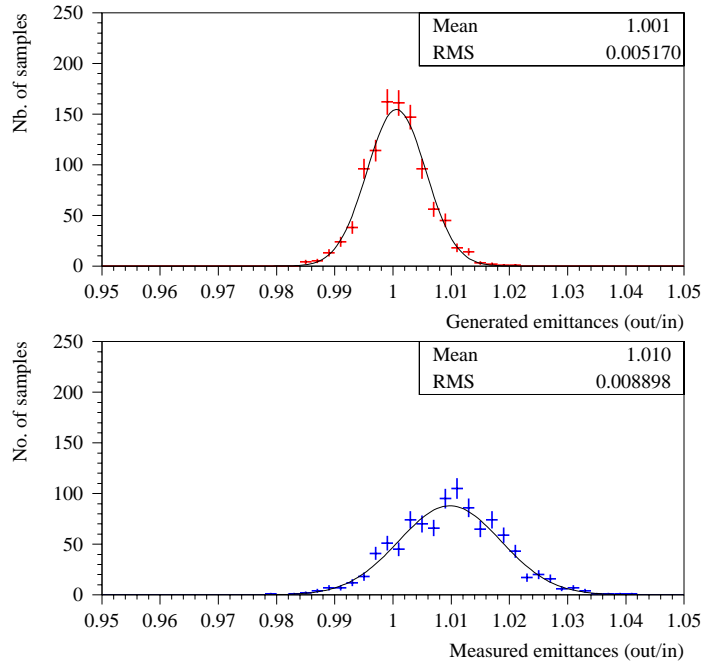
FIG. 49: (Color) Distribution of ratios of output to input six-dimensional emittance for 1000 simulated experiments, each with 1000 accepted muons. The top figure shows the distribution of this ratio for the emittances as generated by simulation; the bottom figure, as “measured” in the simulated experiments. The curves are Gaussian fits to the points.
