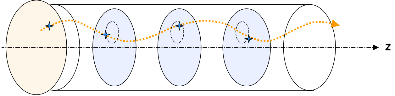
FIG. 46: (Color) Conceptual layout of MICE upstream spectrometer: following an initial time-of-flight (TOF) measurement, muons are tracked using detector planes located within a solenoidal magnetic field. Although in principle three x, y measurements as shown suffice to determine the parameters of each muon’s helical trajectory, in practice additional measurement redundancy will be employed; for example, a fourth measurement plane can be used to eliminate very-low-momentum muons that would execute multiple cycles of helical motion. A similar spectrometer (but with the time-of-flight measurement at the end) will be used downstream of the cooling apparatus.
