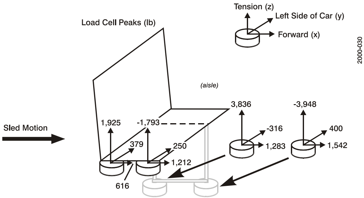
Figure A-2. Experiment No. 2-1 - Forward-Facing Row-to-Row Commuter Seats, Trailing Car Front Row Seat Attachment Loads (Maximums).
