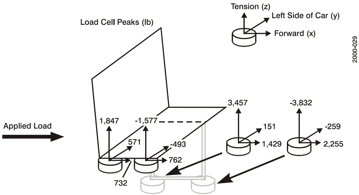
Figure A-1. Experiment No. 1-1 – Forward-Facing Row-to-Row Commuter Seats, Lead Car Front Row Seat Attachment Loads (Maximums)
