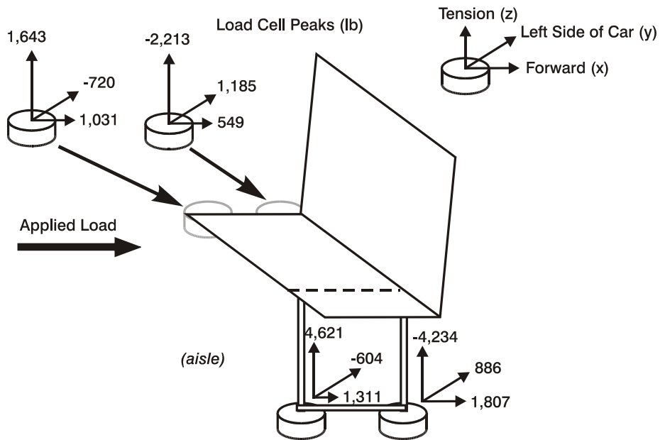
Figure A-4. Experiment No. 1-3 - Rear-Facing Commuter Seat, Lead Car. Seat Attachment Loads (Maximums)
