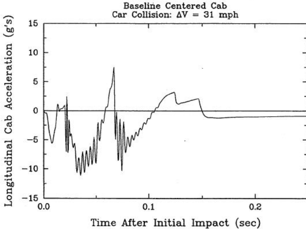
Figure 14. The Cab Car Crash Pulse Corresponding to the Centered Cab Car/Locomotive Collision at a 31 mph Closing Speed
