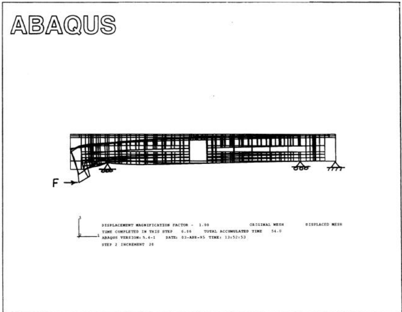
Figure 7. An Example of Predicted Cab Car Underframe Deformation for a Load Applied to the Draft Stop (about 2.5 ft of crush)
