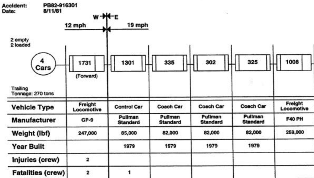
Figure 1. Description of a Cab Car Accident in a Push-Pull Configuration
