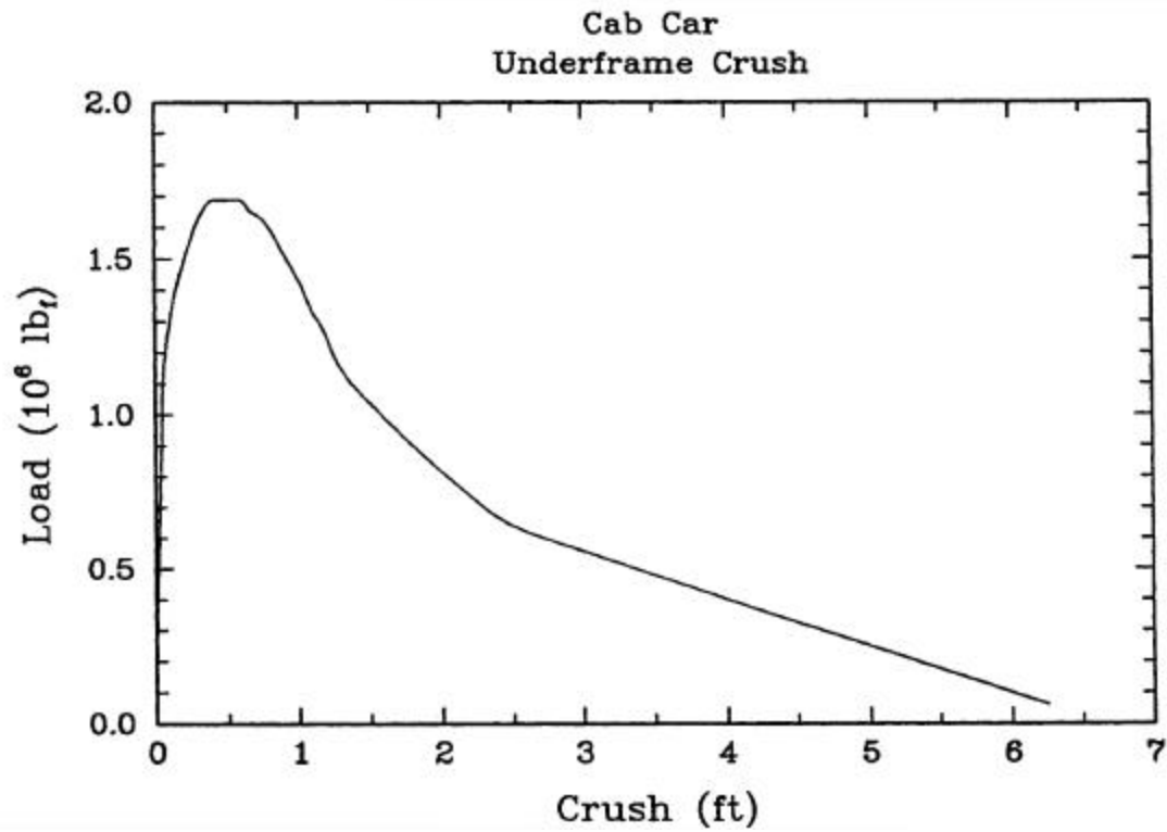
Figure 6. The Idealized Load-Crush Curve for Longitudinal Loading Applied at the Draft Stop of the Underframe
