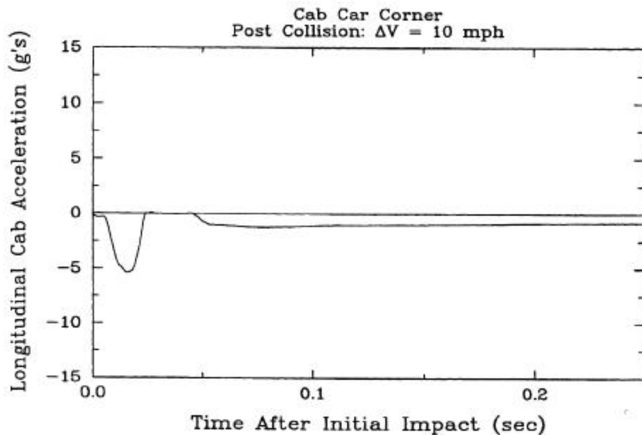
Figure 16. The Cab Car Crash Pulse Corresponding to the Corner Post Collision at a 10 mph Closing Speed
