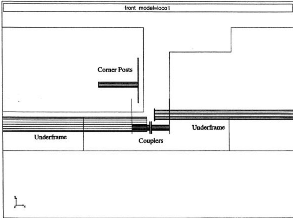
Figure 12. An Illustration of the Vehicle Components Included in the Collision Dynamics Model
