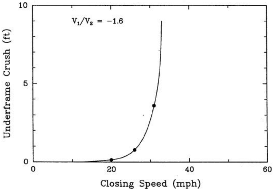
Figure 13. Predicted Cab Car Underframe Crush vs. Closing Speed for Cab Car/Locomotive Crash Scenario
