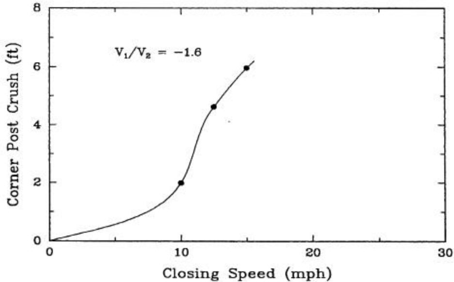
Figure 15. Predicted Cab Car Corner Post Crush vs. Closing Speed for Cab Car/Locomotive Crash Scenario
