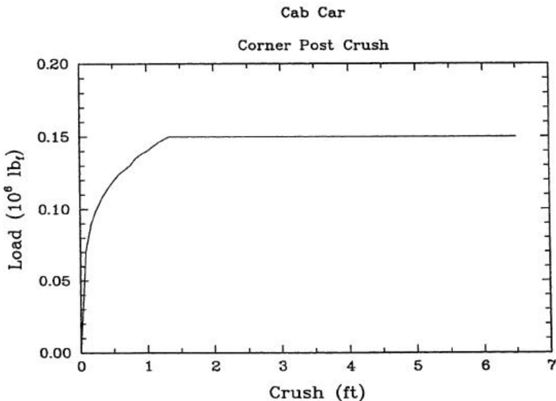
Figure 8. The Idealized Load-Crush Curve for Longitudinal Loading Applied Near the Base of a Corner Post
