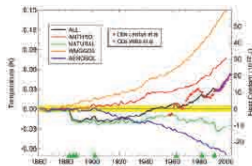
Fig. 3.11. Change in global mean ocean temperature (left axis) and ocean heat content (right axis) for the top 3000 m due to different forcings in the GFDL model. WMGGAS includes all greenhouse gases and ozone; NATURAL includes solar and volcanic aerosols (events shown as green triangles on the bottom axis). Observed ocean heat content changes are shown as well. From Delworth et al., 2005.
