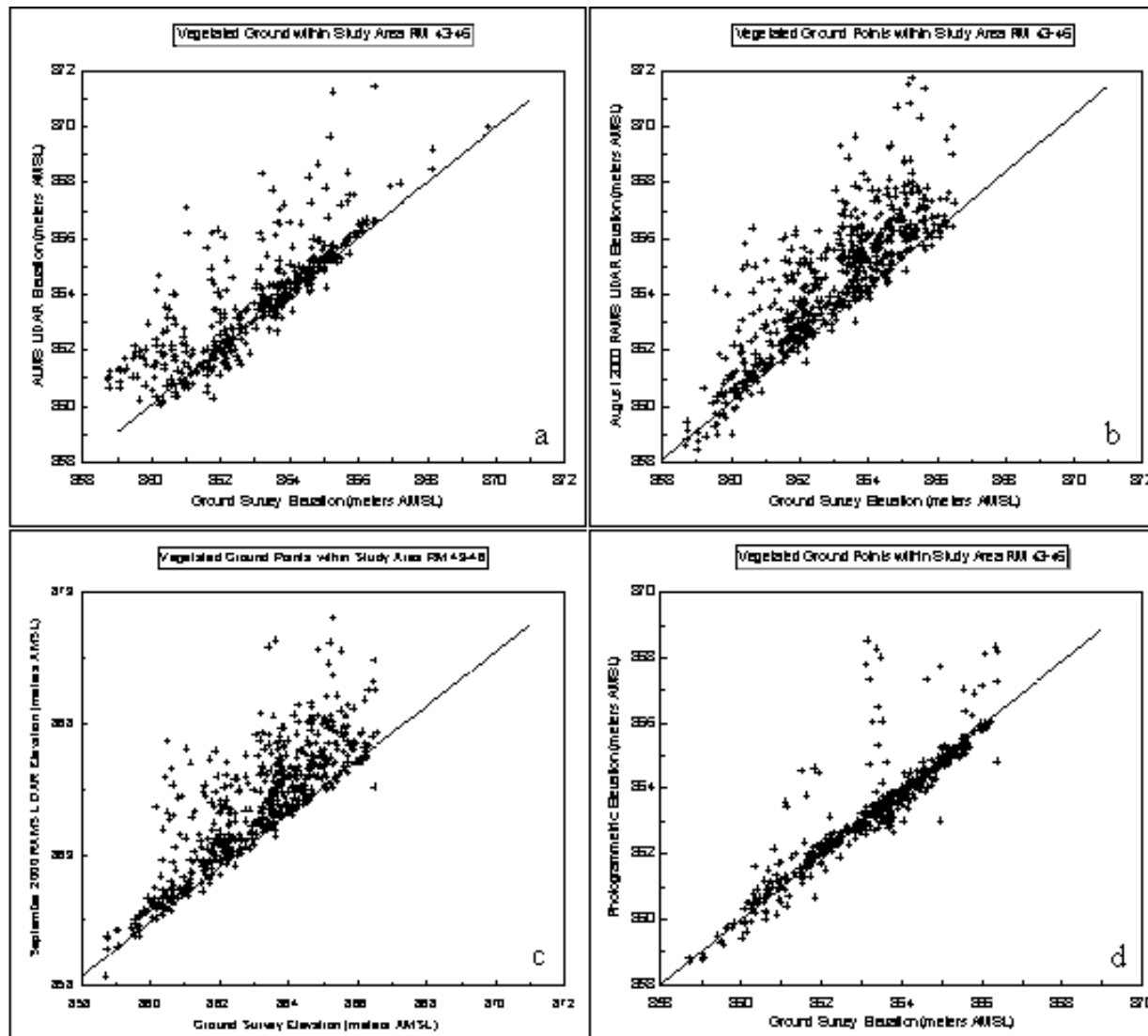
Figure 37. Scatter plots of airborne elevations and surveyed ground elevations on vegetated surfaces within study area RM 43-46. Solid lines are the least-squares regression lines from the bare-ground evaluations shown in Figures 31-34.
