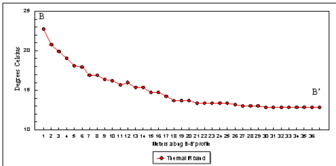
Figure 10. Calibrated, airborne water temperatures along profile B-B'.
