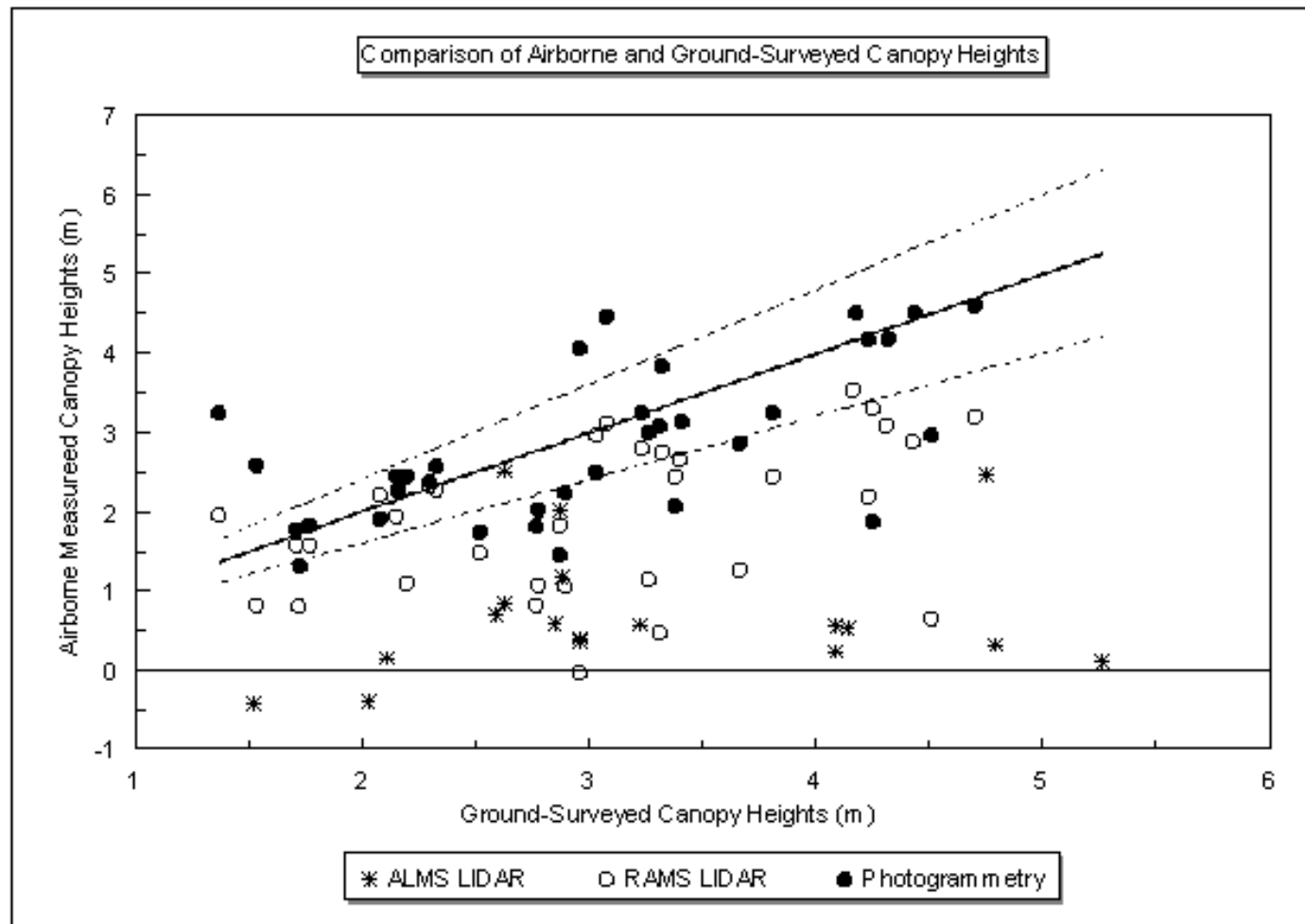
Figure 20. Scatter plot of airborne-derived and ground-surveyed canopy heights. Solid line represents perfect agreement between airborne-derived and ground-surveyed canopy heights. Dashed lines represent the 20% error limit on height measurements.
