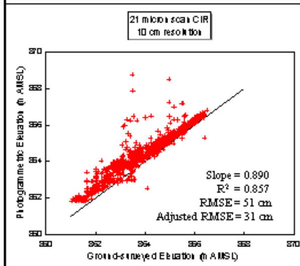
Figure 39. Comparison of photogrammetric ground elevations derived from 10-cm scanned CIR film image data with surveyed ground elevations. Line represents perfect agreement. Adjusted RMSE values derived from photogrammetric elevations have been adjusted downward for an observed average vertical offset from ground-survey elevation data.
