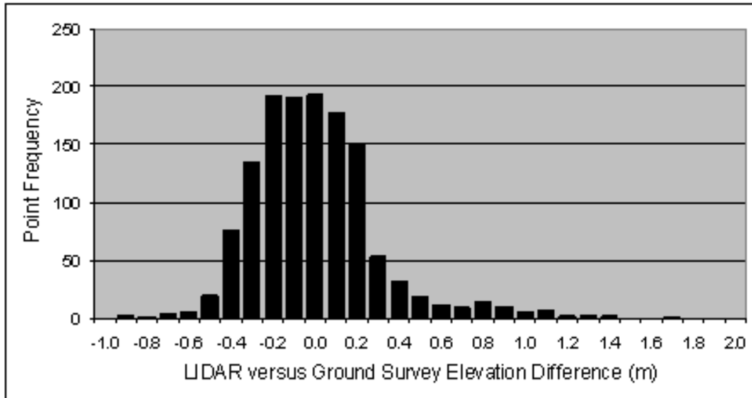
Figure 27. Point frequency distribution of differences between LIDAR elevations on the mainstem and ground-survey elevations of the adjacent water's edge.
