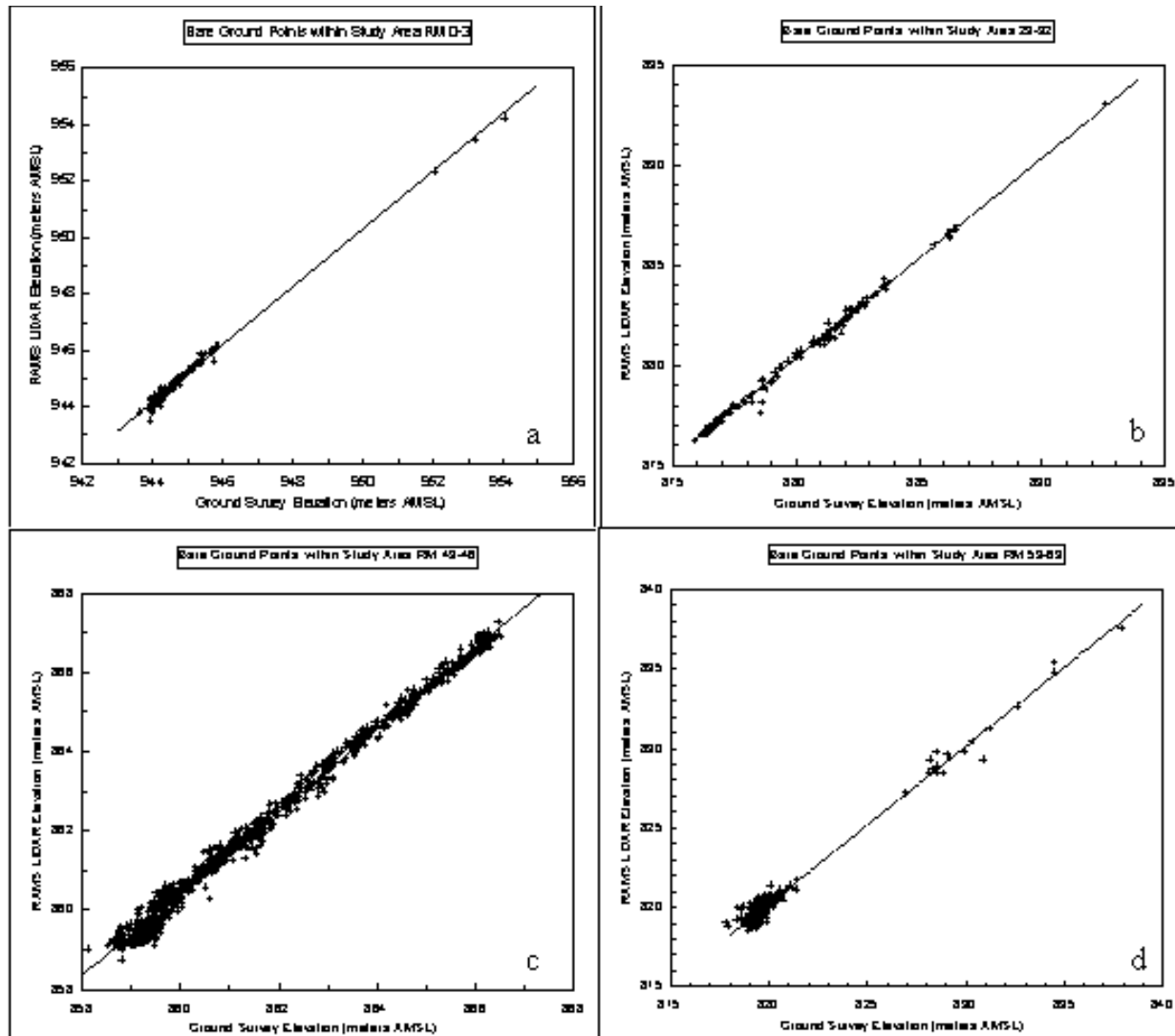
Figure 34. Scatter plots of September 2000 RAMS LIDAR elevations and ground survey elevations on bare ground for study areas (a) RM 0-3, (b) RM 29-32, (c) RM 43-46, and (d) RM 59-63. Solid lines are least-squares regression lines; dashed lines represent perfect agreement between LIDAR and ground-survey elevations.
