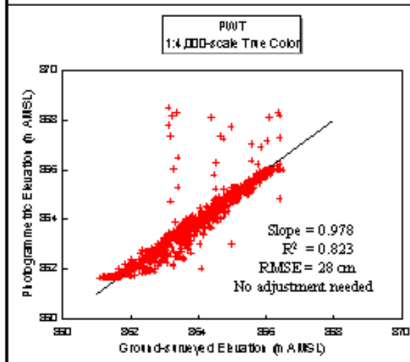
Figure 40. Comparison of photogrammetric ground elevations derived by Pacific Western Technologies (PWT) using 1:4,000-scale true-color film with surveyed ground elevations. Line represents perfect agreement.
