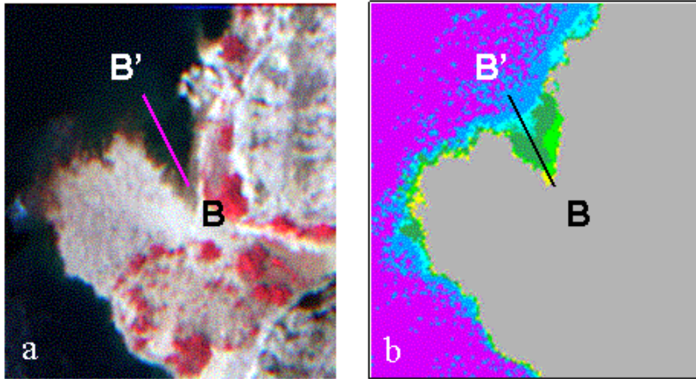
Figure 9. Color-infrared image (a) and color-coded airborne water-temperature map (b) of the left bank of the Colorado River at the mouth of Tatahatso Wash (river mile 43.2). Image width is 128 meters. On (b) land is gray and water colors correspond to temperature scale shown below.
