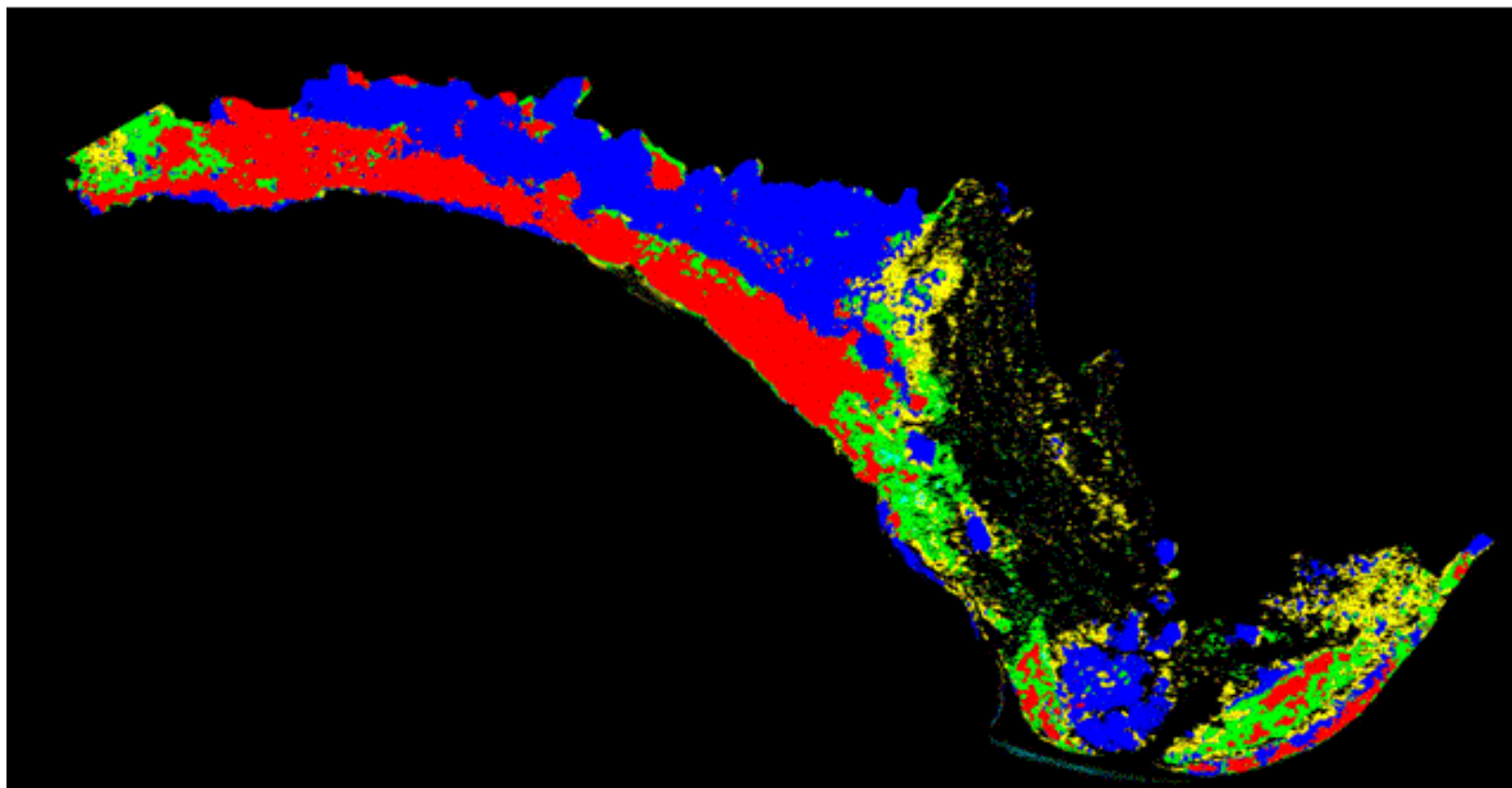
Figure 14. Vegetation classification map of study site RM68.2 produced from maximum likelihood classification of color-infrared (CIR) band data (acquired at 11-cm resolution in July, 2000) and derivative texture data. Map excludes bare ground. Classification accuracy is 62.6% for Kearsley and Ayers vegetation units.
