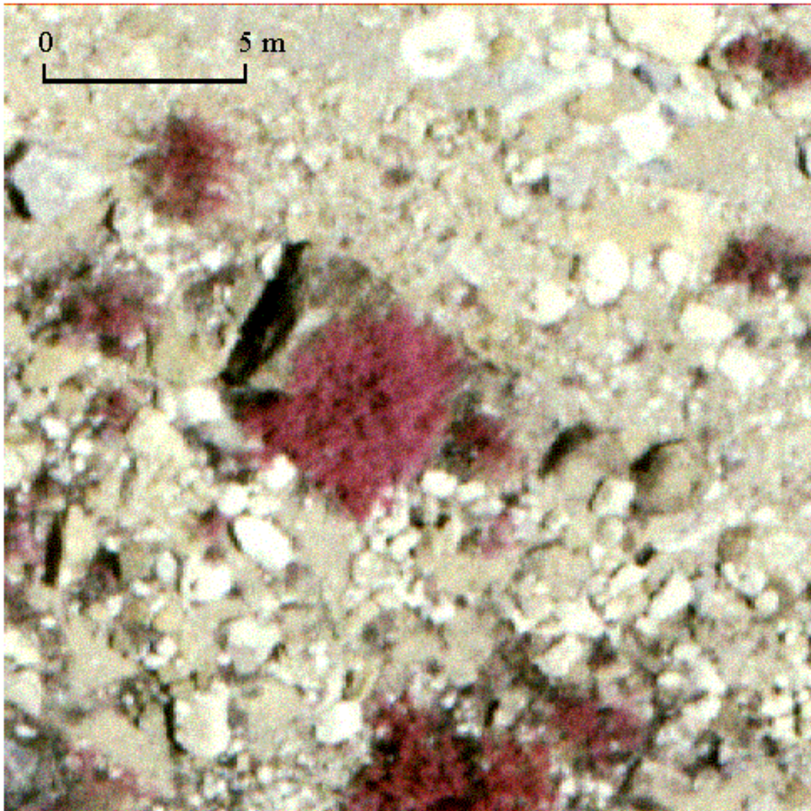
Figure 31. Color-infrared (CIR) image (10-cm resolution produced by a 21-micron scan of 1:4,800-scale film) of debris flow surface at RM 43 study area. Vegetation has very distinct shades of red. Some geologic materials tend to be washed out or saturated white. Image represents the original orientation (no geometric resampling) and the original color balance of the scanned image. Control panel visible on previous images (Figures 23-25) was not present on surface during this image acquisition.
