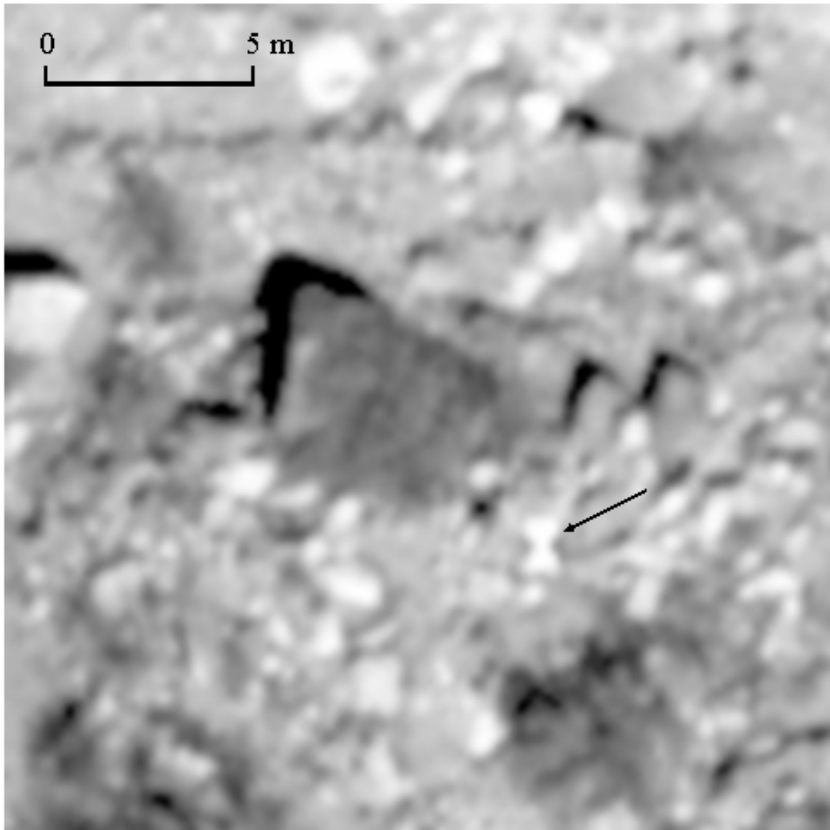
Figure 30. Digital panchromatic image (18-cm resolution) of debris flow surface at RM 43 study area. Vegetation is dark and difficult to distinguish from shadows cast by large rock fragments and even some of the rock fragments themselves. Differences between geologic materials are also difficult to distinguish. This image is a portion of an orthorectified mosaic and has therefore been resampled to some degree. Four-foot control panel near image center (indicated by arrow) has a white hourglass shape.
