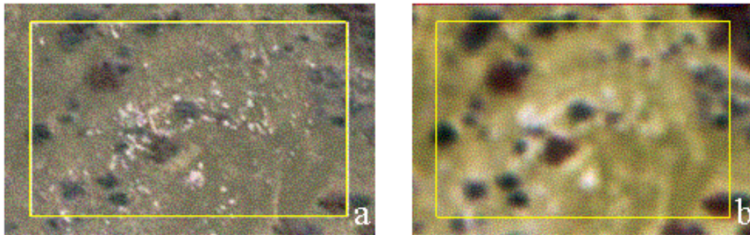
Figure 1. Archaeological structure on the northwest side of Unkar delta shown on natural-color images at (a) 11-cm and (b) 100-cm resolution. Image width is 27.9 meters. Multiple archaeological foundations are easily visible at 11-cm resolution, but are not uniquely discernible from natural alluvial surface materials at 100-cm resolution.
