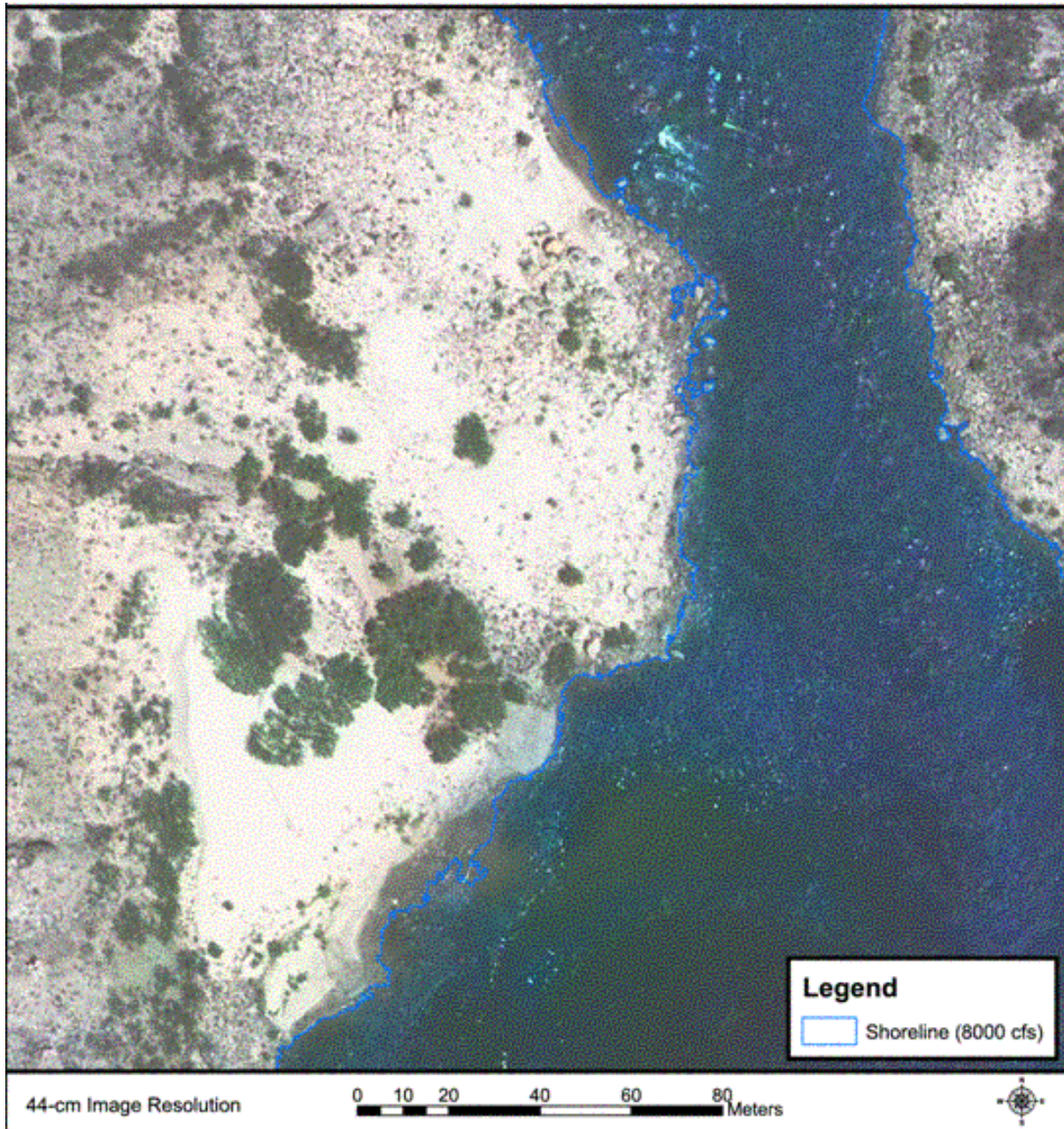
Figure 3. Natural-color image of Malgosa Canyon (RM 58) produced from ISTAR image data collected May 2002. Shoreline at 8,000 cfs is indicated by blue line, vegetation is green, and young sand deposits are bright white.
