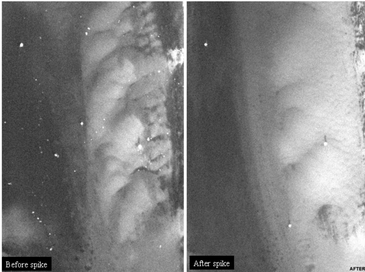
Figure 25. High-gain panchromatic images, contrast stretched to show detail on channel substrate before (left image) and after (right image) the high-flow spike in September, 2000 (Chavez et al., 2002a). Images are the lower subarea shown in Figure 19.
