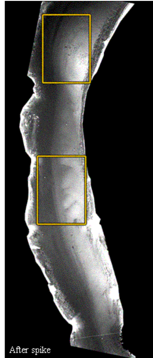
Figure 23. High-gain panchromatic images of a part of the main channel in Glen Canyon acquired in August, 2000 (left image) before the flow spike in early September, 2000 and one week later after the flow spike (right image). Both imagers were contrast stretched to more clearly show substrate information, at the expense of land surfaces (Chavez et al., 2002a). Boxed areas are shown at higher resolutions in the next figures.
