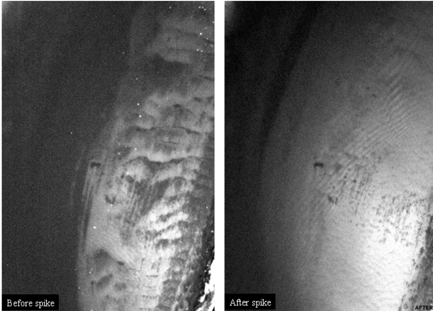
Figure 24. High-gain panchromatic images, contrast stretched to show detail on channel substrate before (left image) and after (right image) the high-flow spike in September, 2000 (Chavez et al., 2002a). Images are the upper subarea shown in Figure 19.
