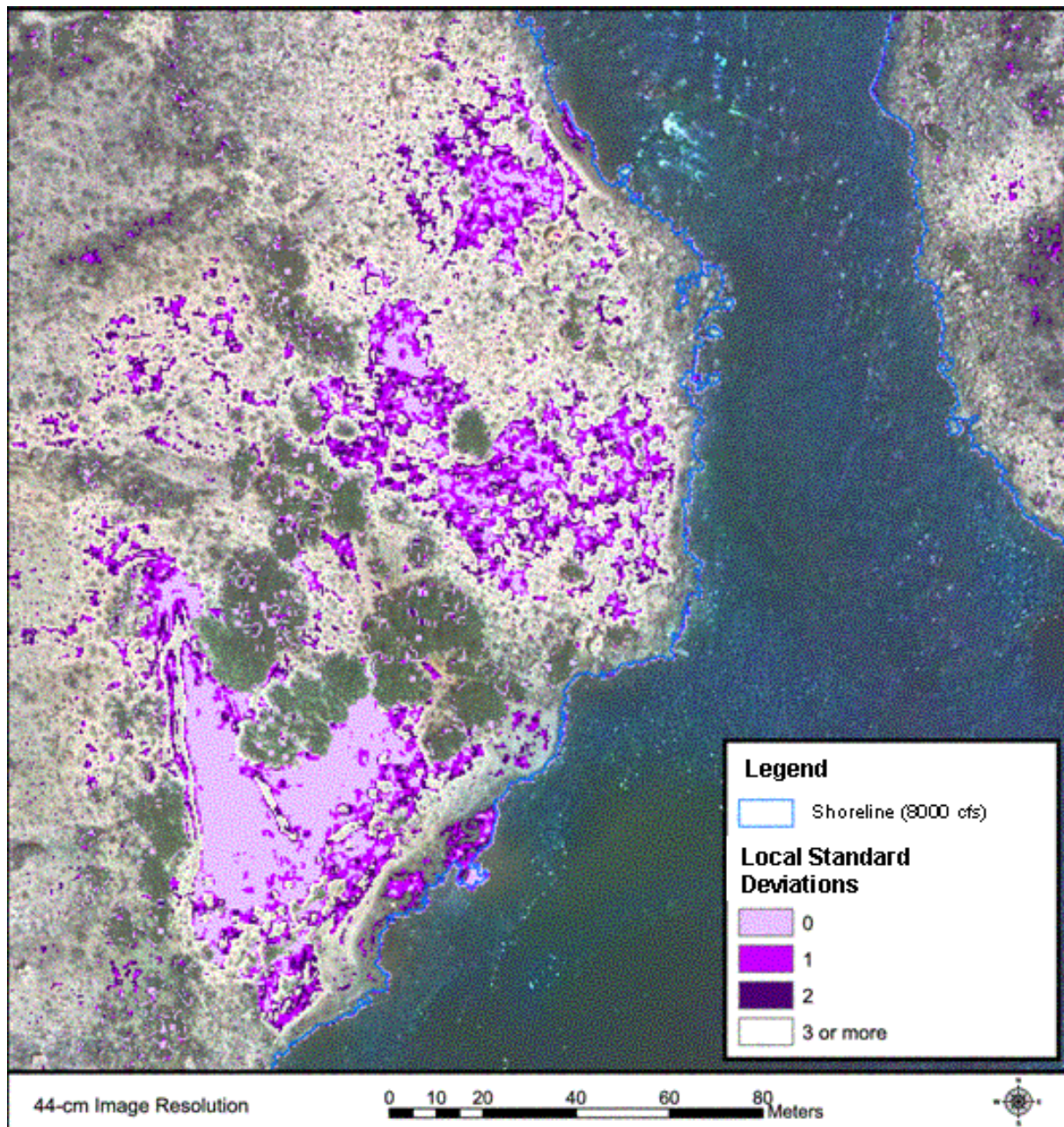
Figure 5. Distribution of surfaces with different relative textures (roughness) based on the average variance in near-infrared-band reflectance within an areal dimension that was found optimal for separating smooth and rough surfaces. Roughness classes are superposed on the natural-color image shown in Figure 3. Shoreline at 8,000 cfs is indicated by blue line.
