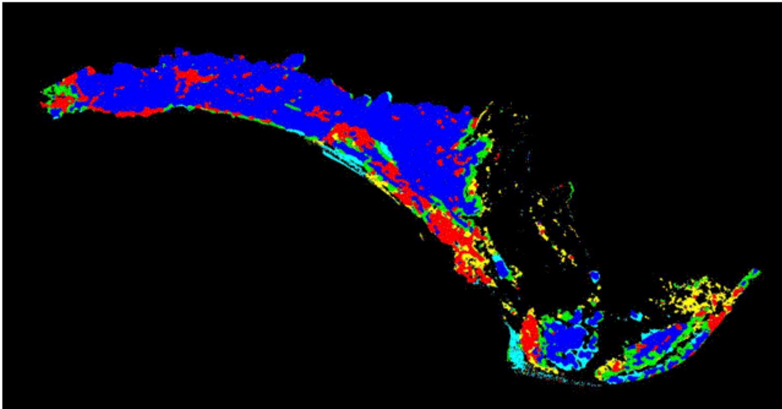
Figure 17. Vegetation classification map of study site RM68.2 produced from maximum likelihood classification of color-infrared (CIR) band data (acquired at 30.5-cm resolution in March, 2000) and derivative texture data. Map excludes bare ground. Classification accuracy is 53.8% for the Kearsley and Ayers vegetation units.
