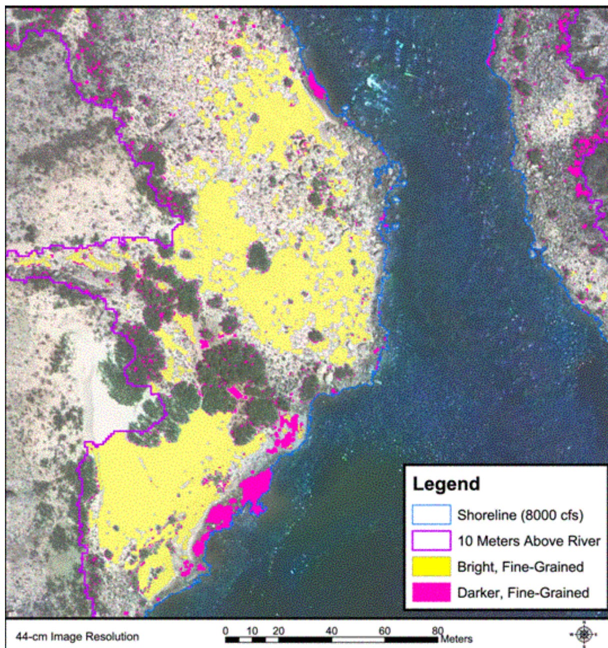
Figure 6. Distribution of near-shore, bright and dark, fine-grained inorganic surface materials based on surface brightness, color, texture, and elevation data. Sediment classes are superposed on the natural-color image shown in Figure 3. Shoreline at 8,000 cfs is indicated by blue line; area within 10 meters of elevation above the water's edge is indicated by a orchid-colored line.
