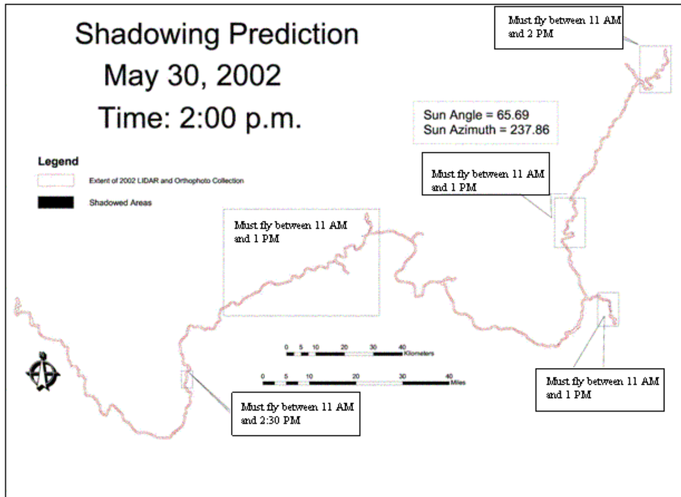
Figure 19. Results from shadow analysis for May 30, 2002 at 2:00 PM. Red line indicates limits of corridor monitoring. Black areas within red zone indicates shadows at the designated time and day. This analysis was used to establish the latest time on a given day for shadow-fee data collection for most of the corridor. Some areas (boxes) are more constrained.
