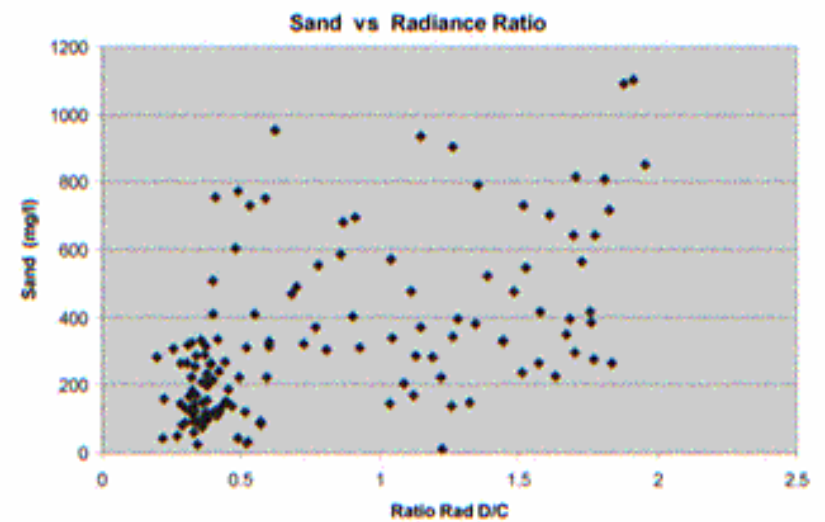
Figure 21. Relation between radiance ratios derived from ground measurements and (a) silt-clay and (b) sand concentrations that were recorded by water gages (Chavez et al., 2002b).
