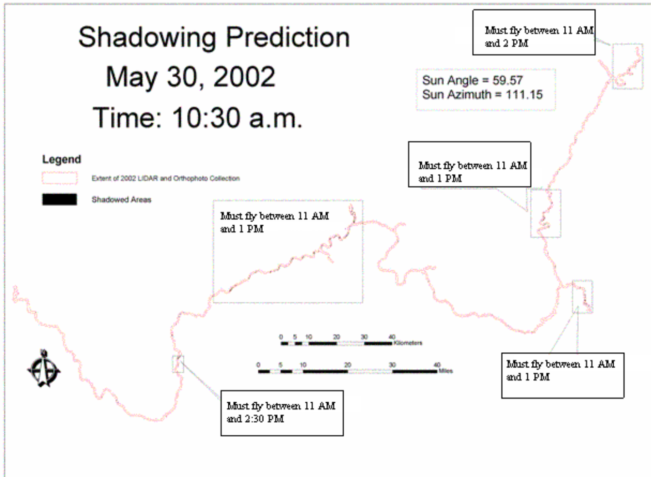
Figure 18. Results from shadow analysis for May 30, 2002 at 10:30 AM. Red line indicates limits of corridor monitoring. Black areas within red zone indicates shadows at the designated time and day. This analysis was used to establish the earliest time on a given day for shadow-fee data collection for most of the corridor. Some areas (boxes) are more constrained.
