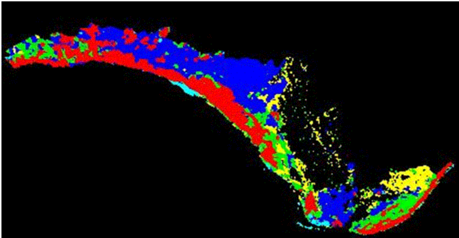
Figure 13. Vegetation classification map of study site RM68.2 produced from maximum likelihood classification of Daedalus multispectral band data (acquired at 100-cm resolution in July, 2000) and derivative texture data. Map excludes bare ground. Classification accuracy is 67.0% for the Kearsley and Ayers vegetation units.
