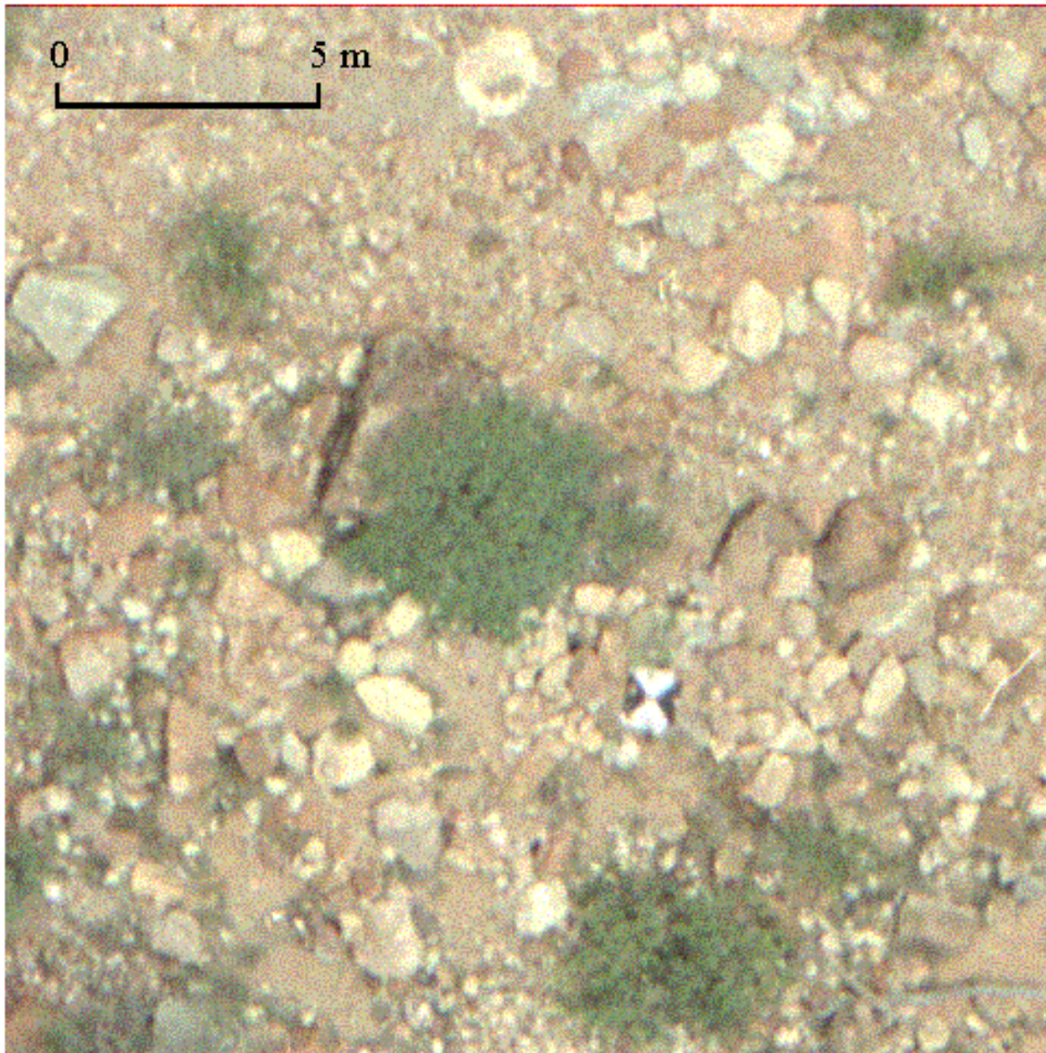
Figure 29. Natural-color image (6-cm resolution produced by a 15-micron scan of 1:4,000-scale film) of debris flow surface at RM 43 study area. Vegetation is green. Geologic materials have their natural colors with little or no saturation. Image represents the original orientation (no geometric resampling) and the original color balance of the scanned image. Scan resolution is near the limit of the film's resolution. Four-foot control panel near image center has a black-and-white hourglass shape.
