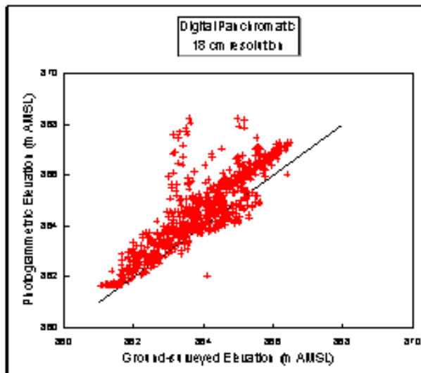
Figure 38. Comparison of photogrammetric ground elevations derived from 18-cm digital panchromatic image data with surveyed ground elevations. Line represents perfect agreement. Adjusted RMSE values derived from photogrammetric elevations have been adjusted downward for an observed average vertical offset from ground-survey elevation data.
