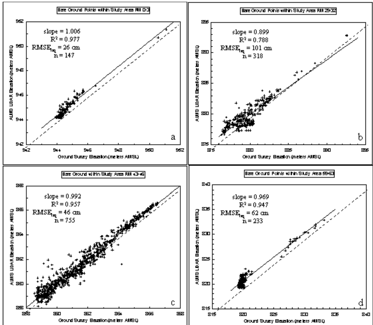
Figure 32. Scatter plots of March 2000 ALMS LIDAR elevations and ground survey elevations on bare ground for study areas (a) RM 0-3, (b) RM 29-32, (c) RM 43-46, and (d) RM 59-63. Solid lines are least-squares regression lines; dashed lines represent perfect agreement between LIDAR and ground-survey elevations.
