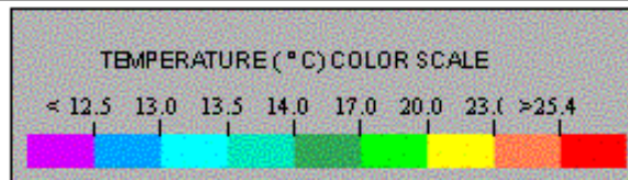
Figure 9. Color-infrared image (a) and color-coded airborne water-temperature map (b) of the left bank of the Colorado River at the mouth of Tatahatso Wash (river mile 43.2). Image width is 128 meters. On (b) land is gray and water colors correspond to temperature scale shown below.
