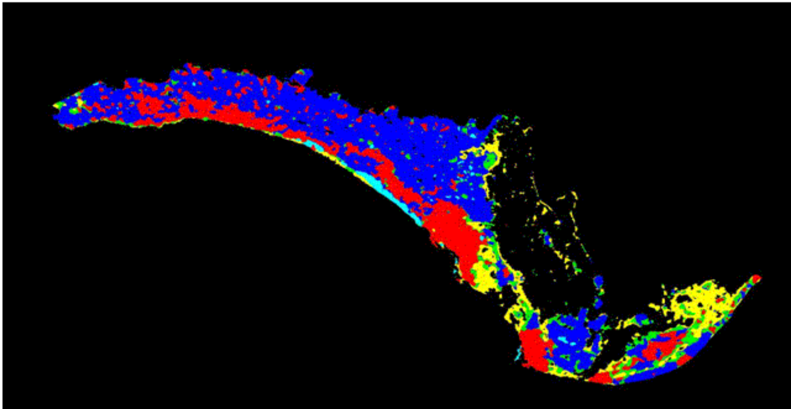
Figure 15. Vegetation classification map of study site RM68.2 produced from maximum likelihood classification of Emerge color-infrared (CIR) band data (acquired at 30.5-cm resolution in September, 1999) and derivative texture data. Map excludes bare ground. Classification accuracy is 59.2% for the Kearsley and Ayers vegetation units.
