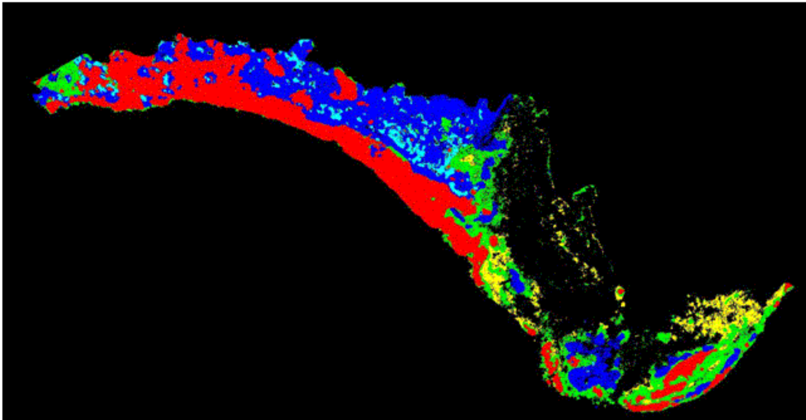
Figure 16. Vegetation classification map of study site RM68.2 produced from maximum likelihood classification of color-infrared (CIR) band data (acquired at 28-cm resolution in September, 2000) and derivative texture data. Map excludes bare ground. Classification accuracy is 58.0% for the Kearsley and Ayers vegetation units.
