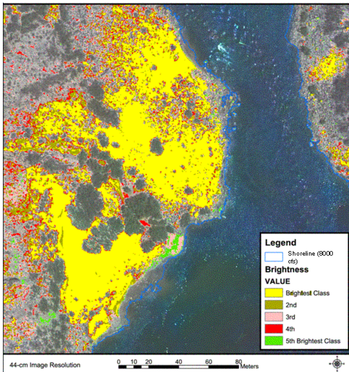
Figure 4. Distribution of inorganic materials of different ranges of brightness (albedo) based on surface brightness shown by the near-infrared-wavelength ISTAR image data. Brightness classes superposed on the natural-color image shown in Figure 3. Shoreline at 8,000 cfs is indicated by blue line.
