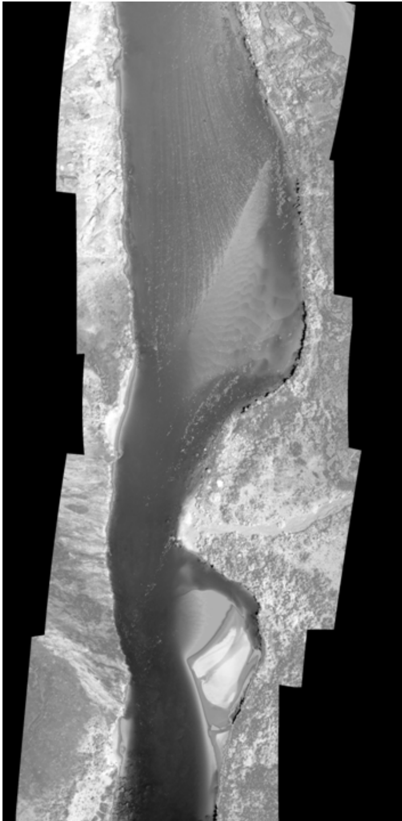
Figure 26. Image showing morphology of channel substrate compiled from high-gain, blue-green image of water areas and a normal-gain, near-infrared image of land areas. Area is south of LCR confluence near river mile 65.
