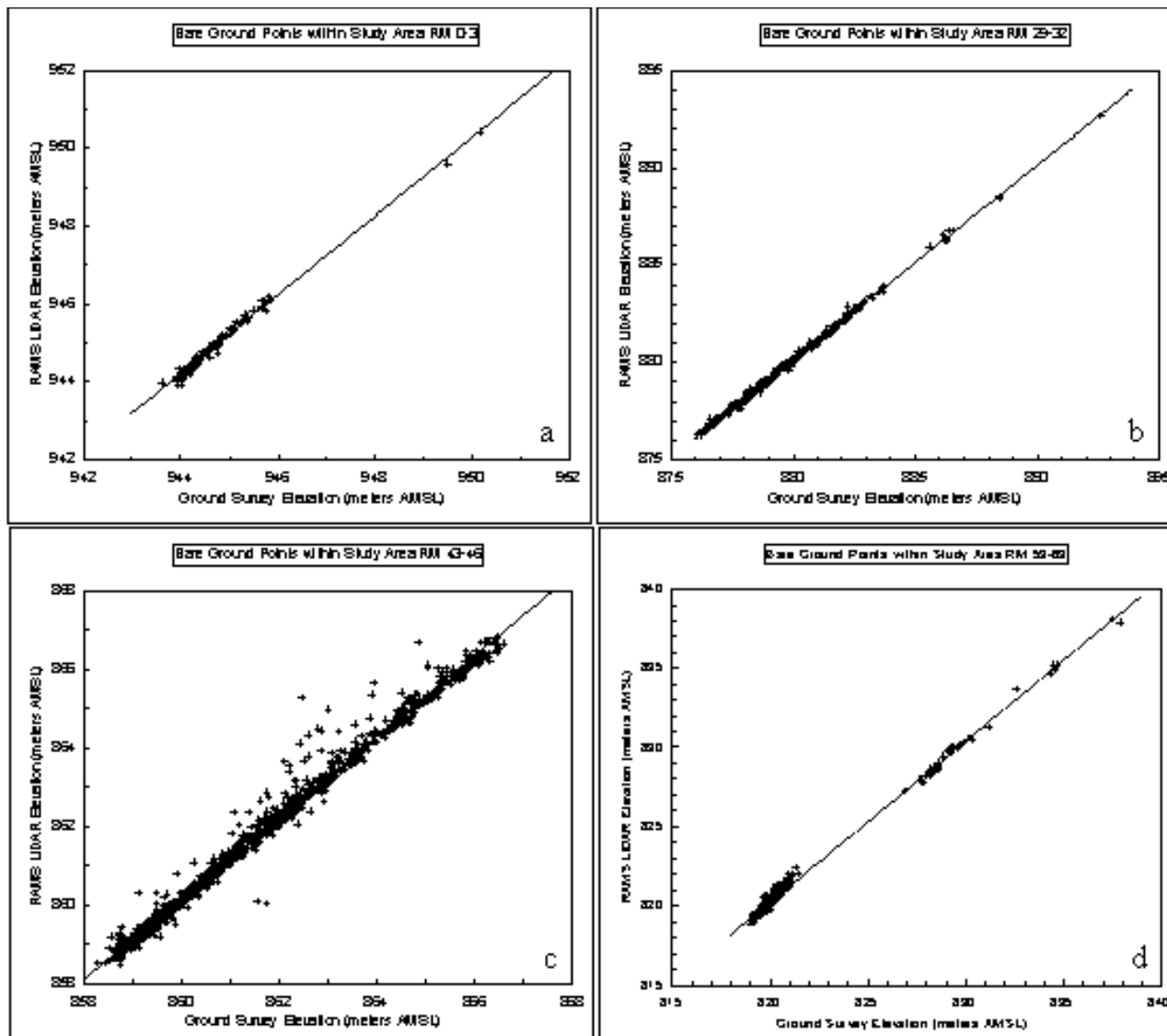
Figure 33. Scatter plots of August 2000 RAMS LIDAR elevations and ground survey elevations on bare ground for study areas (a) RM 0-3, (b) RM 29-32, (c) RM 43-46, and (d) RM 59-63. Solid lines are least-squares regression lines; dashed lines represent perfect agreement between LIDAR and ground-survey elevations.
