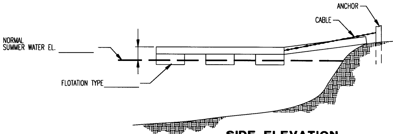
SIDE ELEVATION
