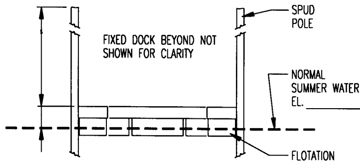
END ELEVATION NOT TO SCALE
