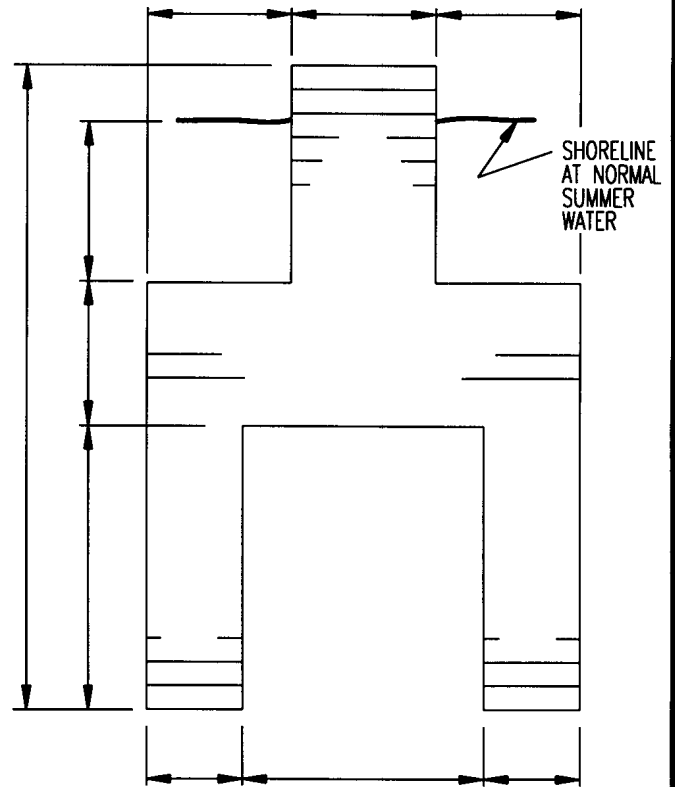
BOAT SLIP
