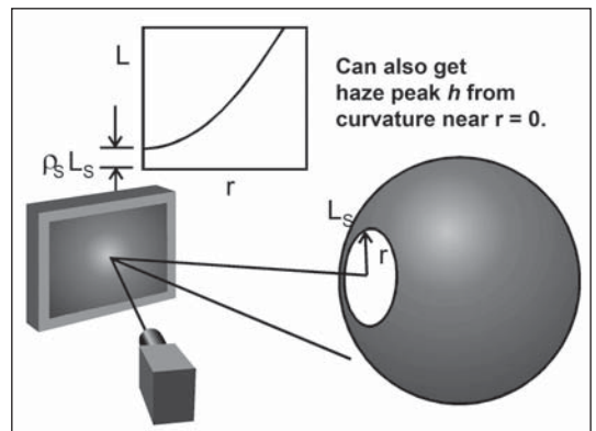
Variable Radius Source Method for Isolation of specular ( \zeta ) and haze ( h ) reflection components.
