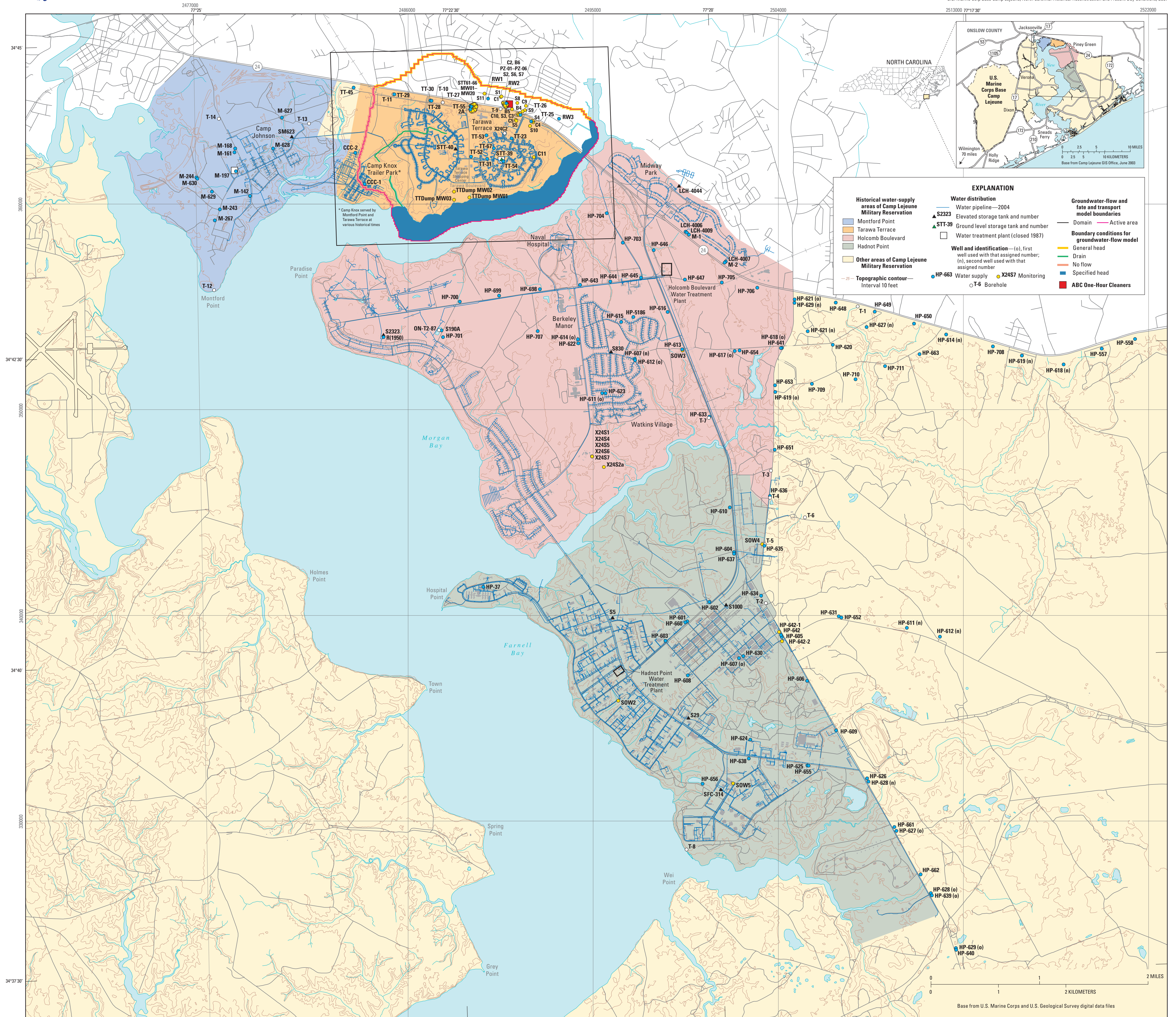
Location of Wells and Boreholes, Groundwater-Flow Model Boundary, and Present-Day (2004) Water-Distribution Systems Serving Tarawa Terrace, Holcomb Boulevard, and Hadnot Point and Vicinity, U.S. Marine Corps Base Camp Lejeune, North Carolina
