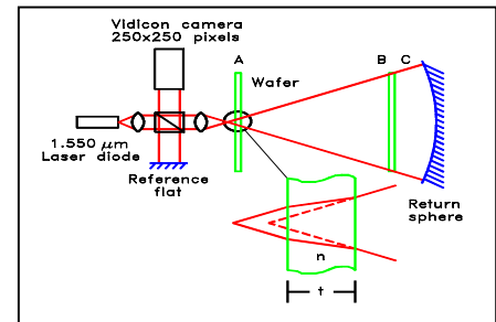
Measurement in 3 positions (A, B & C (B flipped)) provides center thickness, thickness variation and bow
