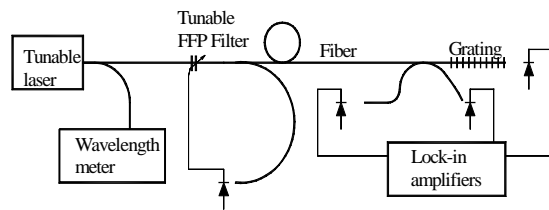
Component spectral reflectance and transmittance system
