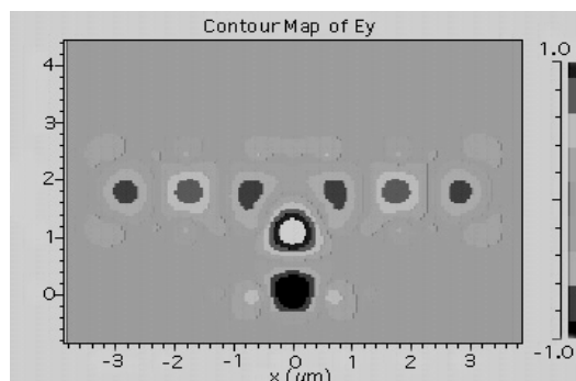
Modeled electric field of photonic crystal tee
