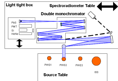
Facility for Automated Spectroradiometric CALibrations Spectral Irradiance Measurements
