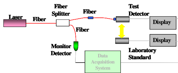
Layout of Optical Fiber Power calibration system.
