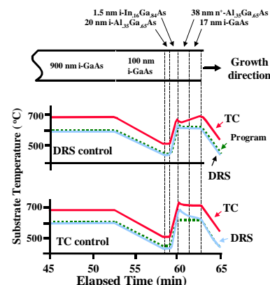
Temperature profiles during growth by MBE.
