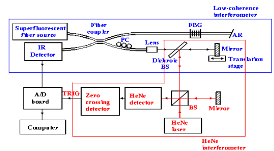
Low-Coherence Interferometer
