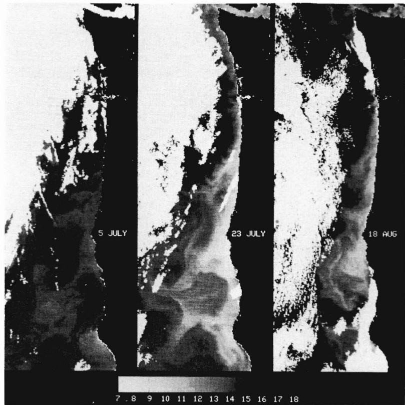
Figure 6. — Variations in the intensity and pattern of coastal upwelling off the Pacific Northwest between lat. 39°00'N and 48°30'N, July-August 1982. Sea surface temperature (°C) from NOAA-7 AVHRR channels 4 and 5. Clouds (white) screened with channel 2 data.
