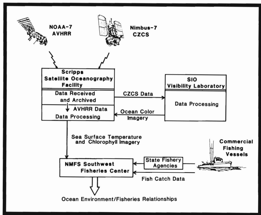
Figure 2. — Satellite data collection and processing network utilized by the National Marine Fisheries Service on the west coast.
