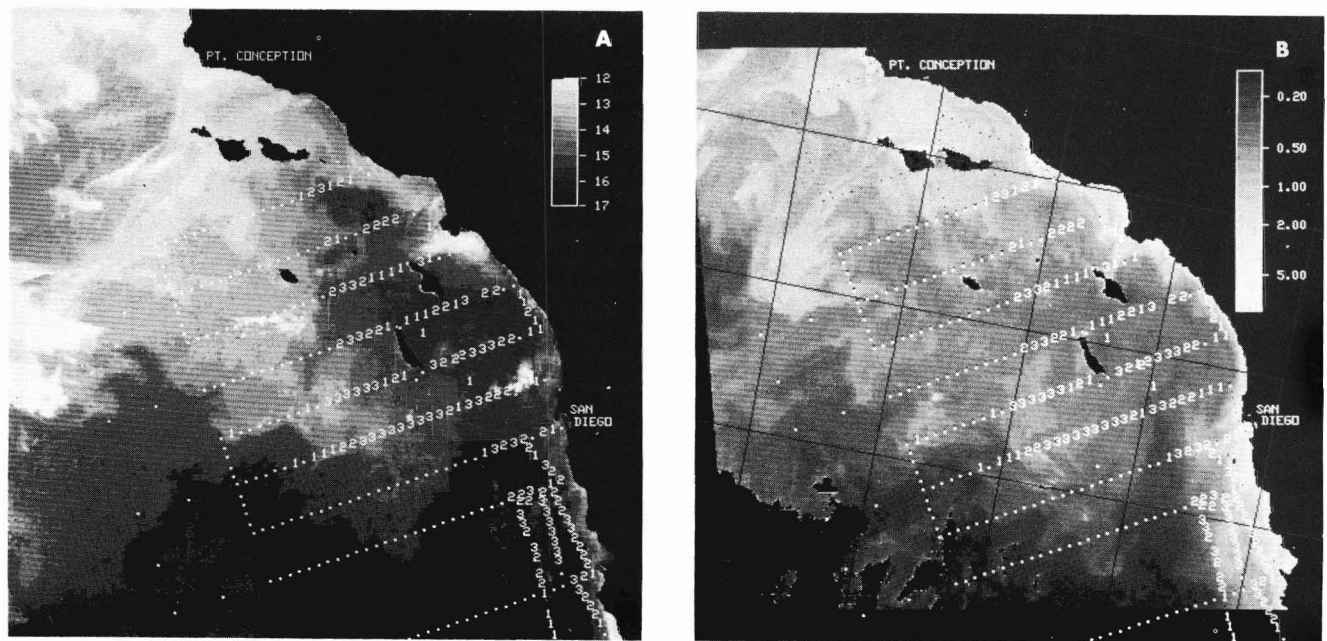
Figure 3.—Northern anchovy egg distribution, 20 March-10 April 1980; • = 0, 1 = 1-4, 2 = 5-17, 3 = 18-245 eggs/0.05 m 2 . Top photo (A) is sea surface temperature (°C) from NOAA-6 AVHRR, 7 April 1980; Photo B is of phytoplankton pigments (mg m -3 ) from Nimbus-7 CZCS, 8 April 1980.
