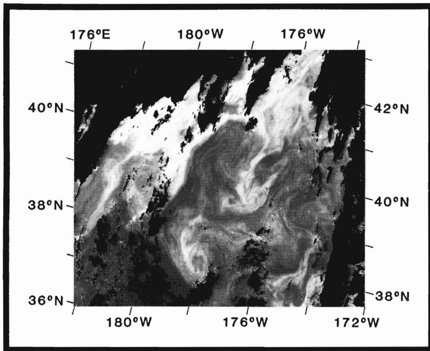
Figure 8. — Phytoplankton pigment concentration in a 600 × 600 km area of the central North Pacific, measured by the Coastal Zone Color Scanner, 30 June 1980. Black = clouds, darkest gray = 0.08 mg m -3 , white = 5.7 mg m -3 .
