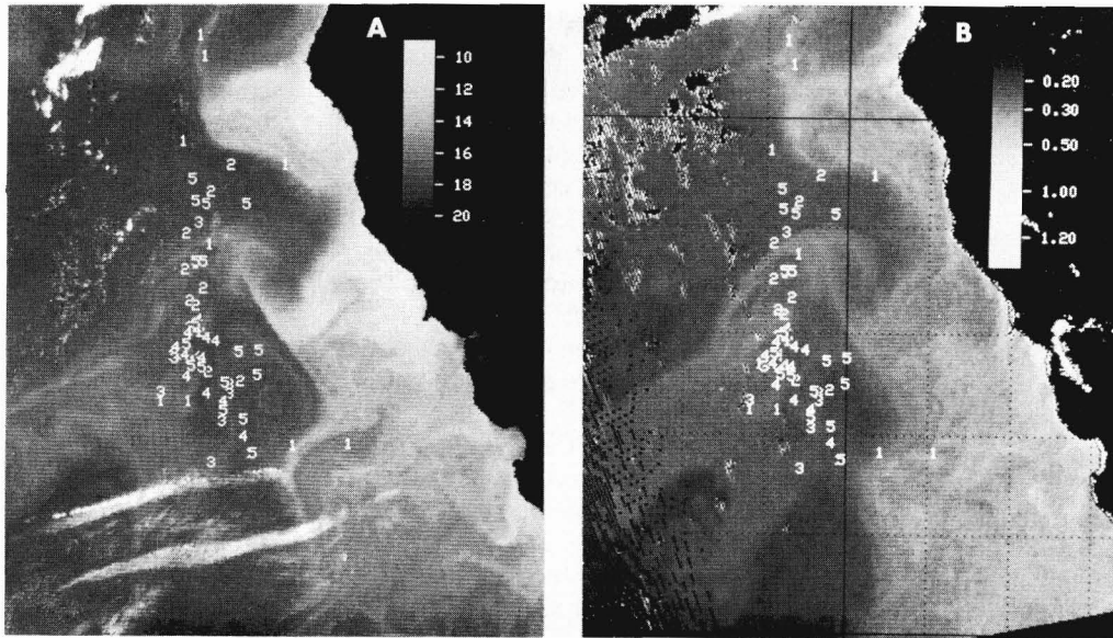
Figure 4.—Daily albacore catches off central California, 19-24 September 1981: 1 = 0-27, 2 = 33-63, 3 = 64-81, 4 = 87-140, 5 = 148-750 fish/boat. A is sea surface temperature ( ^{\circ}\text{C} ) from NOAA-7 AVHRR, 21 September 1981; B is phytoplankton pigments ( \text{mg m}^{-3} ) from Nimbus-7 CZCS, 22 September 1981.
