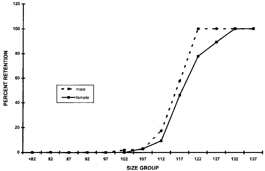
Figure 3.—Percent retention by sex of blue crabs by 5 mm carapace width size group in a 44.4 mm square.
