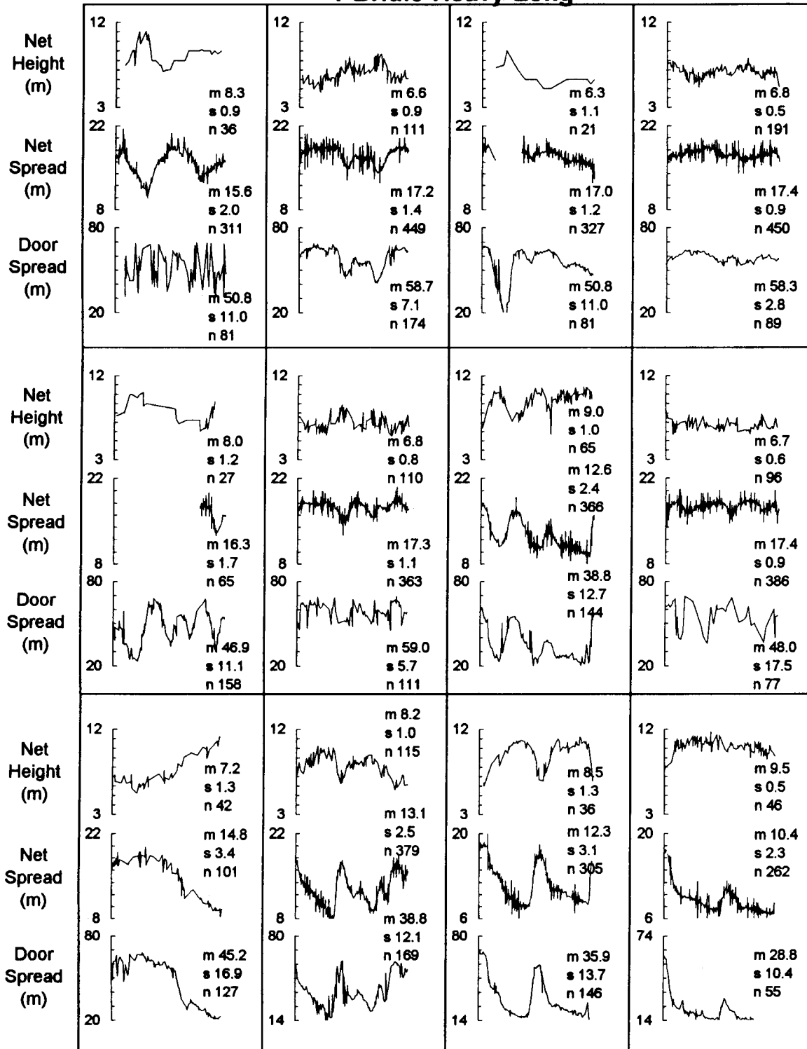
Figure 2.—SCANMAR net height, net width, and door spread during the course of each tow for the 1-bridle-heavy-long gear treatment (m=average, s=standard deviation, n=number of observations).
