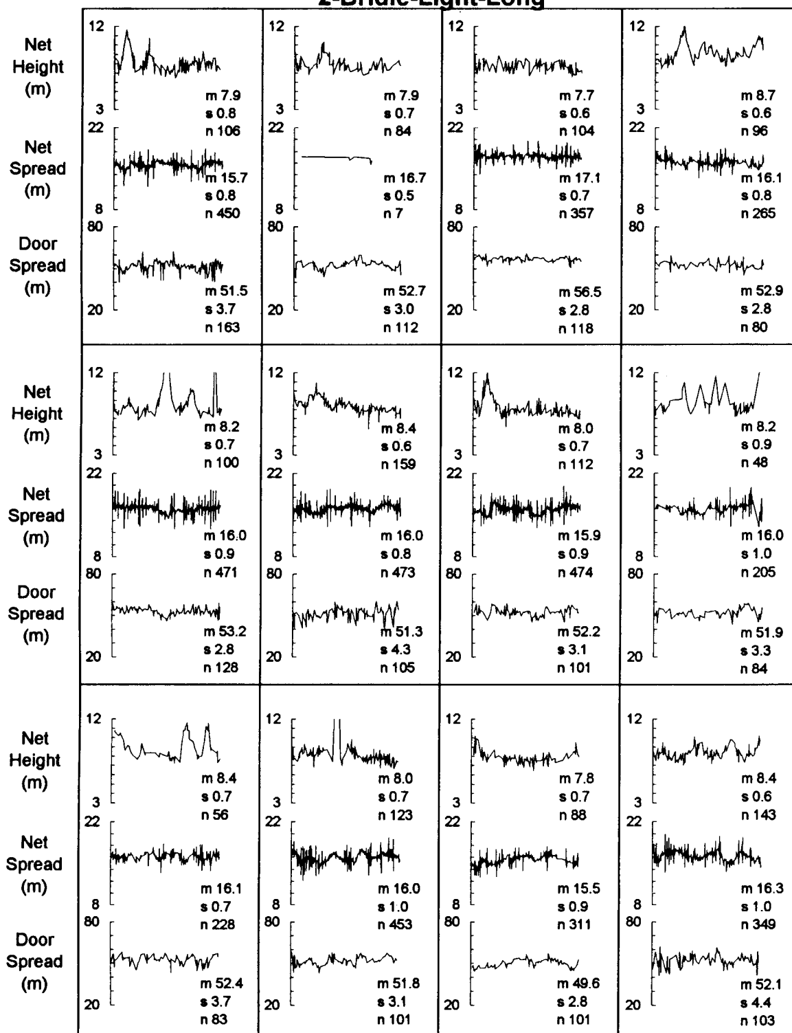
Figure 8.—SCANMAR net height, net width, and door spread during the course of each tow for the 2-bridle-light-long gear treatment (m=average, s=standard deviation, n=number of observations).
