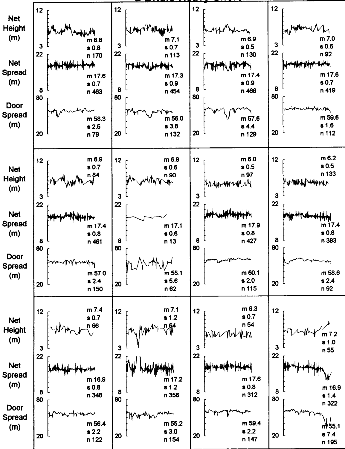
Figure 7.—SCANMAR net height, net width, and door spread during the course of each tow for the 2-bridle-heavy-short gear treatment (m=average, s=standard deviation, n=number of observations).
