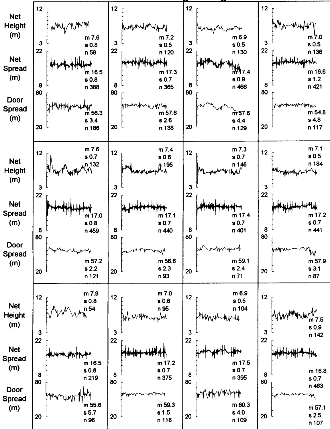
Figure 4.—SCANMAR net height, net width, and door spread during the course of each tow for the 1-bridle-light-long gear treatment (m=average, s=standard deviation, n=number of observations).
