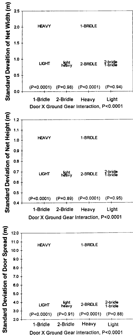
Figure 12.—Results of ANOVA to test the effects of the gear treatments and their interactions on the standard deviations of door spread, net width, and net height. Statistically significant effects ( P < 0.05 ) are with uppercase letters.
