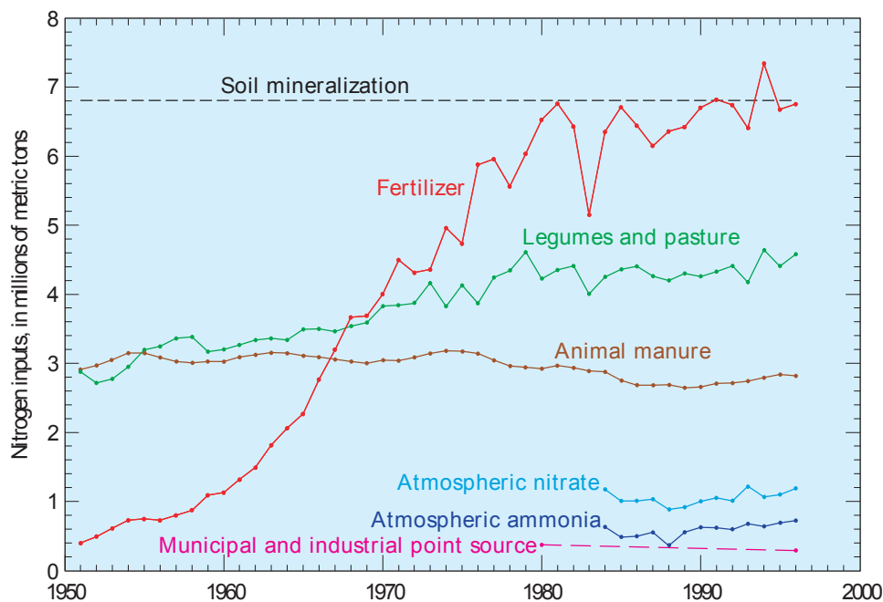
Figure 5. Annual nitrogen inputs to the Mississippi Basin from major sources.
