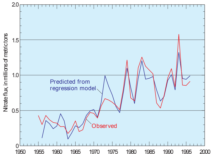
Figure 7. Annual nitrate flux to Gulf of Mexico and nitrate flux predicted from regression model.
