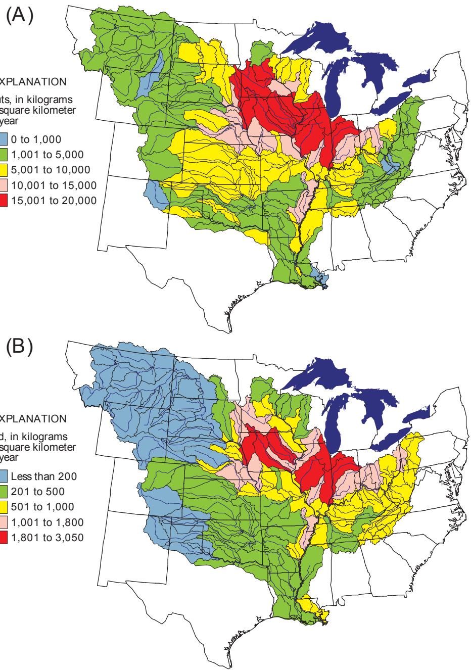
Figure 6. (A) Nitrogen inputs during 1992 and (B) average annual nitrogen yields of streams for 1980–96 (modified from Goolsby and others, 1999).
