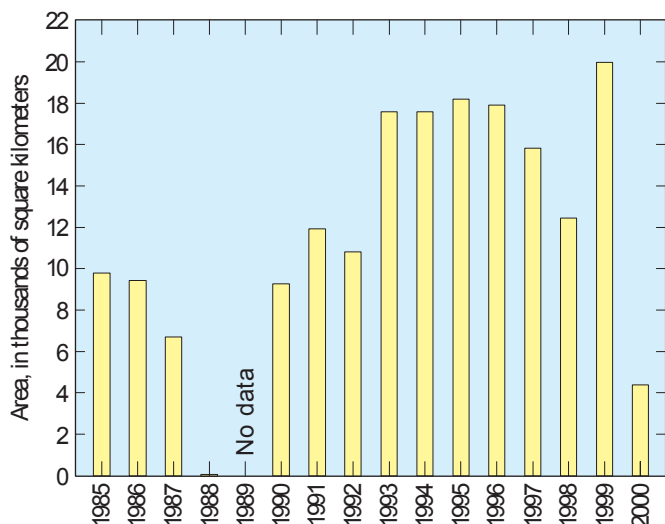
Figure 2. Area of hypoxic zone, 1985–2000 (source: N.N. Rabalais, Louisiana Universities Marine Consortium).
