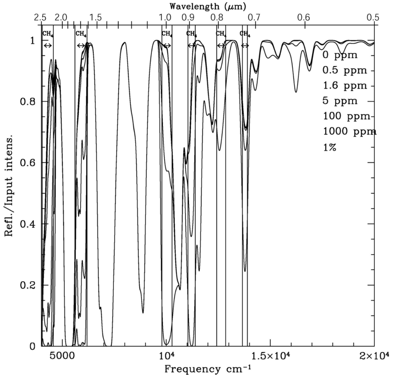
Figure 14. The visible reflection spectrum of methane is shown for seven abundance levels. At low abundances, methane would be detectable only at the longest wavelength, around 2.4 microns. However at moderate and high abundances methane could be detected in the 0.7, 0.8, 0.9, and 1.0 micron bands.
