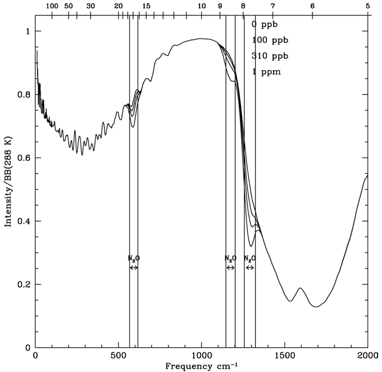
Figure 15. The thermal emission spectrum of nitrous oxide is shown for four abundance levels. As with methane, nitrous oxide only becomes detectable in the 8 micron region at high abundances, and it will be partially blended with methane as well as the dominant water feature. (There is no corresponding visible wavelength feature of nitrous oxide.)
