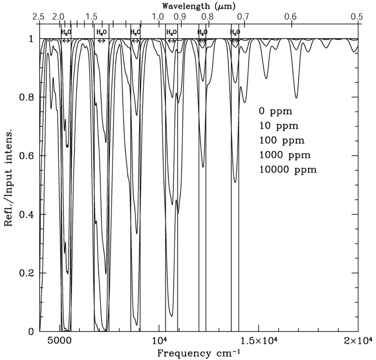
Figure 7. The reflection spectrum of water is shown for five humidity levels, similar to the previous figure. Dominant features are at 0.7, 0.8, and 0.9 microns in the visible, and 1.1, 1.4, and 1.9 microns in the near infrared.
