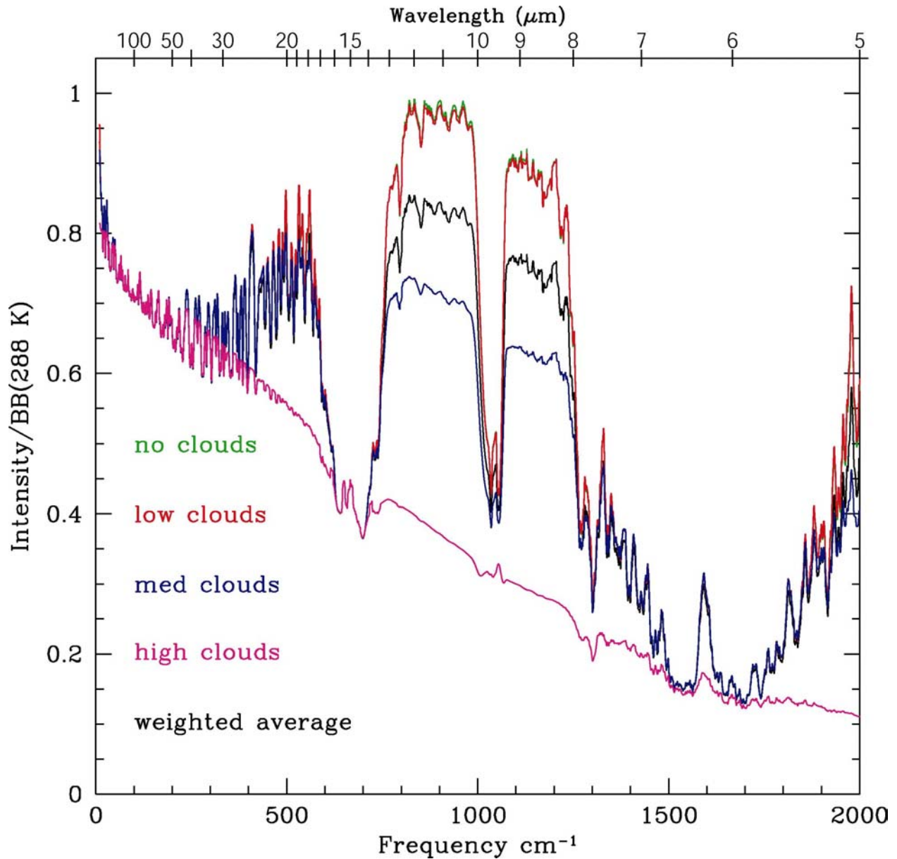
Figure 4. Normalized infrared thermal emission spectral models of the Earth are shown for five cloud conditions. Each spectrum is calculated as discussed in the text, for the present Earth's altitude-dependent, mid-latitude temperature structure and gas species mixing ratio profiles, and at a zenith angle of 60 degrees to closely simulate a whole Earth integration. Frequency (in wavenumbers, \text{cm}^{-1} ) is indicated at the bottom, and wavelength (in microns, 10^{-6} m) as marked at the top.
