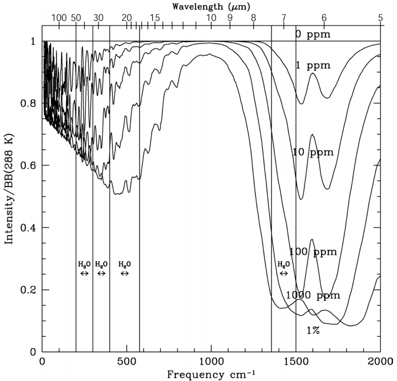
Figure 6. The thermal emission spectrum of water is shown for six humidity levels ranging from completely dry to essentially saturated. In each case the Earth's water vapor vertical mixing ratio profile is used, but scaled to give the surface mixing ratios indicated. Dominant features are the 15-100 micron rotational bands, and the 6 micron vibrational bands. Here and in subsequent figures, potential broad detection wavelength regions are indicated, chosen for their likelihood of producing a relatively clean detection of each species for an extrasolar terrestrial planet.
