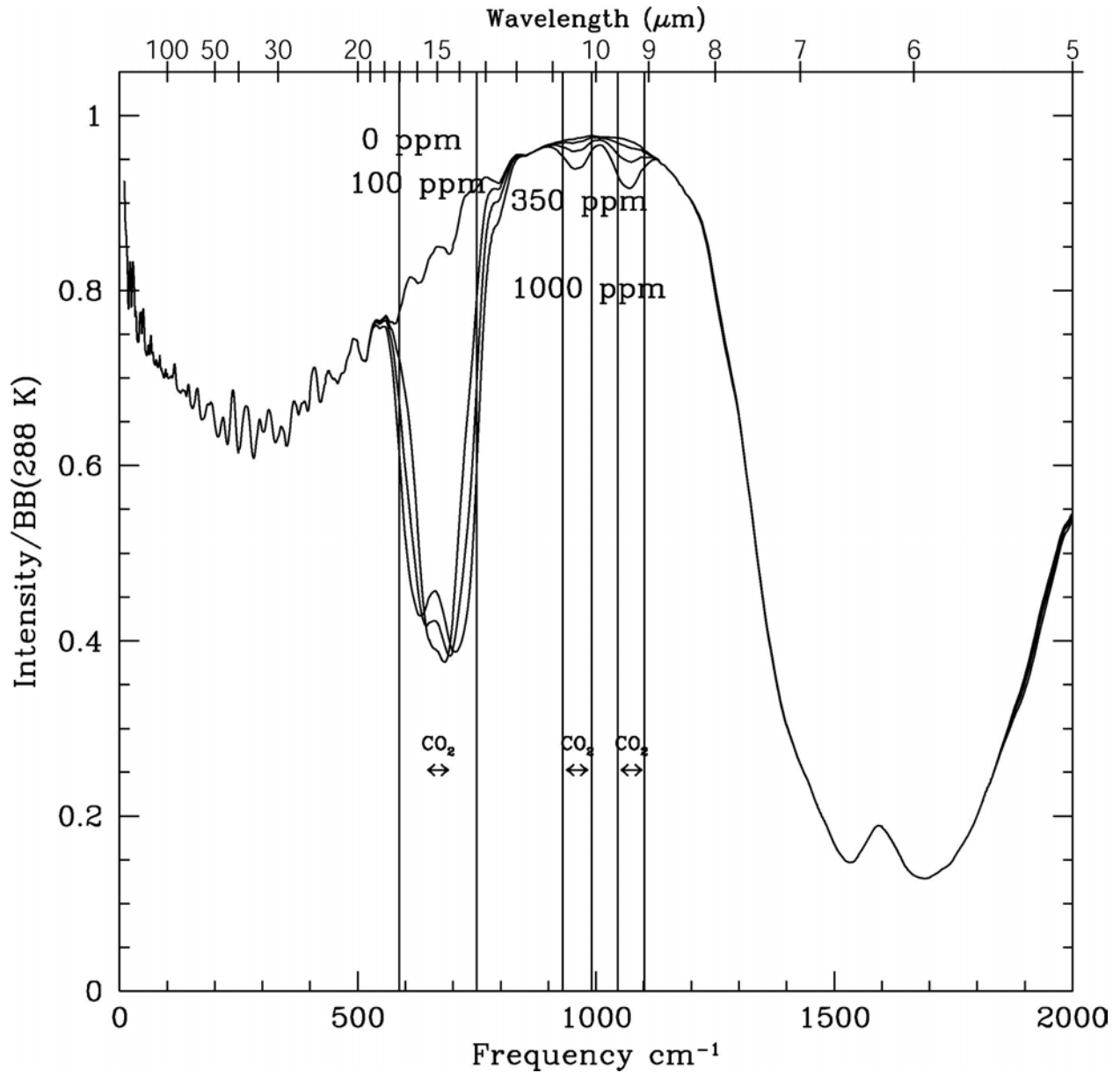
Figure 8. The thermal emission spectrum of carbon dioxide is shown for four abundance levels. A nominal level of water vapor is assumed to be simultaneously present. The 15 micron feature of CO 2 dominates the spectrum, but at high abundances the weak 9 and 10 micron bands also begin to show up. Note the inversion in the core of the 15 micron band at high abundances, due to increased opacity in the warm stratospheric layer.
