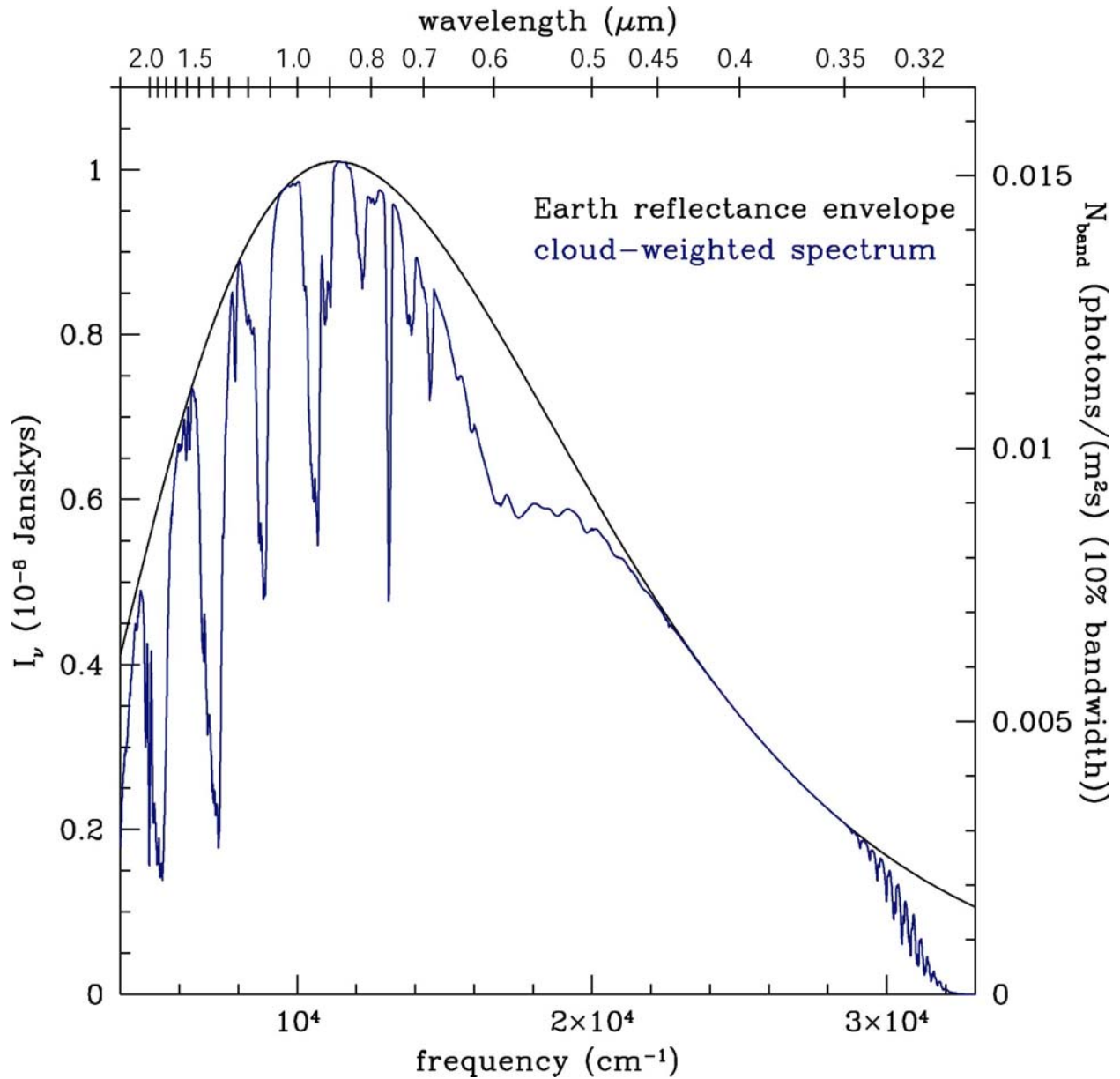
Figure 3. Visible to near-IR portion of the Earth model spectrum, showing a reflection spectrum of the Earth's surface and clouds in the absence of an atmosphere (upper curve), and the net spectrum after the addition of the dominant atmospheric molecular species and a realistic model atmosphere mixed in with a model distribution of opaque clouds distributed over several altitudes (lower curve). Two intensity scales are provided, astrophysical units (left) and photons (right).
