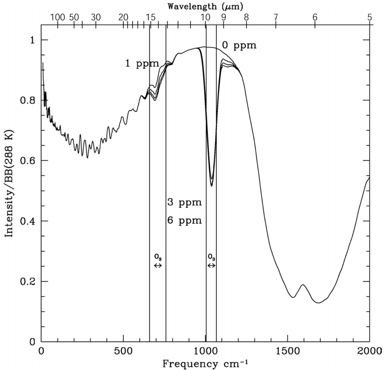
Figure 10. The thermal emission spectrum of ozone is shown for four abundance levels, where the present Earth's mixing ratio profile, dominated by the stratospheric ozone layer, has been scaled, and the value indicated is that at the peak of the ozone layer. The 9 micron feature is saturated for all indicated abundances, and only the 14 micron feature, which would be hidden by any CO 2 present, is on the linear part of the curve of growth.
