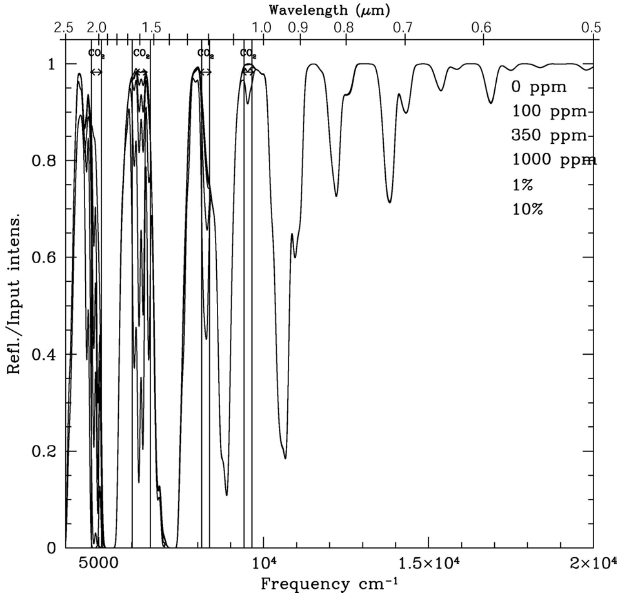
Figure 9. The reflection spectrum of carbon dioxide is shown for six abundances. As in the preceding and following figures, a background abundance of water vapor is also included. At high abundances, CO 2 could be detected in the 1.06 and 1.3 micron bands, but to see lower abundances the 1.6 and 2.0 micron bands would be needed.
