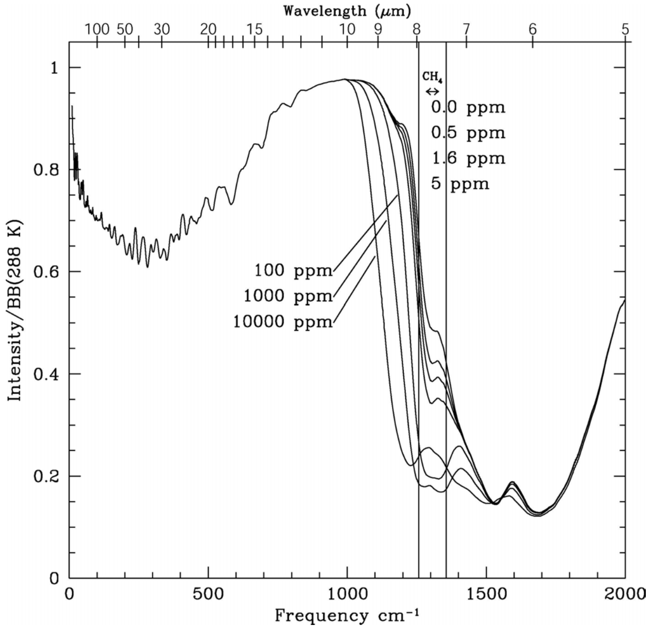
Figure 13. The thermal emission spectrum of methane is shown for seven mixing ratios. The 7 micron band would show up more distinctly if it were not for the presence of water in the background, which in this case is a serious potential spectral contaminant. Present terrestrial methane levels will only produce a weak feature on the side of the dominant water band, but high methane levels, such as may have been present in the early Earth's atmosphere, could produce a stronger, more easily detectable feature.
