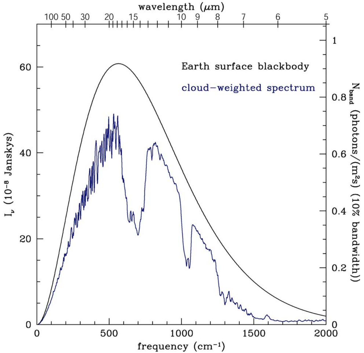
Figure 2. IR portion of the Earth model spectrum, showing the blackbody spectrum of the Earth's surface in the absence of an atmosphere (upper curve), and the net spectrum after the addition of the dominant atmospheric molecular species and a realistic model atmosphere mixed in with a model distribution of opaque clouds distributed over several altitudes (lower curve). Two intensity scales are provided, astrophysical units (left) and photons (right).
