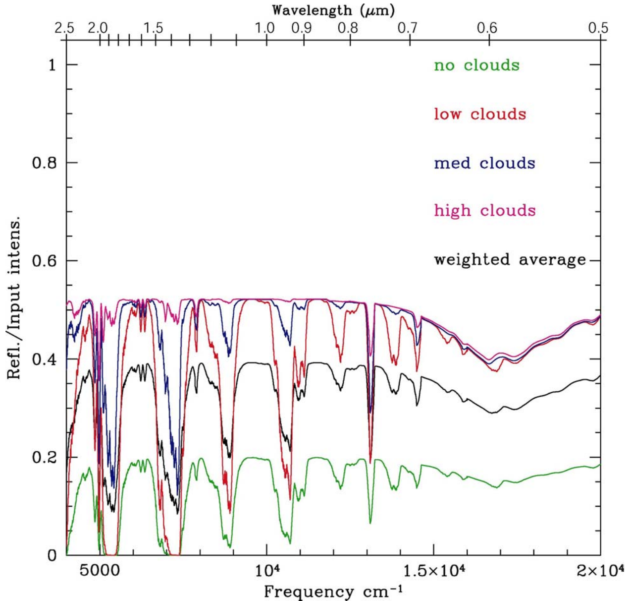
Figure 5. Normalized visible reflection spectral models of the Earth, for the same model atmosphere and cloud conditions as shown in Figure 4. The clear atmosphere case in the lower curve has the smallest continuum level owing to the fact that the surface reflectivity is low compared to clouds, and conversely the overcast cloud cases have high continuum fluxes. The weighted average is a linear combination of the extreme cases, and was calculated for an overall albedo of about 39%, which is higher than the most recently available value of about 29.7% (Goode et al., 2001). The weighted average spectra have cloud altitudes and covering fraction as follows: low cloud, 1 km, 20%; medium cloud, 6 km, 30%; and high cloud, 12 km, 10%. In the reflected spectrum, the main effect of adding clouds is to increase the reflected continuum flux and reduce the relative depths of absorption features.
