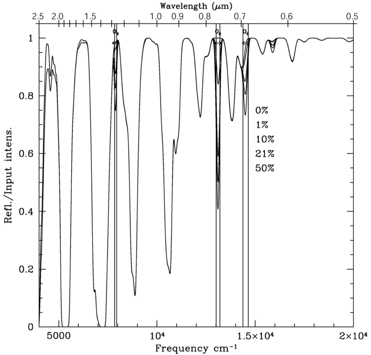
Figure 16. The visible reflection spectrum of molecular oxygen is shown for five abundance levels. Candidate detection bands are the 0.7 and 0.76 micron bands, which are spectrally relatively narrow, but which are roughly linear in their response to oxygen abundance. At 0.76 micron there is no known interfering feature. (There is no corresponding feature for oxygen in the mid-IR wavelength range)
