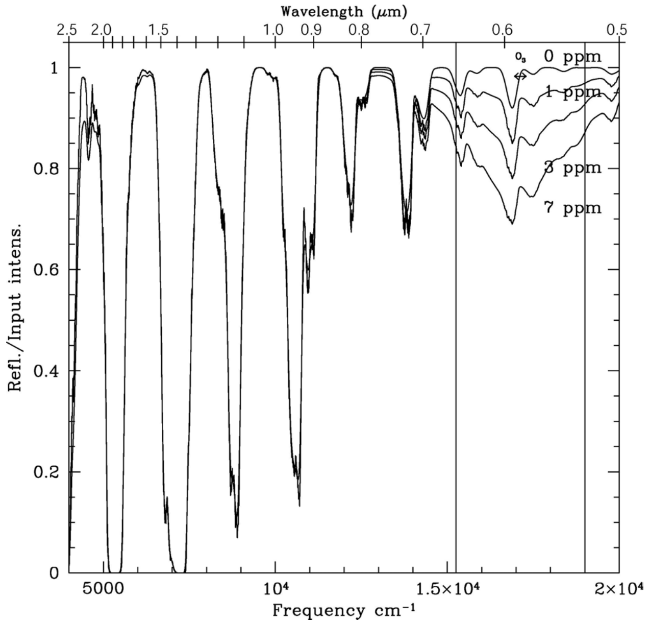
Figure 11. The visible reflection spectrum of ozone is shown for four abundance levels, for conditions as given in the previous figure caption. The broad 0.6 micron band intensity responds linearly to variations in mixing ratio.
