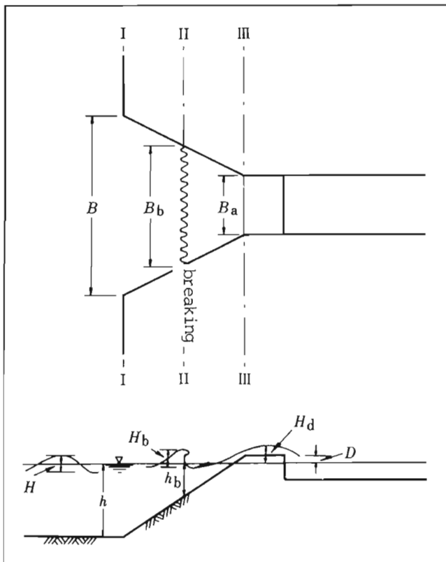
Figure 6 Wave energy concentration and breaking of wave.
