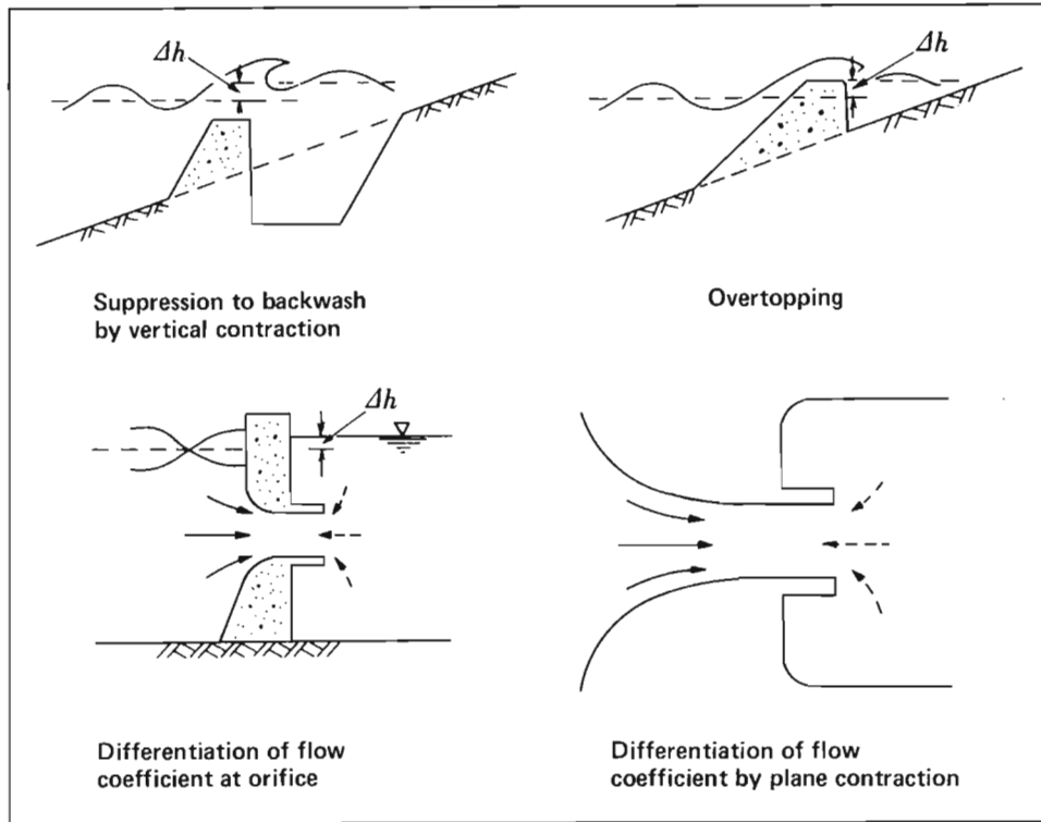
Figure 5 Mean water level raised by wave energy.
