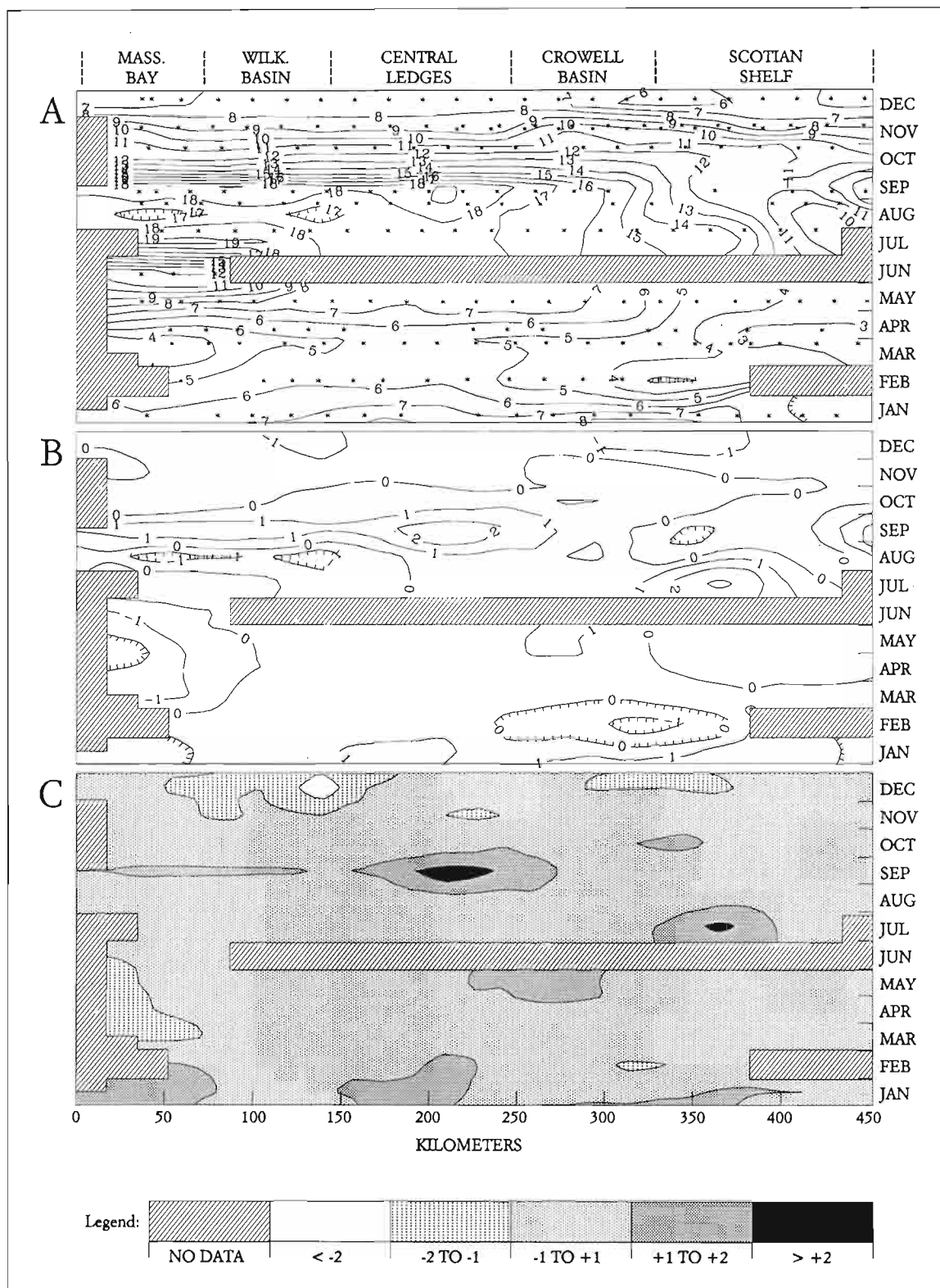
Figure 64 Surface temperature conditions along the Gulf of Maine route during 1980. (A) Measured values (degrees Celsius). Dots indicate sampling locations. (B) Anomalies based on 1978 through 1990 means. (C) Standardized anomalies (standard deviations) based on 1978 through 1990 means and variances. In panels A and B, values decline on those sides of contour lines with hachures.
