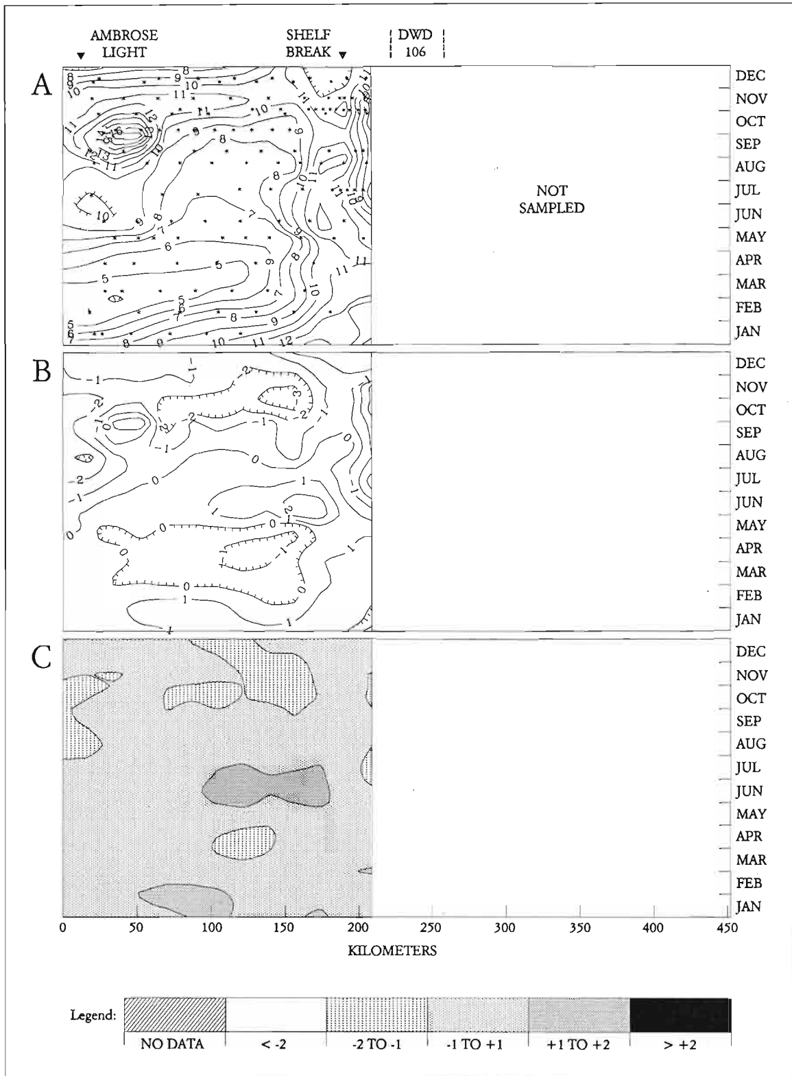
Figure 44 Bottom temperature conditions along the Middle Atlantic Bight route during 1987. (A) Measured values (degrees Celsius). Dots indicate sampling locations. (B) Anomalies based on 1978 through 1990 means. (C) Standardized anomalies (standard deviations) based on 1978 through 1990 means and variances. In panels A and B, values decline on those sides of contour lines with hachures.
