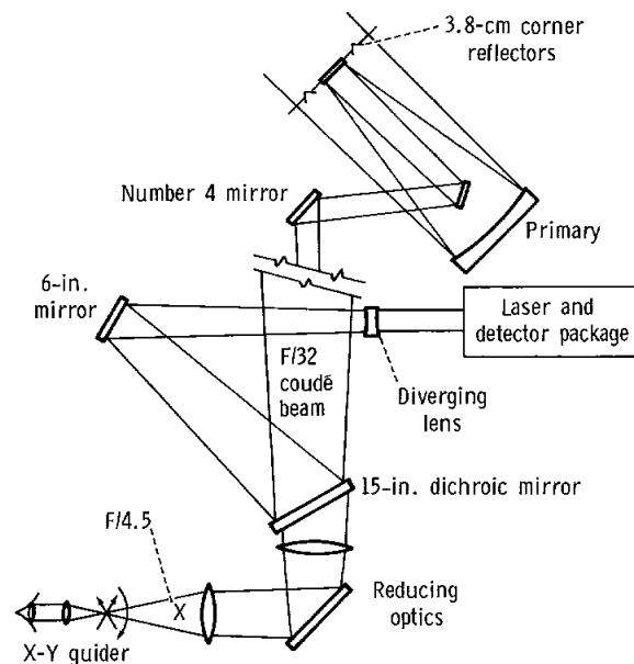
FIGURE 11-7.—Telescope matching optics and guider.
