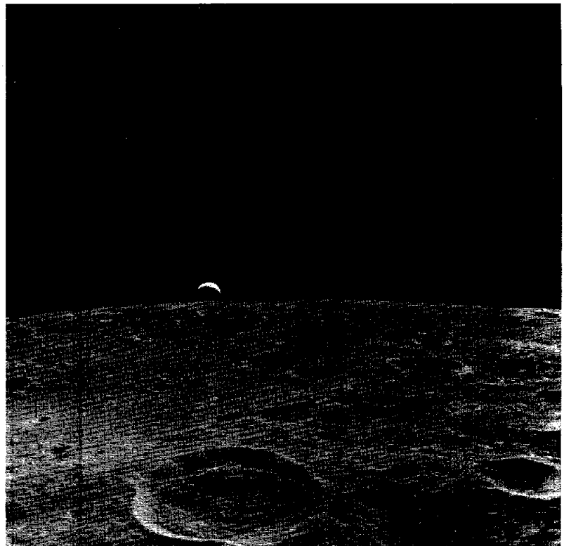
FIGURE 1-4.—Earthrise photographed as the LM reacquired communications with Earth one revolution before landing at Fra Mauro. Pasteur Crater, in the foreground, is centered near latitude 12^{\circ} S, longitude 105^{\circ} E in rugged terrain just beyond the eastern limb of the Moon as viewed from Earth (AS14-66-9228).
