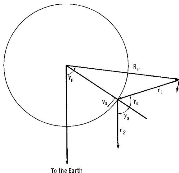
FIGURE 17-1.—Experiment geometry and parameter definition.
