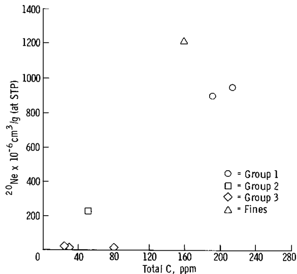
FIGURE 5-12.—The solar-wind-derived ^{20}\text{Ne} as a function of C content. Samples are classified according to group; it should be noted that C appears to follow Ne and that some correlation with rock type exists.
