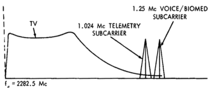
Lunar Module FM Downlink Spectrum
