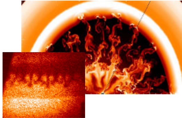
A simulation of a Type II Supernova shock wave, exhibiting complex compressible hydrodynamic flow compared with a radiograph showing the results of an experiment using the Omega laser to create a shock wave which exhibits similar behavior on a much smaller scale.
