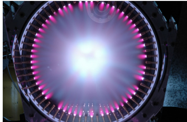
Convergence of high velocity plasma jets creates high energy density plasmas.
