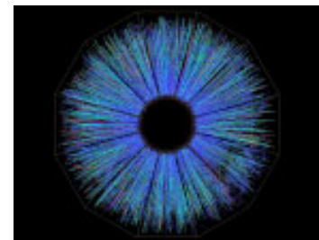
End view of a collision of two 30-billion electron-volt gold beams in the STAR detector at the Relativistic Heavy Ion Collider at BNL. The beams travel in opposite directions at nearly the speed of light before colliding.
