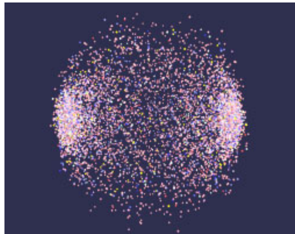
The aftermath of a head-on collision of two gold nuclei at RHIC in which over 6,000 particles (shown as dots) are produced.
