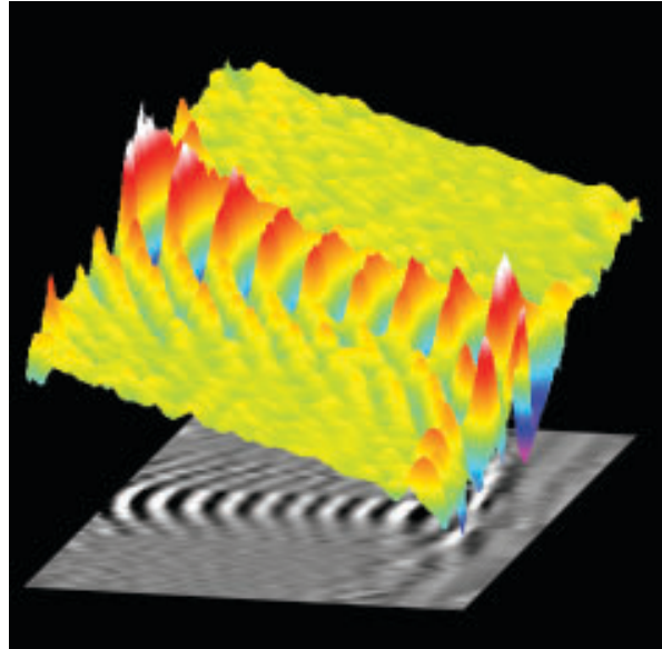
Images of a wake field produced by a 30 TW laser pulse in plasma of density 2.7 \times 10^{18} \text{ cm}^{-3} . These waves show curved wavefronts, an important feature for generating and accelerating electrons that had been predicted, but never before seen.
