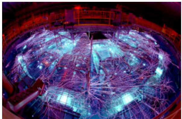
Time-exposure photograph of electrical flashover arcs produced over the surface of the water in the accelerator tank as a byproduct of the operation of the Z pulsed power facility at SNL. These flashovers are much like strokes of lightning.
