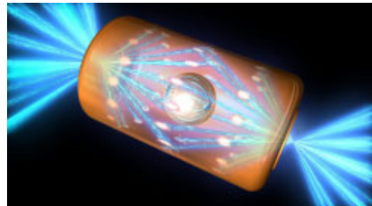
An artist's rendering of a gold cylinder or "hohlraum" approximately 1 cm in length being illuminated in the indirect drive configuration by the NIF laser. The laser beams deposit their energy on the inside surface of the hohlraum, where the energy is converted to thermal x-rays which heat and ablate the surface of the ignition capsule, causing it to implode.
