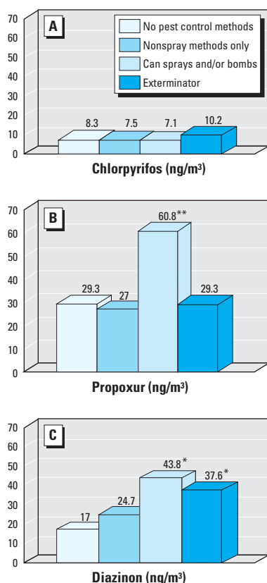
Figure 1. Geometric mean levels of (A) chlorpyrifos, (B) propoxur, and (C) diazinon in personal air samples (ng/m 3 ) stratified by whether or not pest control methods were used during pregnancy. Pesticide levels were log-transformed prior to statistical analyses.
