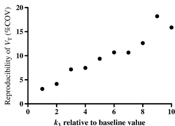
Fig. 4. Reproducibility of distribution volume estimation as a function of receptor density, as simulated by increasing the value of k_3 . Simulations were performed by using average rate constants obtained in thalamus ( K_1 = 0.12 mL \bullet cm ^{-3} min ^{-1} , k_2 = 0.11 min ^{-1} , k_3 = 0.069 min ^{-1} , and k_4 = 0.023 min ^{-1} ) and average input function, and by increasing k_3 up to 10 times of its baseline value. The increases caused poorer reproducibility (i.e., larger % COV), but the % COV was still less than 10% for a fivefold increase in k_3 .
