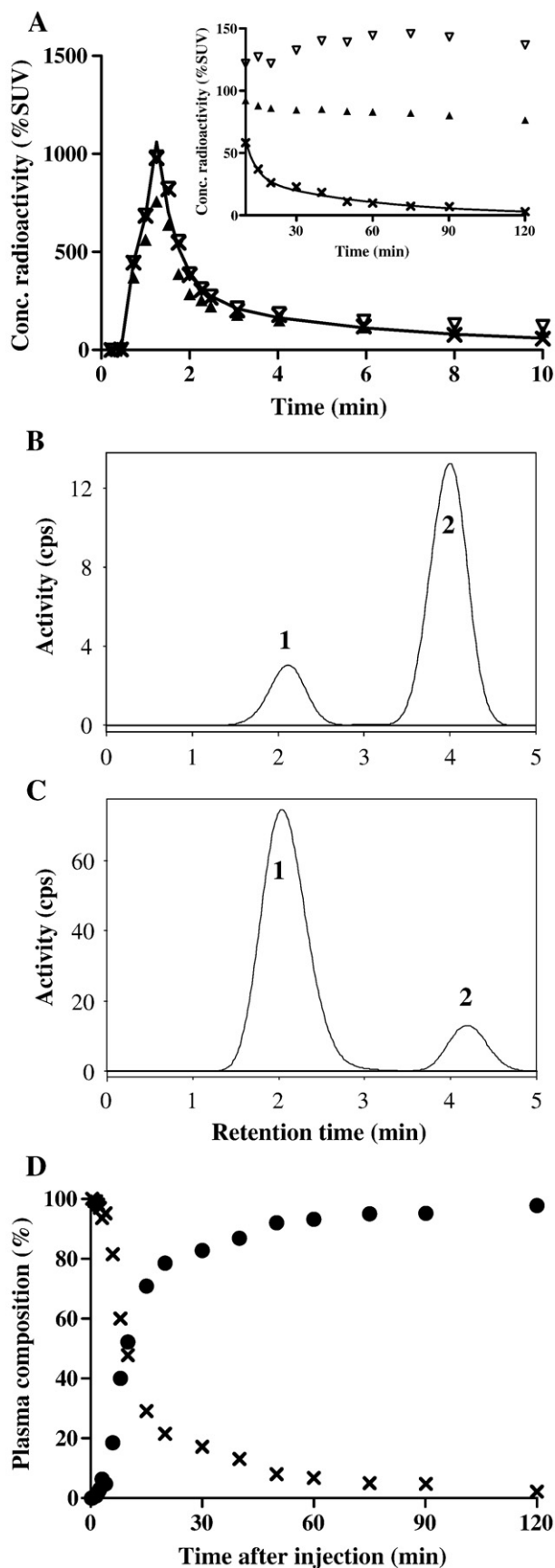
Fig. 2. Concentration of radioactivity in plasma of the typical healthy subject shown in Figs. 1A and B. (A) Concentrations are plotted for unchanged parent radioligand [ 11 C]PBR28 (×), total radioactivity in blood (▲), and total radioactivity in plasma (▽). The time course of [ 11 C]PBR28 was fitted to a tri-exponential curve (—). Radiochromatograms of activity extracted from plasma at 6 (B) and 40 (C) min after injection of [ 11 C]PBR28. Peak 2 was confirmed to be [ 11 C]PBR28 based on HPLC coelution with nonradioactive PBR28. Peak 1 was a radiometabolite with lipophilicity lower than that of [ 11 C]PBR28. (D) The percentage composition of plasma radioactivity over time is shown for [ 11 C]PBR28 (×) and the radiometabolite (●).
