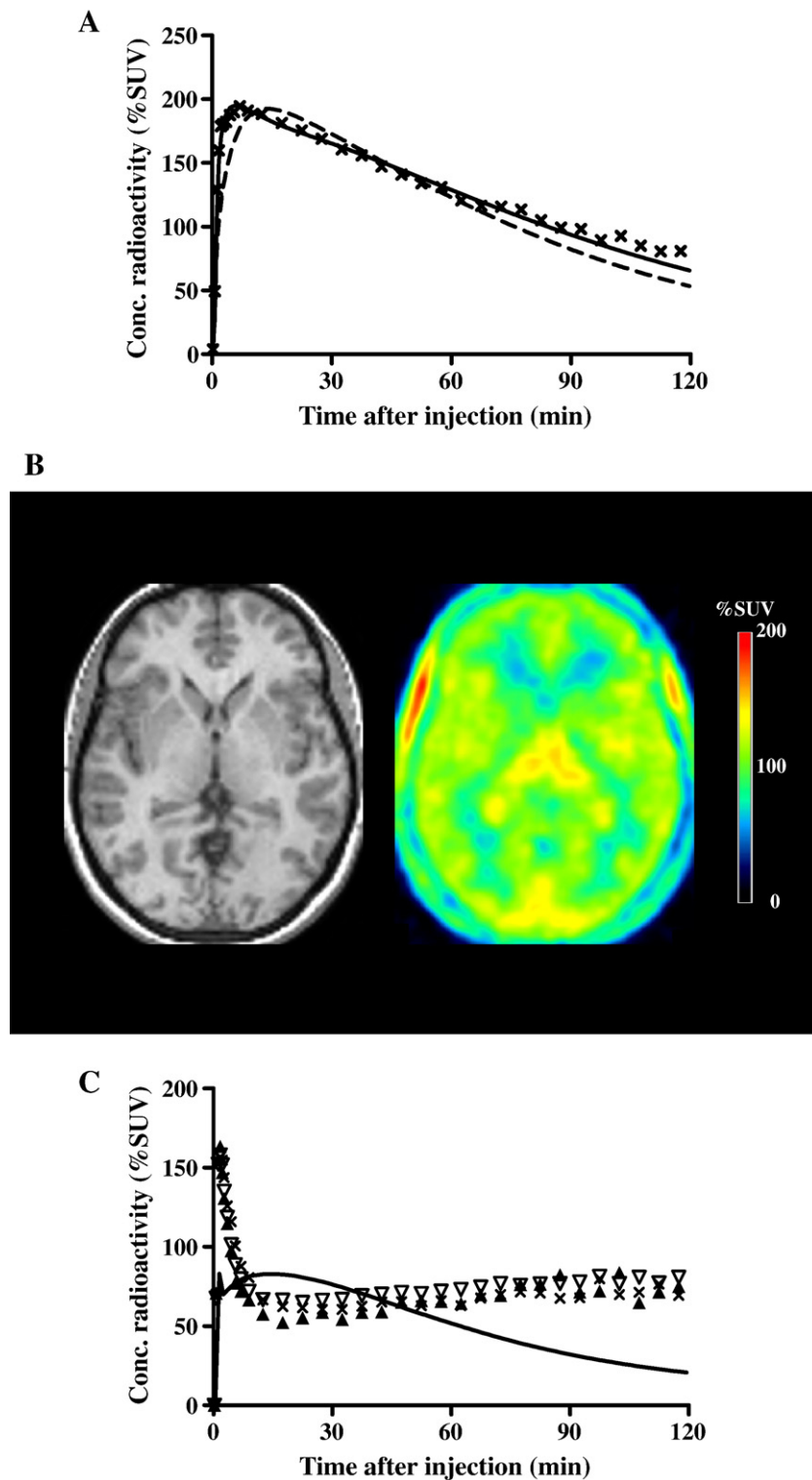
Fig. 1. Time course of radioactivity and images of its distribution in brain after injection of [^{11}\text{C}]\text{PBR28} . (A) Concentrations ( \times ) of radioactivity in thalamus of a typical healthy subject—namely, one who showed binding of the radioligand. The measured data were fitted with one- and two-tissue compartment models with no constraint. The two-tissue compartment model (—) more closely followed the measured values than did the one-compartment model (---). The constrained two-tissue compartment model with a fixed value of K_1/k_2 (not plotted) was visually indistinguishable from the unconstrained two-compartment model. (B) The transverse PET image (right) of this typical healthy subject was created by averaging all frames and scaled using % SUV. The coregistered MRI (left) of this subject identifies that the PET image was obtained at the level of the thalamus. (C) Concentrations of radioactivity in thalamus ( \times ), caudate ( \blacktriangle ), and parietal cortex ( \nabla ) in an atypical human subjects—i.e., one who appeared to have no binding of the radioligand. The one-compartment fitting (solid line) converged but with large deviations from the observed data, and two-compartmental fitting (not plotted) did not converge.
