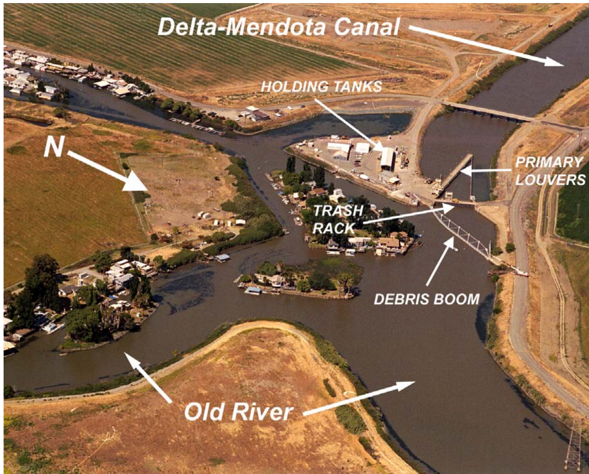
FIGURE 1.—Tracy Fish Collection Facility, Old River Branch of the San Joaquin River, California.
