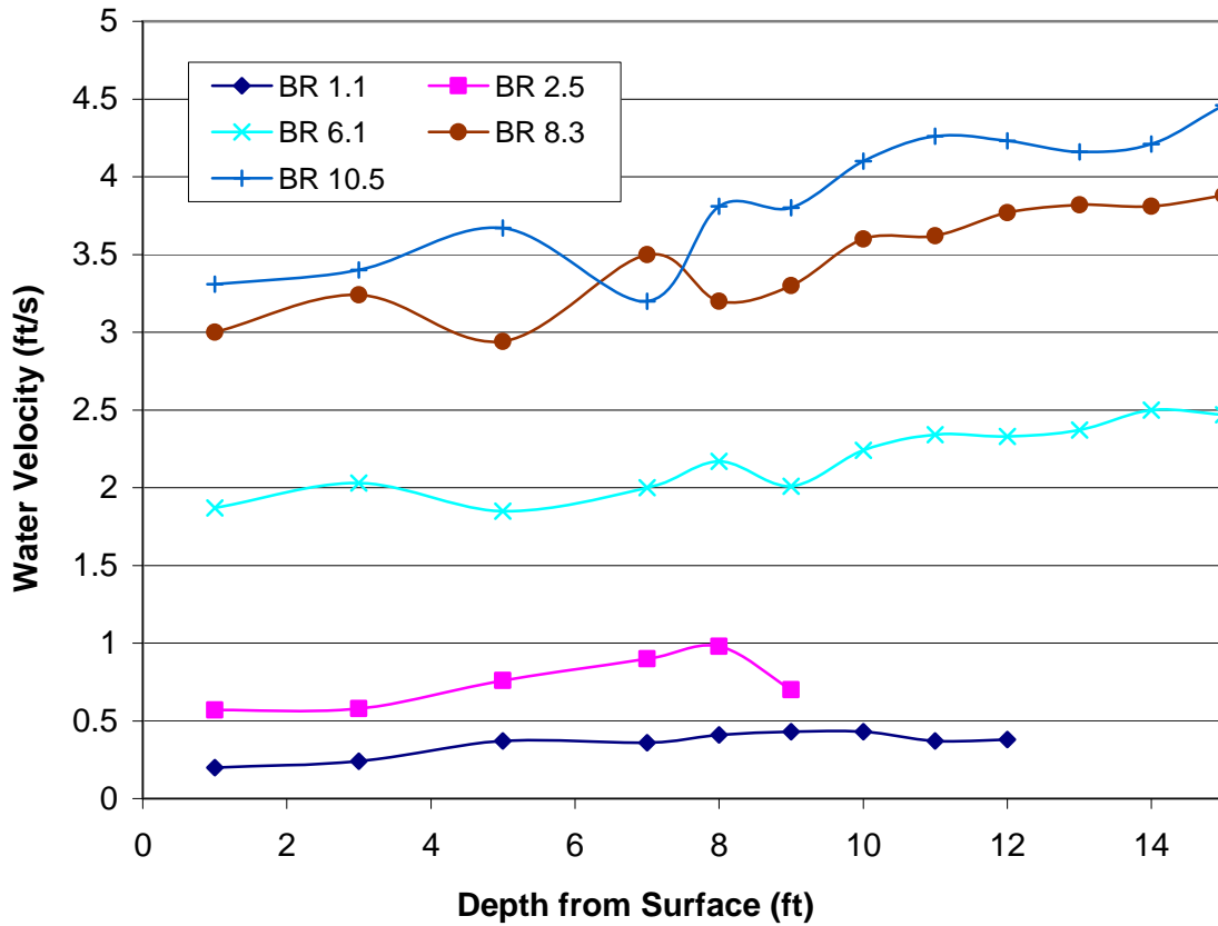
FIGURE 8.—Vertical velocity profiles in the mouth of bypass No. 4 at five bypass ratios (BR): 1.1, 2.5, 6.1, 8.3, and 10.5. Flows through the bypass were 4.1, 10.9, 21.9, 34.6, and 38.8 ft 3 /s (0.1, 0.3, 0.6, 1.0, and 1.1 m 3 /s), respectively.
